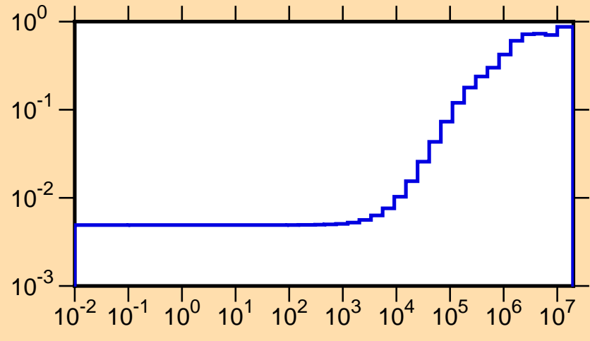
\mu vs. E for ^{138}\text{Sm}(\text{mt251})
