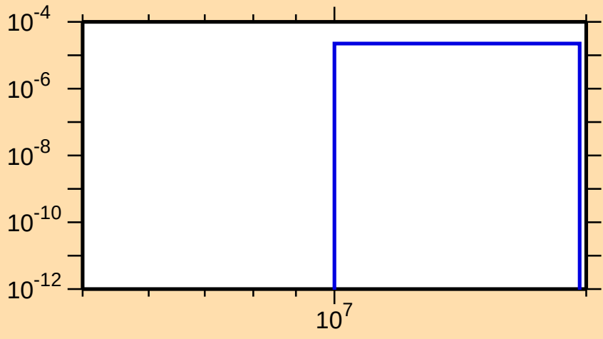
\sigma vs. E for ^{138}\text{Sm}(n,t)
