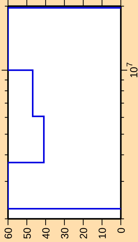
\Delta\sigma/\sigma vs. E for ^{138}\text{Sm}(n,\text{ncont.})
