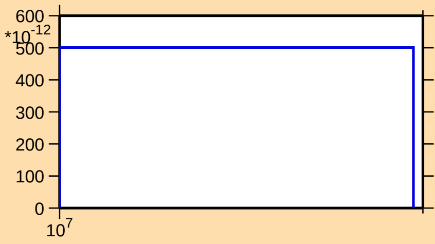
\sigma vs. E for ^{138}\text{Sm}(n,\text{nd})
