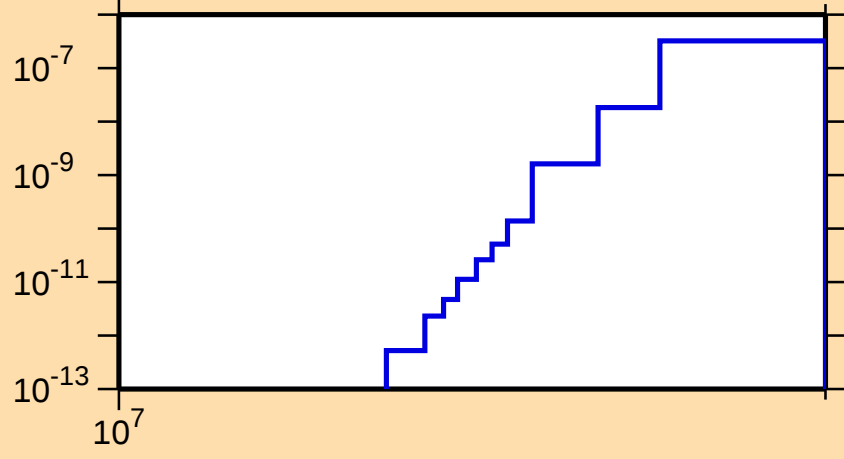
\sigma vs. E for ^{139}\text{Sm}(\text{mt } 45)
