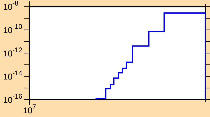
\sigma vs. E for ^{139}\text{Sm}(\text{mt } 34)
