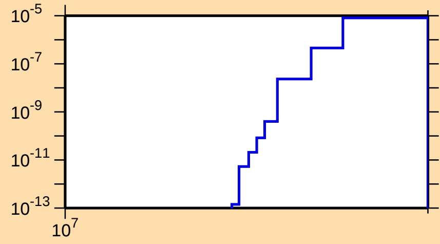
\sigma vs. E for ^{139}\text{Sm}(n,\text{nd})
