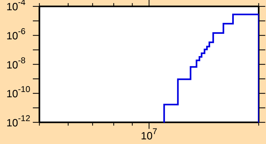
\sigma vs. E for ^{139}\text{Sm}(n,\text{pd})
