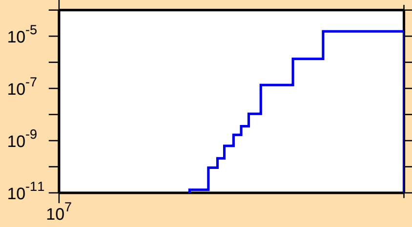
\sigma vs. E for ^{139}\text{Sm}(n,2n\alpha)
