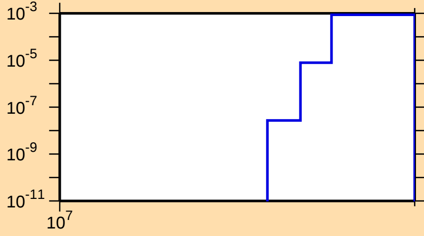
\sigma vs. E for ^{139}\text{Sm}(n,2np)
