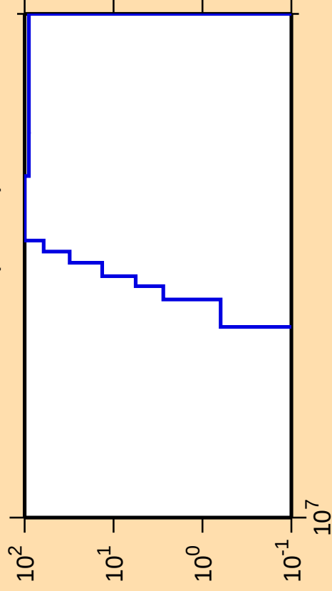
\Delta\sigma/\sigma vs. E for ^{139}\text{Sm}(\text{mt } 45)
