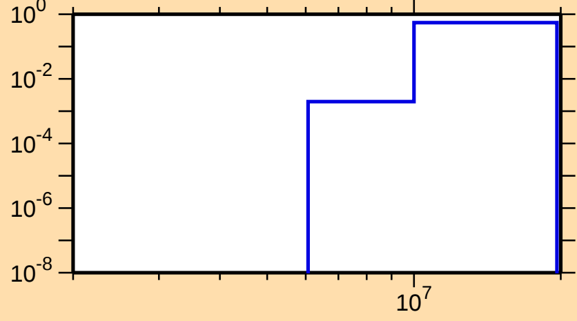
\sigma vs. E for ^{139}\text{Sm}(n,np)
