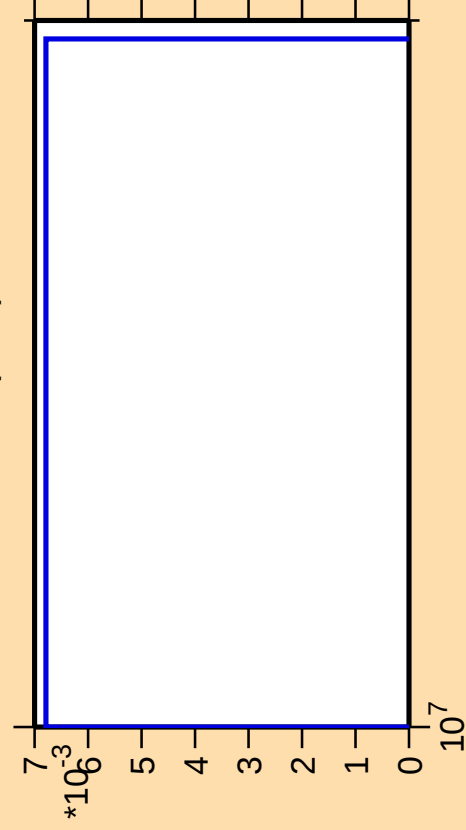
\Delta\sigma/\sigma vs. E for ^{139}\text{Sm}(n,\text{nt})
