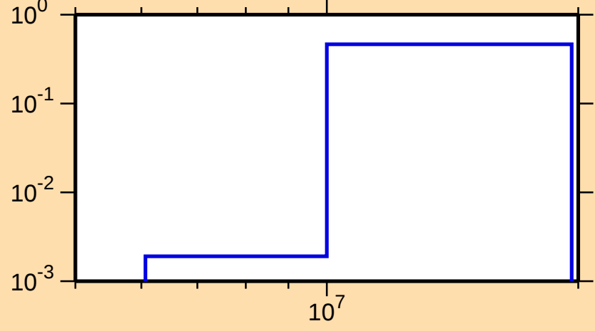
\sigma vs. E for ^{139}\text{Sm}(n,2n)
