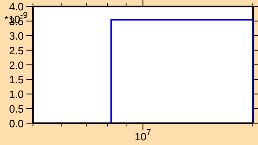
\sigma vs. E for ^{139}\text{Sm}(\text{mt } 45)
