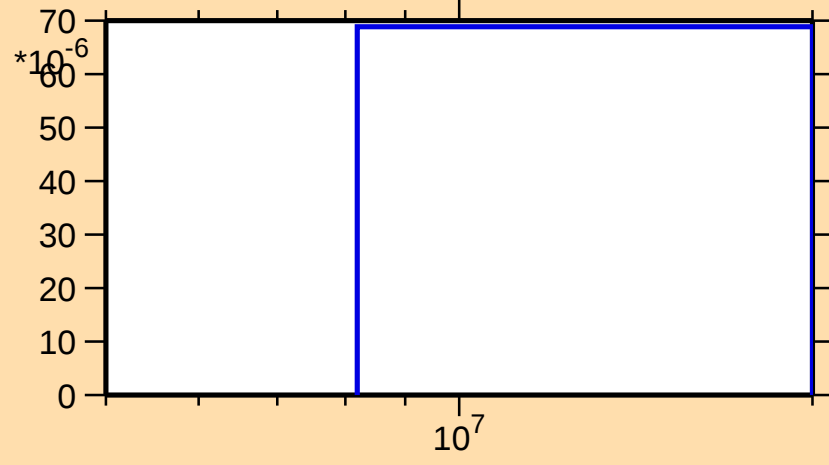
\sigma vs. E for ^{139}\text{Sm}(n,t)
