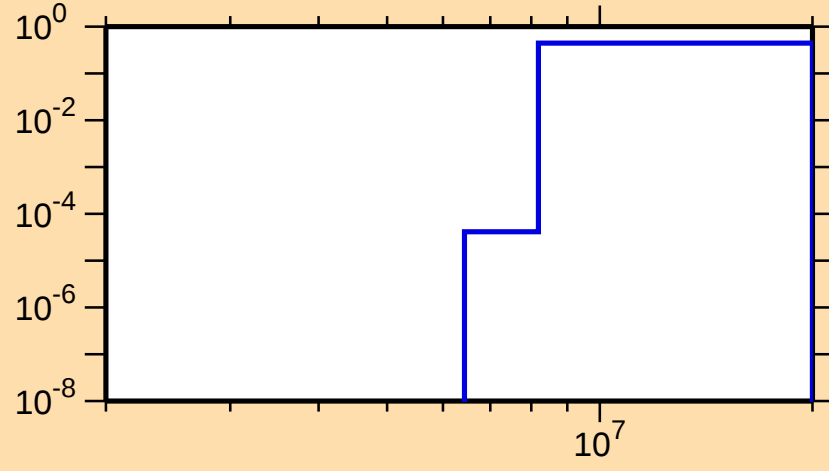
\sigma vs. E for ^{139}\text{Sm}(n,np)
