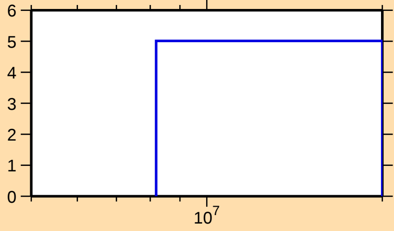
\Delta\sigma/\sigma vs. E for ^{139}\text{Sm}(n,\text{tot.})
