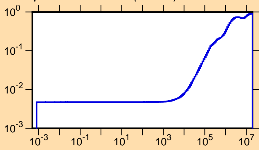
\mu vs. E for ^{143}\text{Sm}(\text{mt251})
