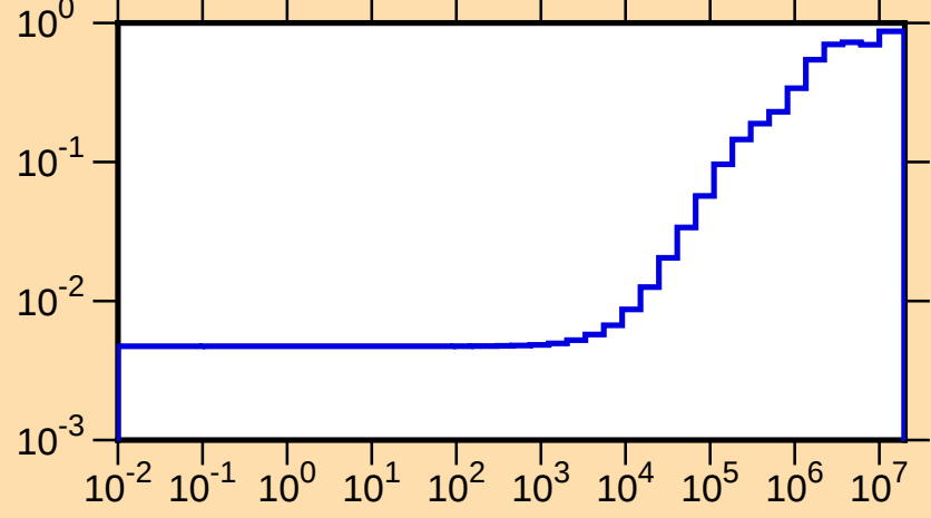
\mu vs. E for ^{143}\text{Sm}(\text{mt251})
