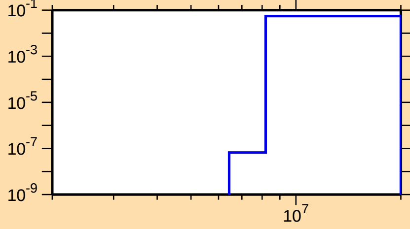
\sigma vs. E for ^{143}\text{Sm}(n,np)
