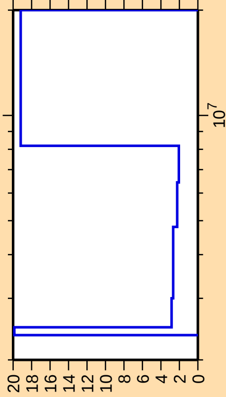
\Delta\sigma/\sigma vs. E for ^{143}\text{Sm}(n,\text{ncont.})
