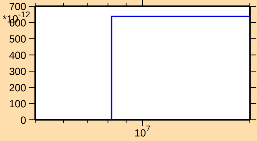
\sigma vs. E for ^{143}\text{Sm}(n,3n)
