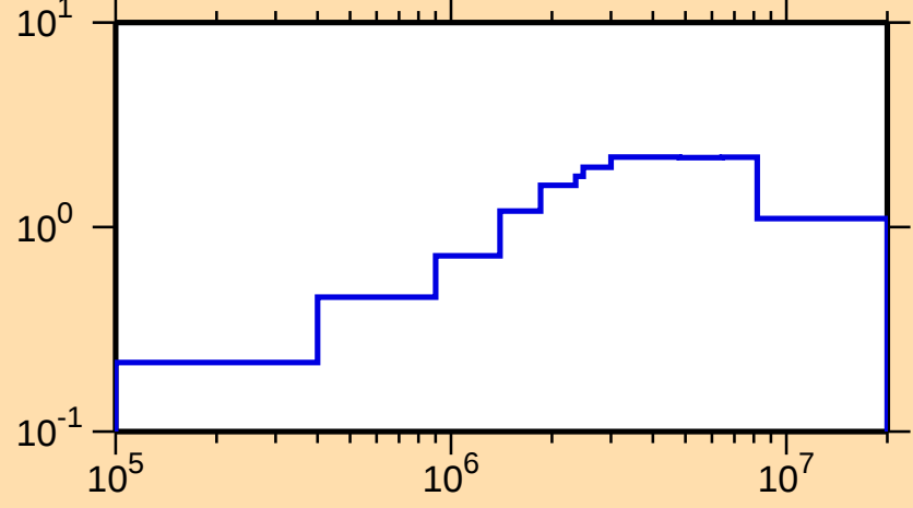
\sigma vs. E for ^{143}\text{Sm}(n,\text{inel.})
