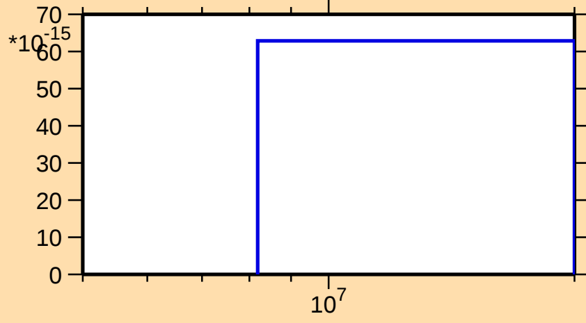
\sigma vs. E for ^{143}\text{Sm}(\text{mt } 45)
