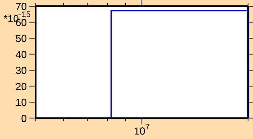
\sigma vs. E for ^{143}\text{Sm}(\text{mt } 34)
