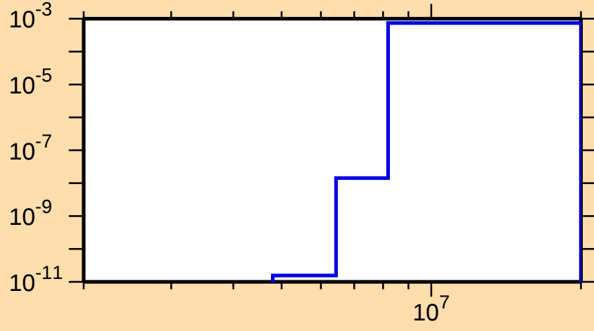
\sigma vs. E for ^{143}\text{Sm}(n,n\alpha)
