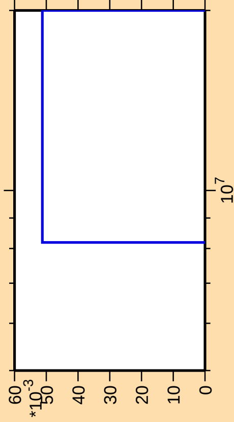
\Delta\sigma/\sigma vs. E for ^{143}\text{Sm}(\text{mt } 45)
