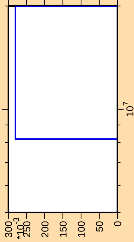
\Delta\sigma/\sigma vs. E for ^{143}\text{Sm}(\text{mt } 34)
