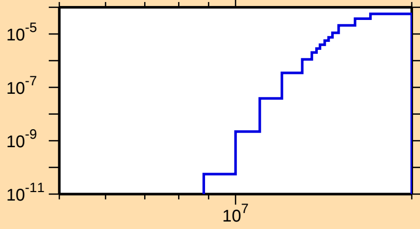
\sigma vs. E for ^{147}\text{Sm}(n,2n\alpha)
