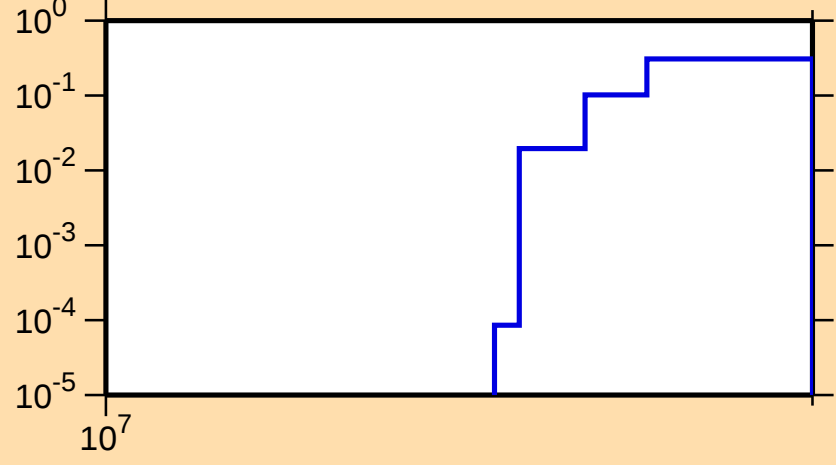
\sigma vs. E for ^{147}\text{Sm}(n,3n)
