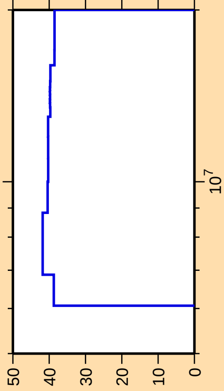
\Delta\sigma/\sigma vs. E for ^{147}\text{Sm}(n,n_1)
