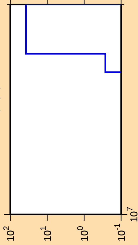
\Delta\sigma/\sigma vs. E for ^{147}\text{Sm}(n,\text{pt})
