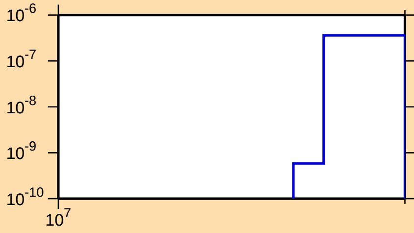
\sigma vs. E for ^{147}\text{Sm}(n,\text{nt})
