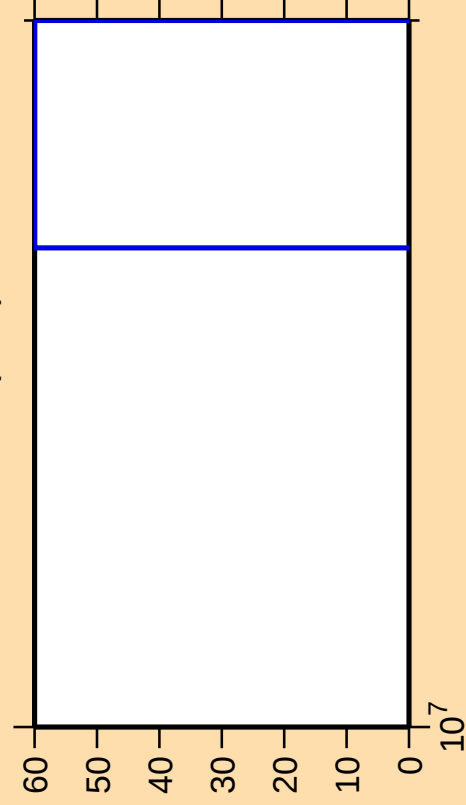
\Delta\sigma/\sigma vs. E for ^{147}\text{Sm}(n,\text{nt})
