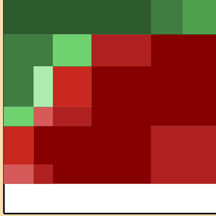
\Delta\sigma/\sigma vs. E for ^{147}\text{Sm}(n,\text{inel.})
