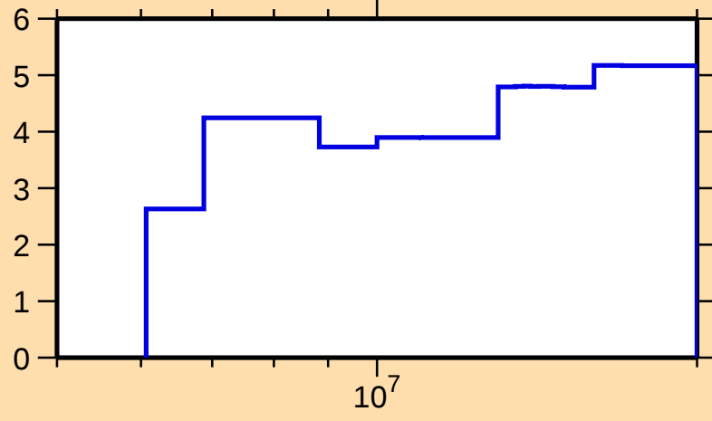
\Delta\sigma/\sigma vs. E for ^{147}\text{Sm}(n,\text{tot.})
