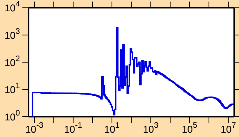
\sigma vs. E for ^{147}\text{Sm}(n,\text{el.})
