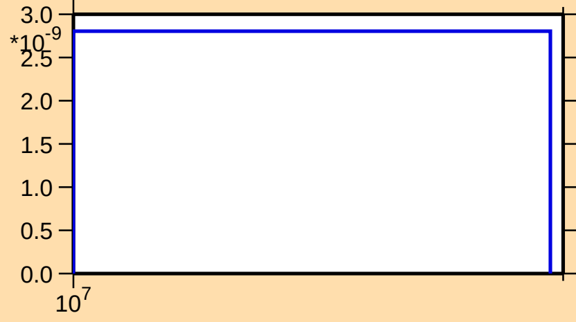
\sigma vs. E for ^{147}\text{Sm}(n,nt)
