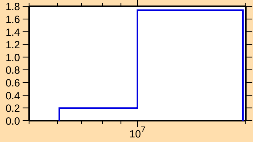
\sigma vs. E for ^{147}\text{Sm}(n,2n)
