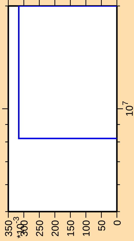
\Delta\sigma/\sigma vs. E for ^{147}\text{Sm}(n,\text{pt})
