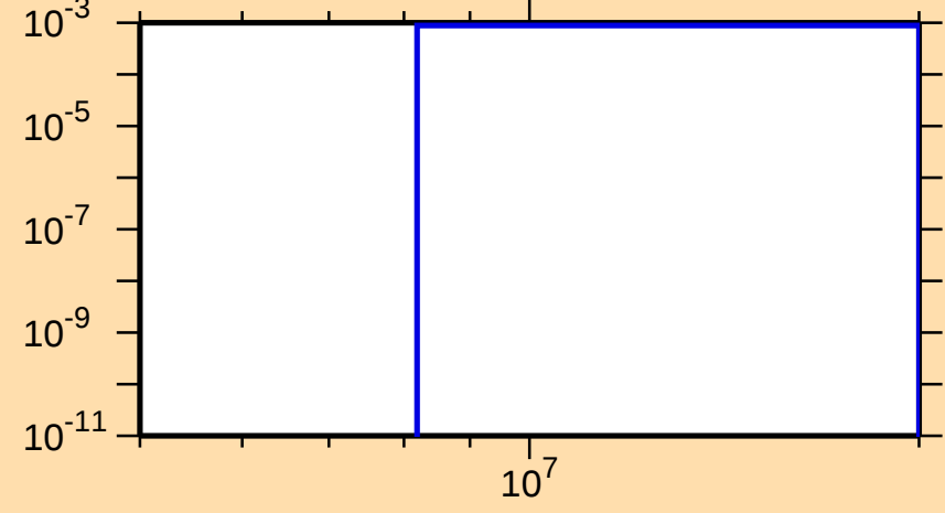
\sigma vs. E for ^{147}\text{Sm}(n,d)
