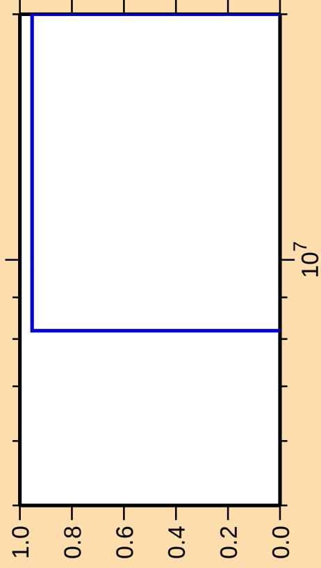
\Delta\sigma/\sigma vs. E for ^{147}\text{Sm}(\text{mt } 45)
