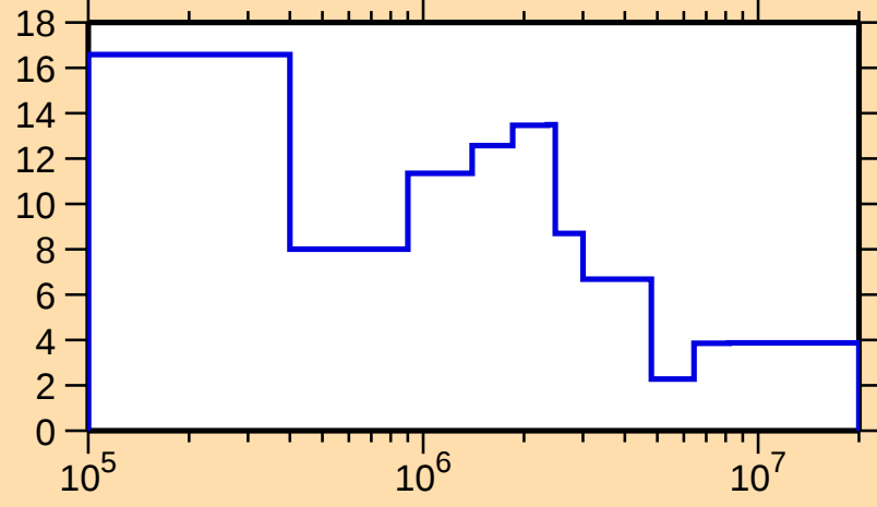
\Delta\sigma/\sigma vs. E for ^{147}\text{Sm}(n,\text{tot.})
