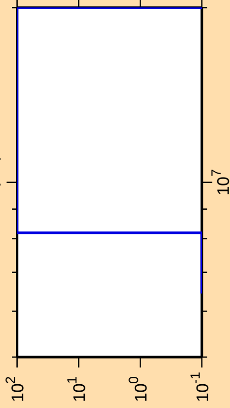
\Delta\sigma/\sigma vs. E for ^{147}\text{Sm}(n,t)
