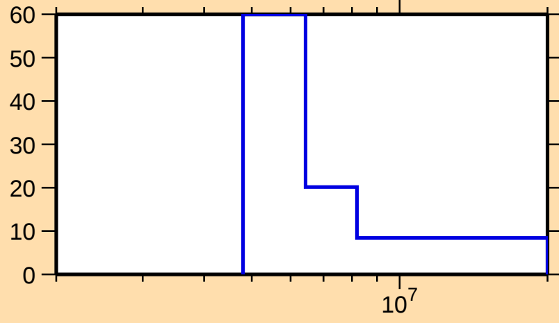
\Delta\sigma/\sigma vs. E for ^{147}\text{Sm}(n,2n)
