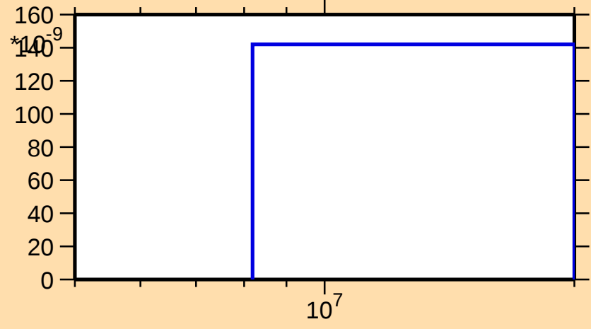
\sigma vs. E for ^{147}\text{Sm}(n,\text{nd})
