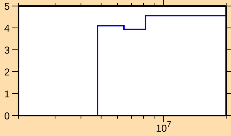
\Delta\sigma/\sigma vs. E for ^{147}\text{Sm}(n,\text{nonel.})
