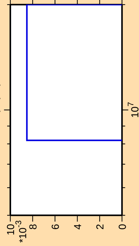
\Delta\sigma/\sigma vs. E for ^{147}\text{Sm}(n,\text{pd})
