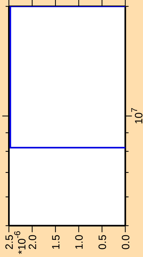
\Delta\sigma/\sigma vs. E for ^{147}\text{Sm}(\text{mt } 11)
