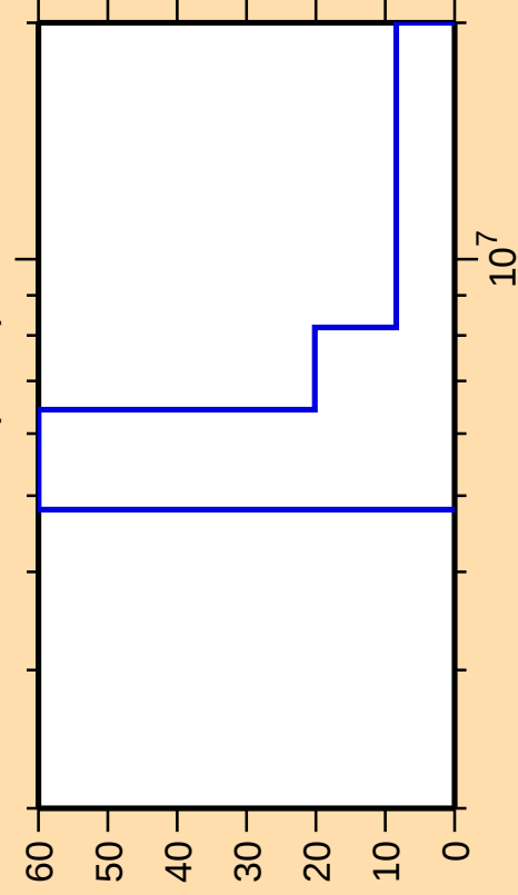
\Delta\sigma/\sigma vs. E for ^{147}\text{Sm}(n,2n)
