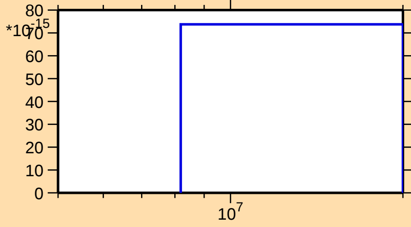
\sigma vs. E for ^{147}\text{Sm}(n,\text{pt})
