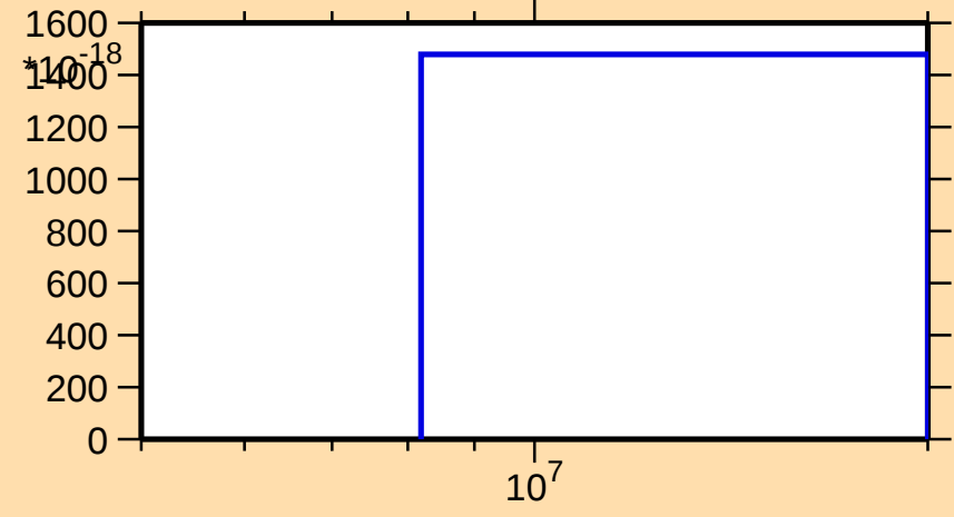
\sigma vs. E for ^{147}\text{Sm}(n,\text{pd})
