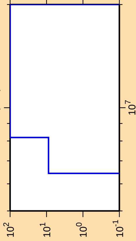
\Delta\sigma/\sigma vs. E for ^{147}\text{Sm}(n,d)
