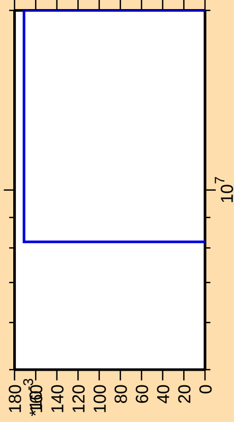
\Delta\sigma/\sigma vs. E for ^{147}\text{Sm}(\text{mt } 34)
