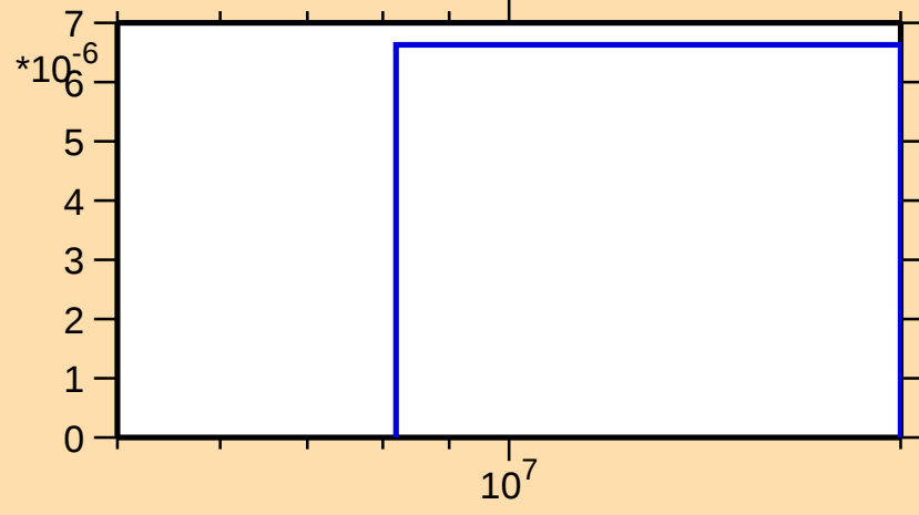
\sigma vs. E for ^{147}\text{Sm}(n,2n\alpha)
