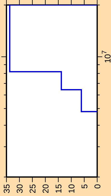
\Delta\sigma/\sigma vs. E for ^{147}\text{Sm}(n,n\text{cont.})
