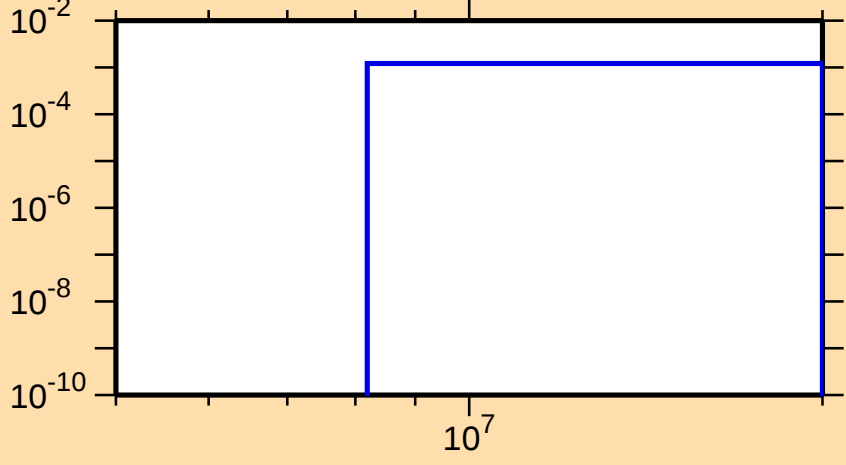
\sigma vs. E for ^{147}\text{Sm}(n,np)
