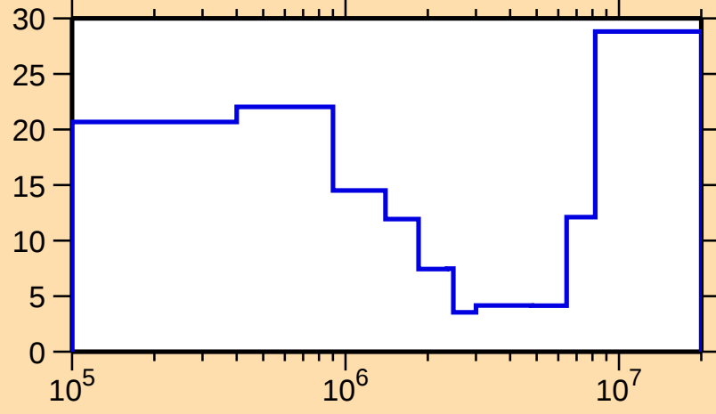
\Delta\sigma/\sigma vs. E for ^{147}\text{Sm}(n,\text{inel.})
