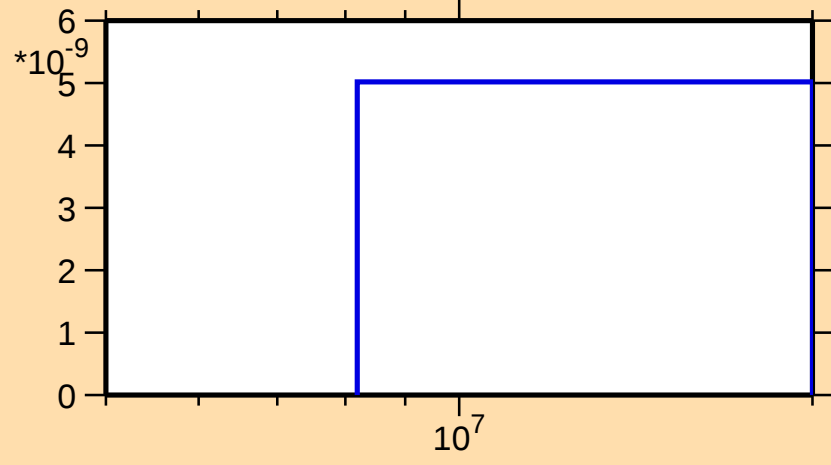
\sigma vs. E for ^{147}\text{Sm}(n,\text{He3})
