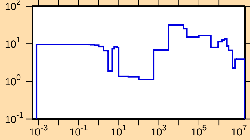
\Delta\sigma/\sigma vs. E for ^{147}\text{Sm}(n,\text{tot.})
