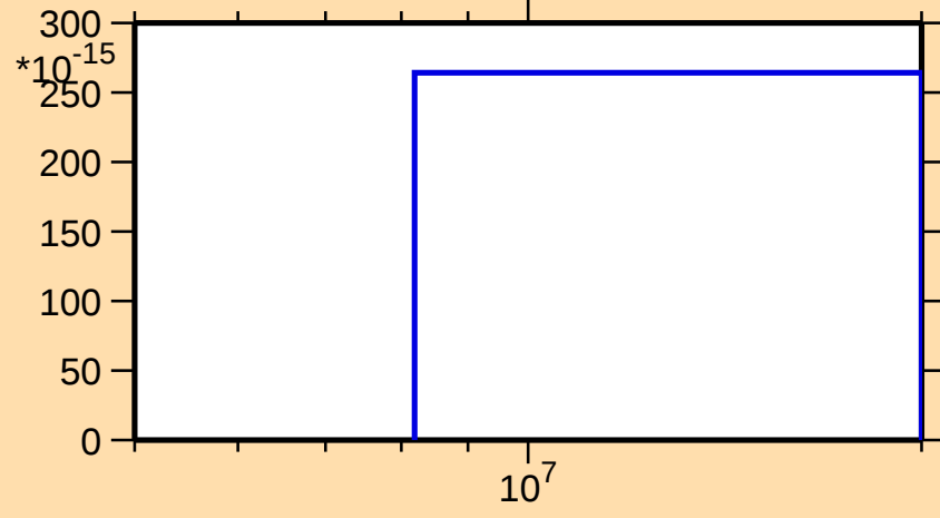
\sigma vs. E for ^{147}\text{Sm}(\text{mt117})
