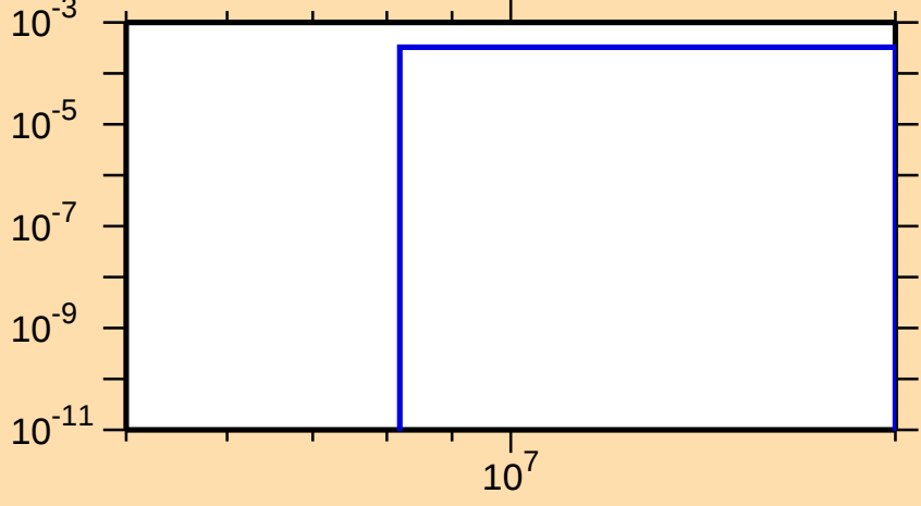
\sigma vs. E for ^{147}\text{Sm}(n,t)
