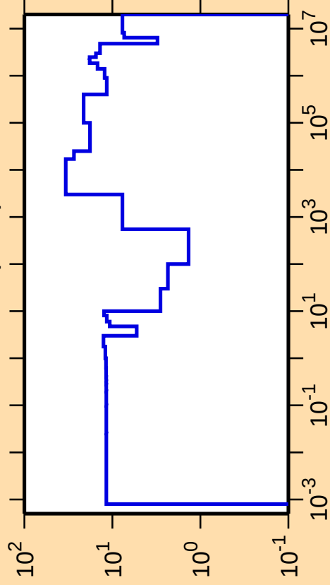
\Delta\sigma/\sigma vs. E for ^{147}\text{Sm}(n,\text{el.})
