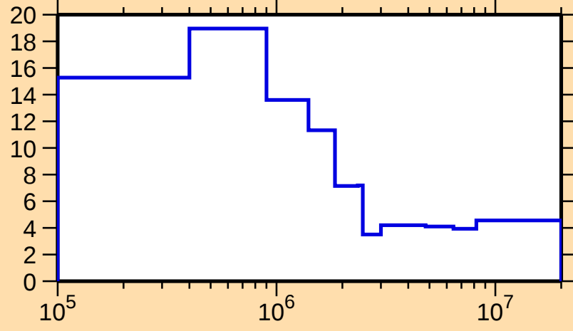
\Delta\sigma/\sigma vs. E for ^{147}\text{Sm}(n,\text{nonel.})
