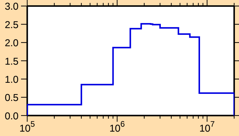
\sigma vs. E for ^{147}\text{Sm}(n,\text{inel.})
