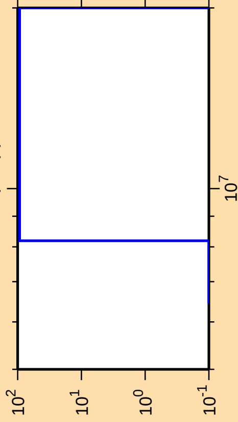
\Delta\sigma/\sigma vs. E for ^{147}\text{Sm}(n,np)
