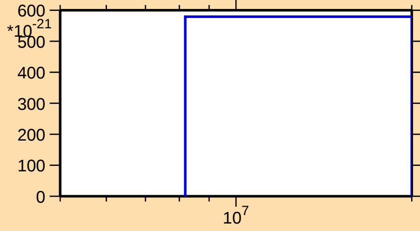
\sigma vs. E for ^{147}\text{Sm}(\text{mt } 11)
