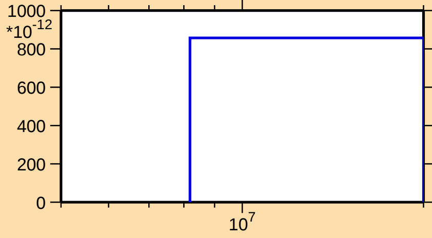
\sigma vs. E for ^{147}\text{Sm}(n,p\alpha)
