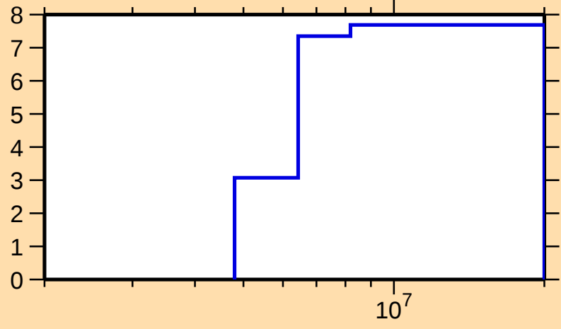
\Delta\sigma/\sigma vs. E for ^{147}\text{Sm}(n,\text{el.})
