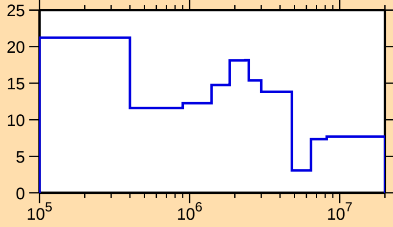
\Delta\sigma/\sigma vs. E for ^{147}\text{Sm}(n,\text{el.})
