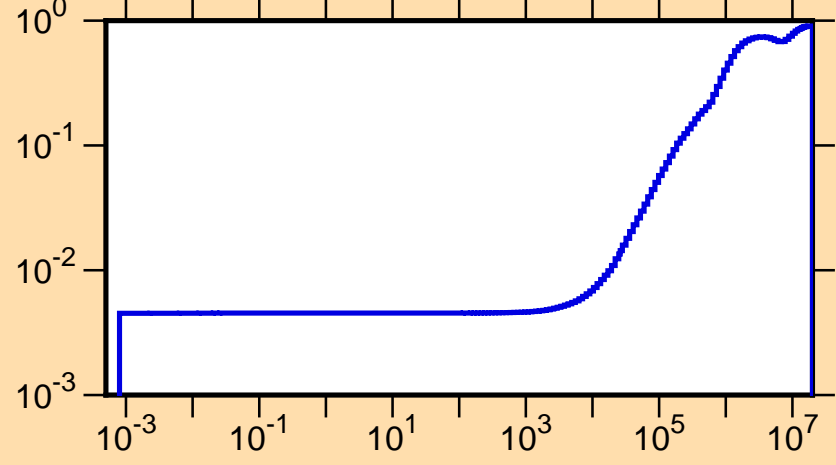
\mu vs. E for ^{149}\text{Sm}(\text{mt251})
