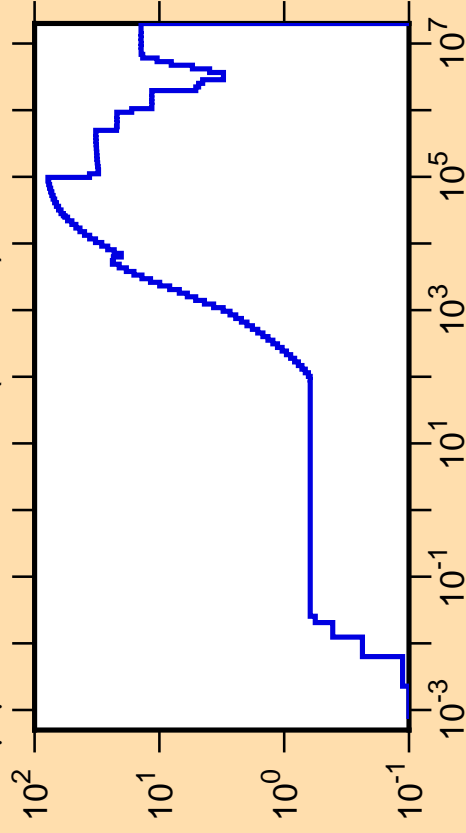
\Delta\mu/\mu vs. E for ^{149}\text{Sm}(\text{mt251})
