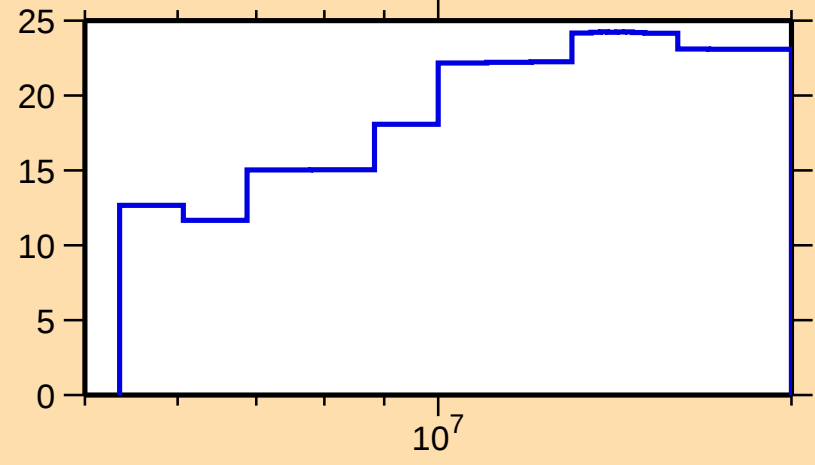
\Delta\sigma/\sigma vs. E for ^{149}\text{Sm}(n,\text{inel.})
