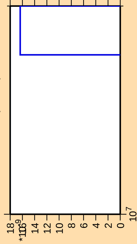
\Delta\sigma/\sigma vs. E for ^{149}\text{Sm}(\text{mt } 11)
