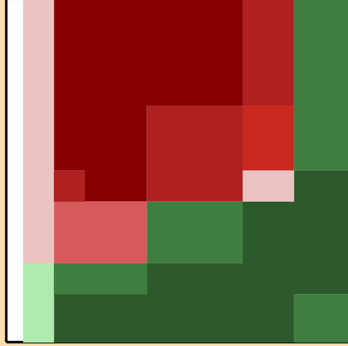
\Delta\sigma/\sigma vs. E for ^{149}\text{Sm}(n,2n)
