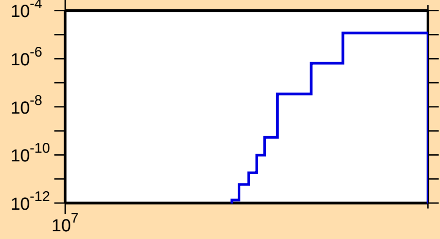
\sigma vs. E for ^{149}\text{Sm}(n,\text{nd})
