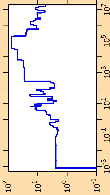
\Delta\sigma/\sigma vs. E for ^{149}\text{Sm}(n,\text{el.})
