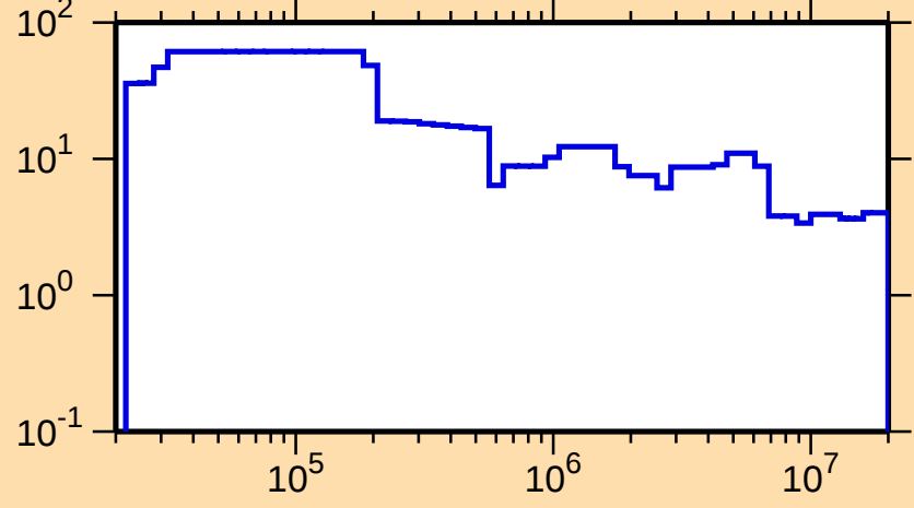
\Delta\sigma/\sigma vs. E for ^{149}\text{Sm}(n,\text{tot.})
