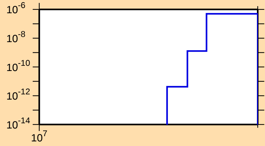
\sigma vs. E for ^{149}\text{Sm}(n,\text{nt})
