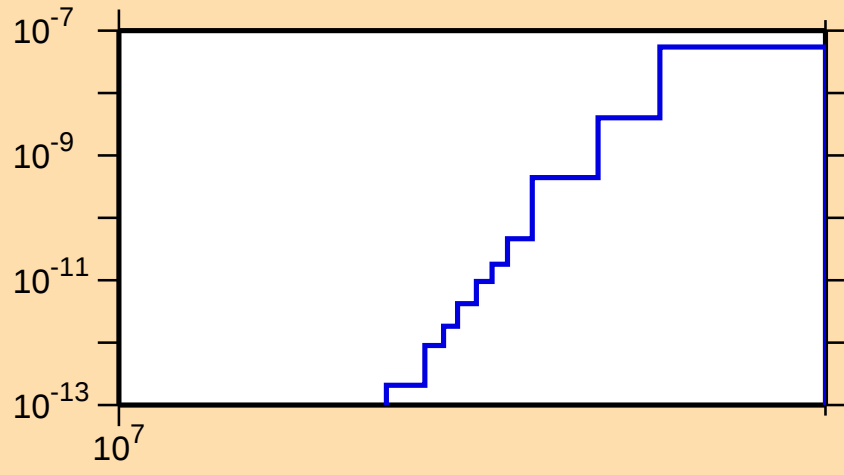
\sigma vs. E for ^{149}\text{Sm}(n,\text{He}3)
