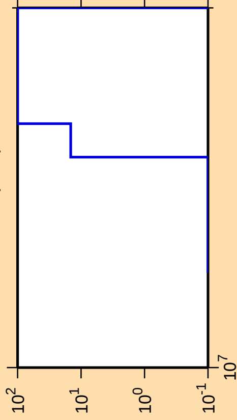
\Delta\sigma/\sigma vs. E for ^{149}\text{Sm}(n,\text{nt})
