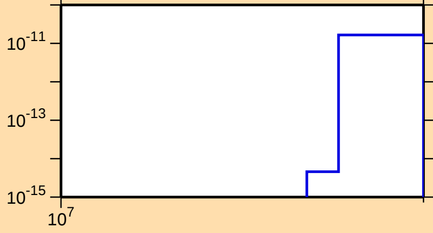
\sigma vs. E for ^{149}\text{Sm}(n,3n\alpha)
