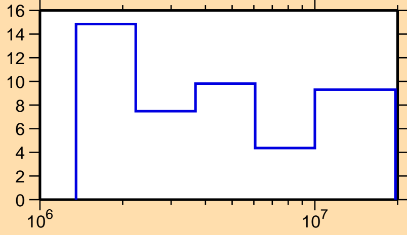
\Delta\sigma/\sigma vs. E for ^{149}\text{Sm}(n,el.)
