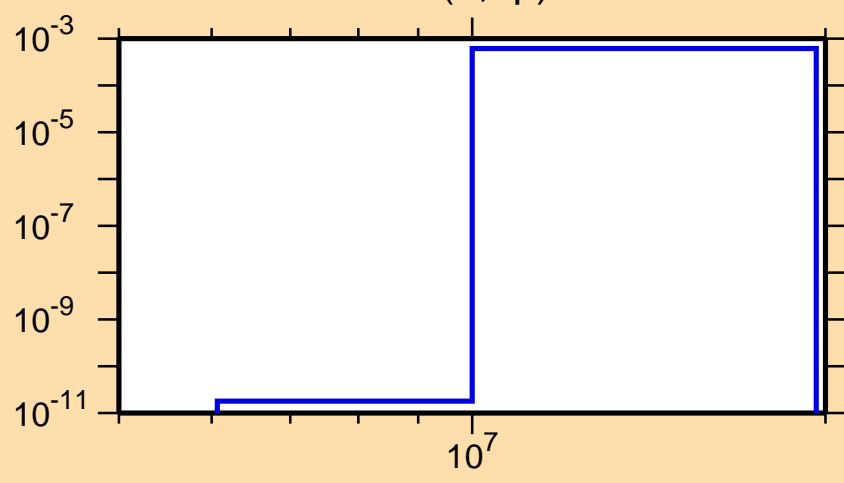
\sigma vs. E for ^{149}\text{Sm}(n,np)
