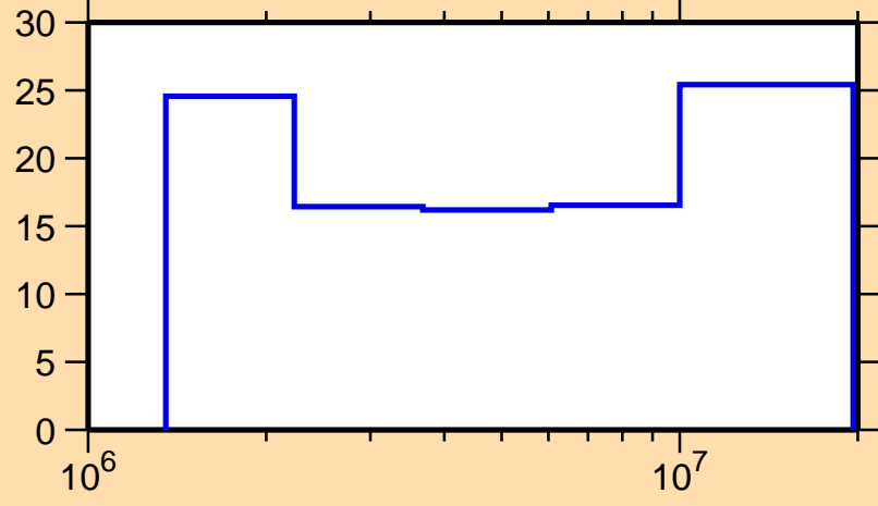
\Delta\sigma/\sigma vs. E for ^{149}\text{Sm}(n,ncont.)
