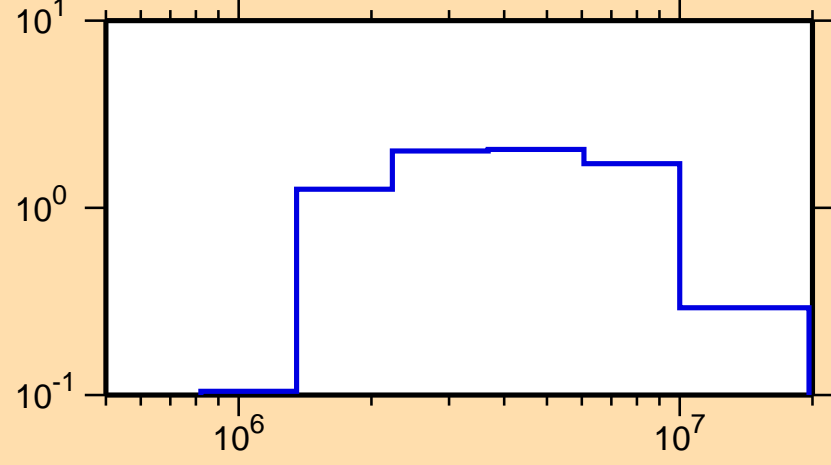
\sigma vs. E for ^{149}\text{Sm}(n,n\text{cont.})
