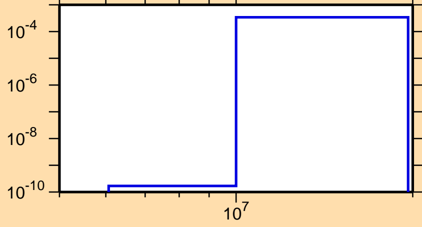
\sigma vs. E for ^{149}\text{Sm}(n,t)
