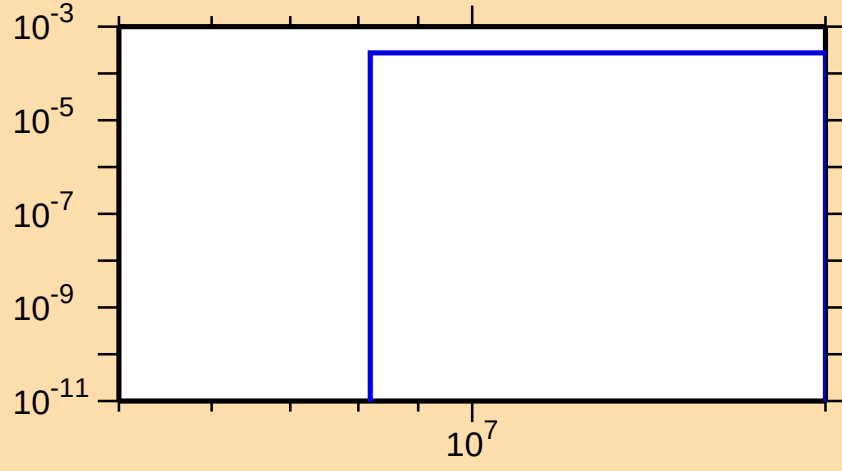
\sigma vs. E for ^{149}\text{Sm}(n,t)
