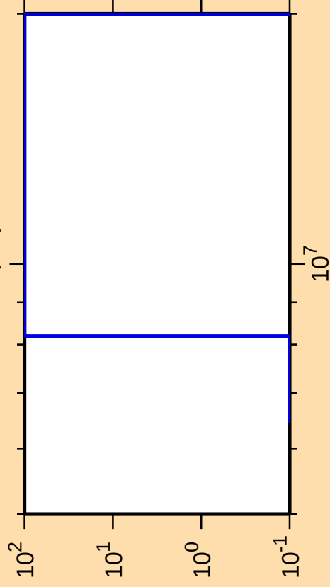
\Delta\sigma/\sigma vs. E for ^{149}\text{Sm}(n,t)
