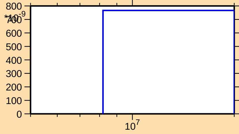
\sigma vs. E for ^{149}\text{Sm}(n,2n\alpha)
