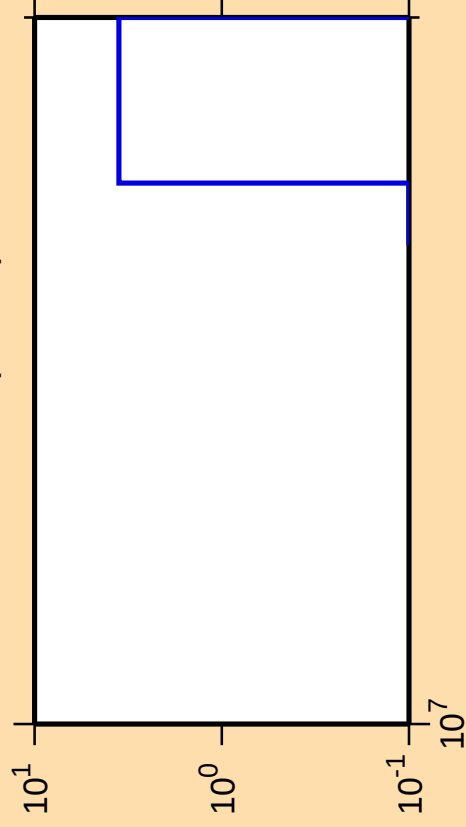
\Delta\sigma/\sigma vs. E for ^{150}\text{Sm}(n,3n\alpha)
