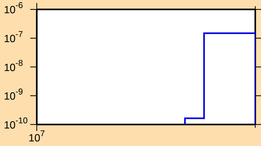
\sigma vs. E for ^{150}\text{Sm}(n,nt)
