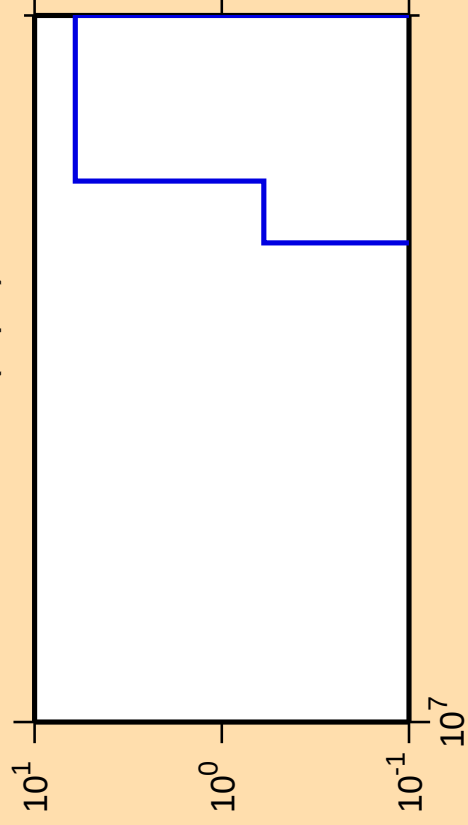
\Delta\sigma/\sigma vs. E for ^{150}\text{Sm}(n,p\alpha)
