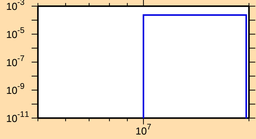
\sigma vs. E for ^{150}\text{Sm}(n,np)
