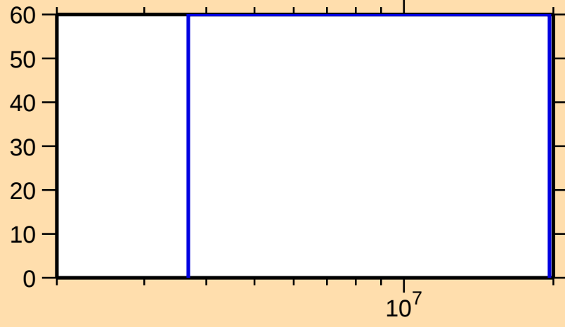
\Delta\sigma/\sigma vs. E for ^{150}\text{Sm}(n,\gamma)
