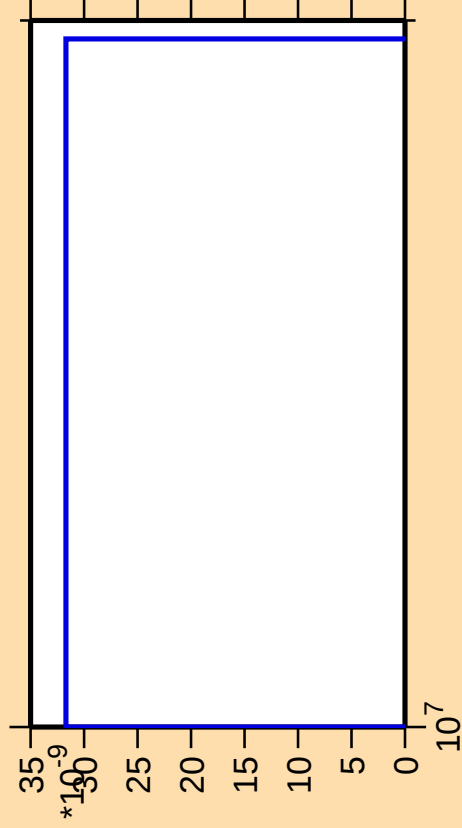
\Delta\sigma/\sigma vs. E for ^{150}\text{Sm}(\text{mt } 11)
