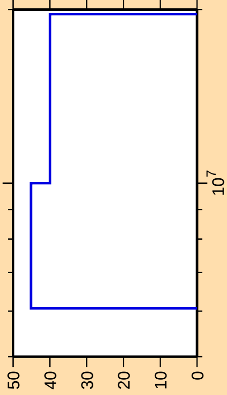
\Delta\sigma/\sigma vs. E for ^{150}\text{Sm}(n,n_1)
