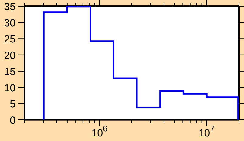
\Delta\sigma/\sigma vs. E for ^{150}\text{Sm}(n,\text{nonel.})
