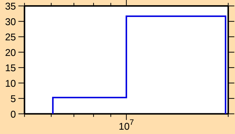
\Delta\sigma/\sigma vs. E for ^{150}\text{Sm}(n,\text{inel.})
