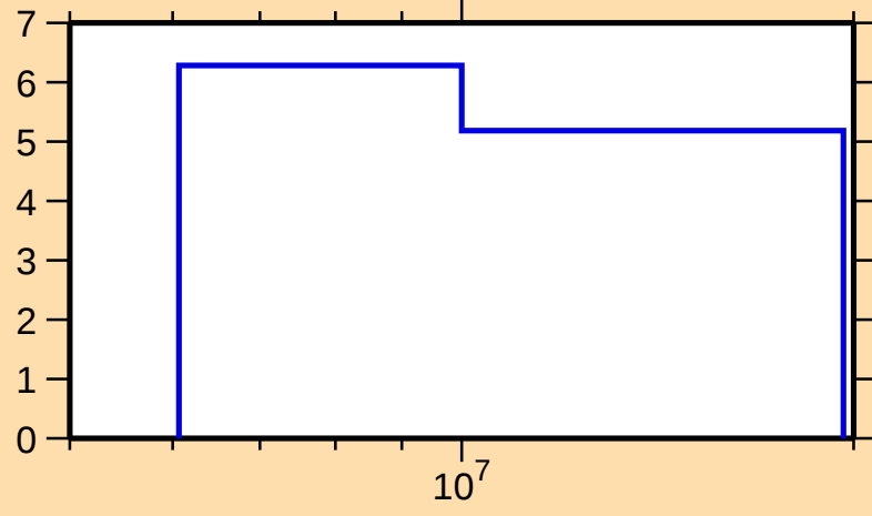
\Delta\sigma/\sigma vs. E for ^{150}\text{Sm}(n,\text{tot.})
