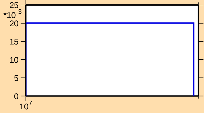
\sigma vs. E for ^{150}\text{Sm}(n,3n)
