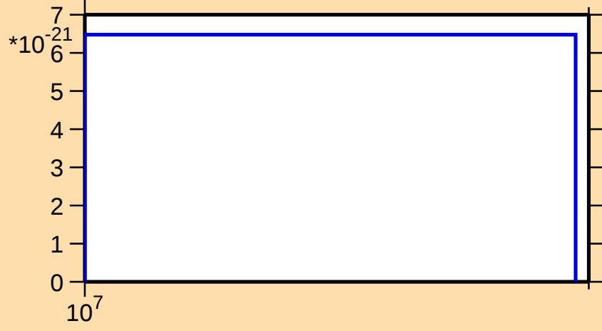
\sigma vs. E for ^{150}\text{Sm}(\text{mt } 11)
