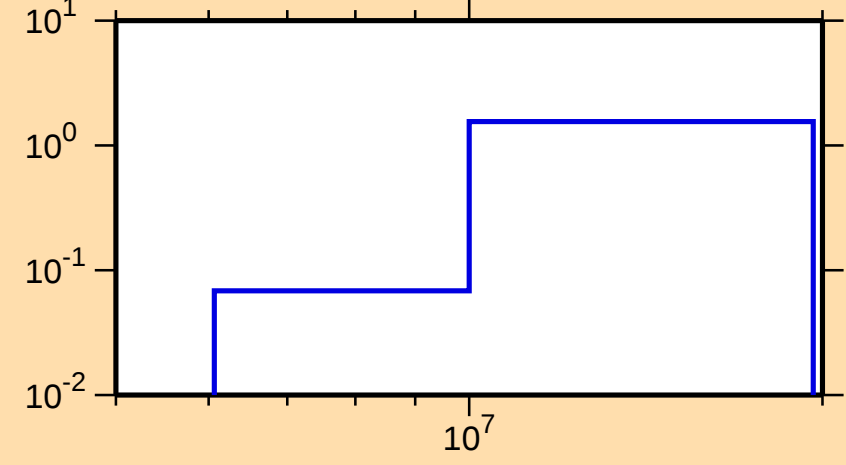
\sigma vs. E for ^{150}\text{Sm}(n,2n)
