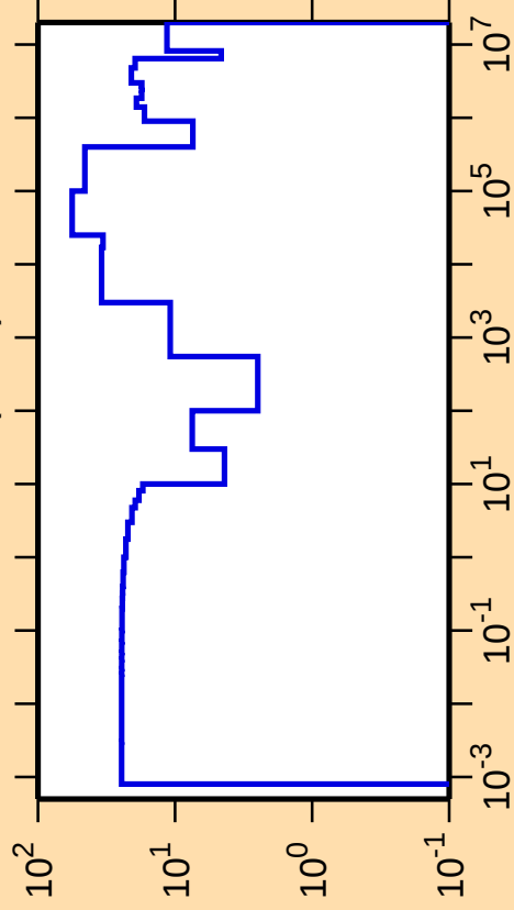
\Delta\sigma/\sigma vs. E for ^{150}\text{Sm}(n,\text{el.})
