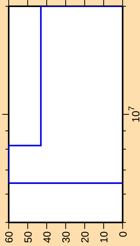
\Delta\sigma/\sigma vs. E for ^{150}\text{Sm}(n,\alpha)
