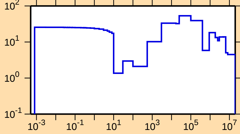
\Delta\sigma/\sigma vs. E for ^{150}\text{Sm}(n,\text{tot.})
