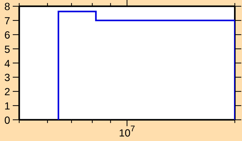
\Delta\sigma/\sigma vs. E for ^{150}\text{Sm}(n,\text{nonel.})
