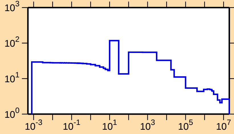
\sigma vs. E for ^{150}\text{Sm}(n,\text{el.})
