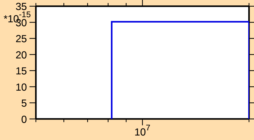
\sigma vs. E for ^{150}\text{Sm}(n,3n\alpha)
