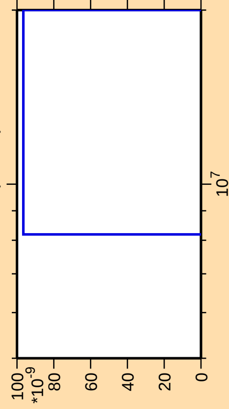
\Delta\sigma/\sigma vs. E for ^{150}\text{Sm}(\text{mt } 11)
