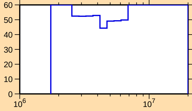
\Delta\sigma/\sigma vs. E for ^{157}\text{Sm}(n,\gamma)
