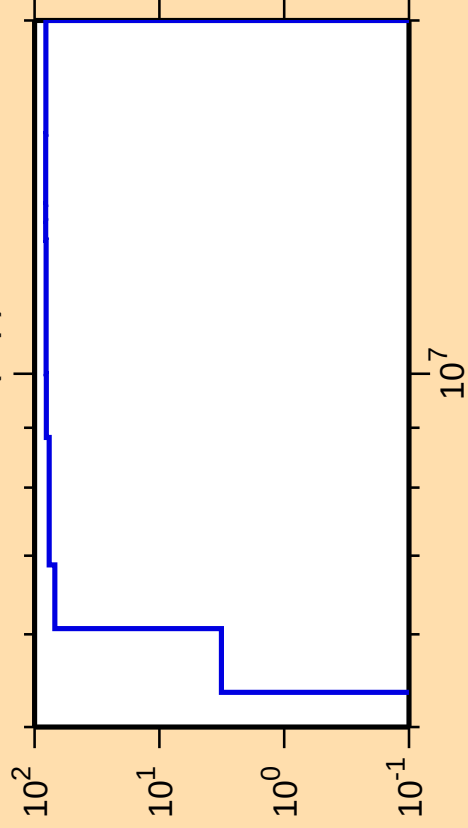
\Delta\sigma/\sigma vs. E for ^{157}\text{Sm}(n,p)
