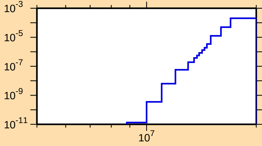
\sigma vs. E for ^{157}\text{Sm}(n,n\alpha)
