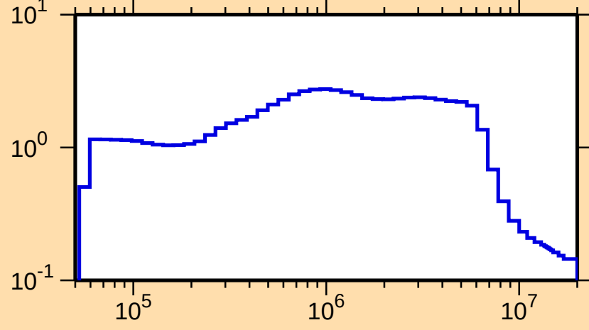
\sigma vs. E for ^{157}\text{Sm}(n,\text{inel.})
