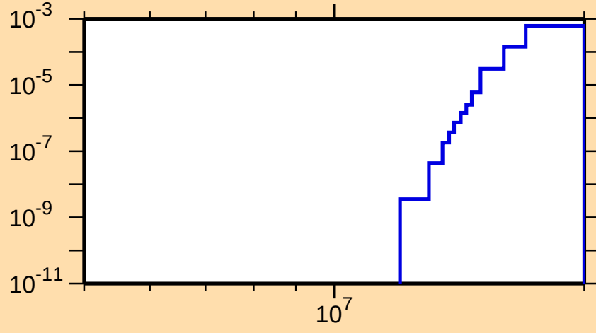
\sigma vs. E for ^{157}\text{Sm}(n,np)
