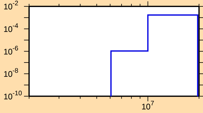
\sigma vs. E for ^{157}\text{Sm}(n,p)
