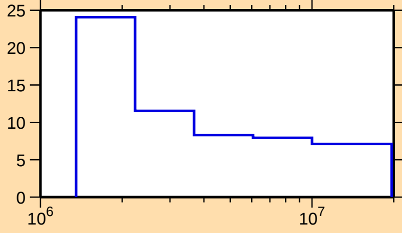
\Delta\sigma/\sigma vs. E for ^{157}\text{Sm}(n,n\text{oncl.})
