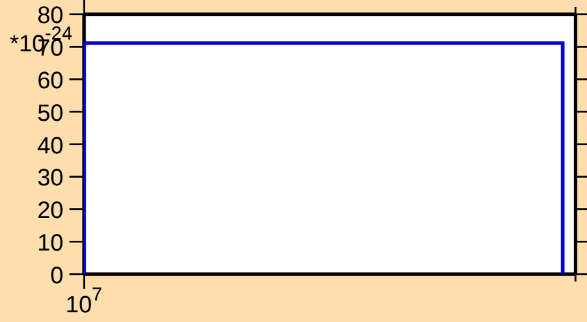
\sigma vs. E for ^{157}\text{Sm}(\text{mt } 11)
