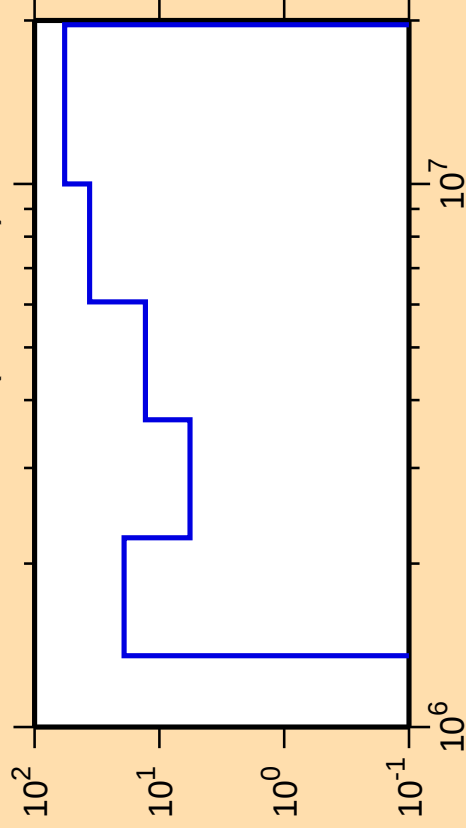
\Delta\sigma/\sigma vs. E for ^{157}\text{Sm}(n,\text{ncont.})
