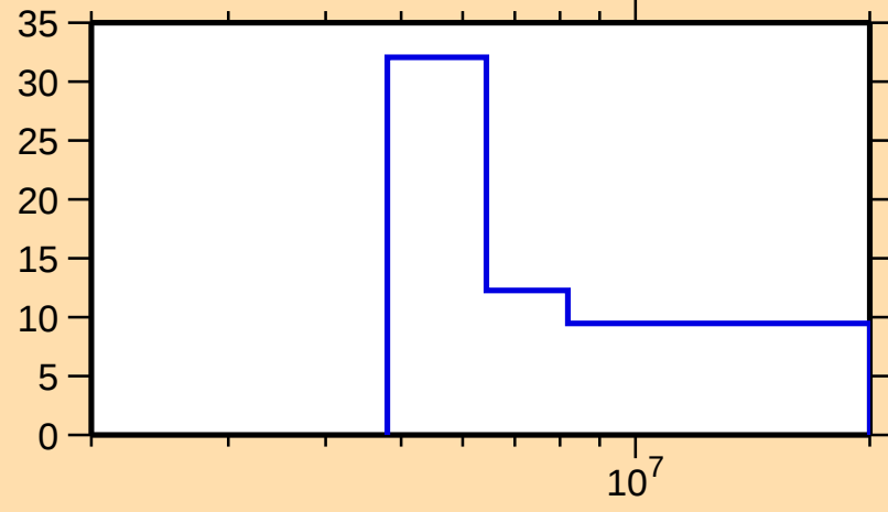
\Delta\sigma/\sigma vs. E for ^{157}\text{Sm}(n,2n)
