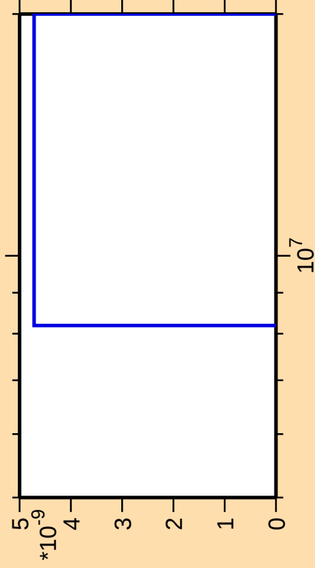
\Delta\sigma/\sigma vs. E for ^{157}\text{Sm}(\text{mt } 11)
