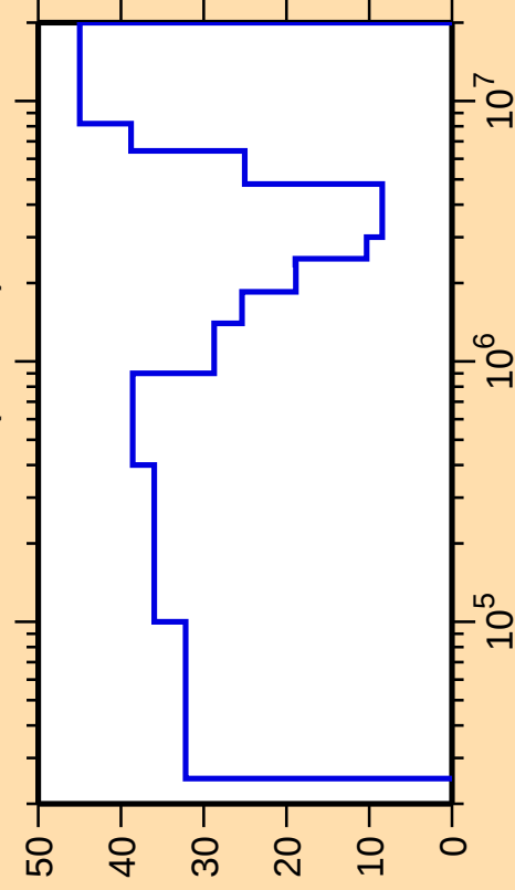
\Delta\sigma/\sigma vs. E for ^{157}\text{Sm}(n,\text{inel.})
