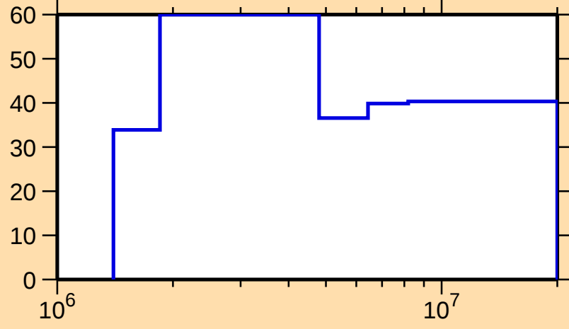
\Delta\sigma/\sigma vs. E for ^{157}\text{Sm}(n,n_1)
