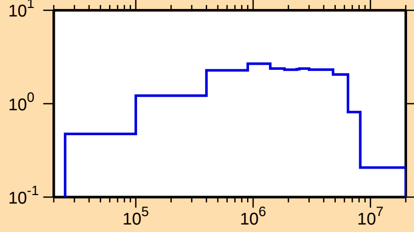
\sigma vs. E for ^{157}\text{Sm}(n,\text{inel.})
