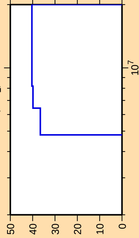
\Delta\sigma/\sigma vs. E for ^{157}\text{Sm}(n,n_1)
