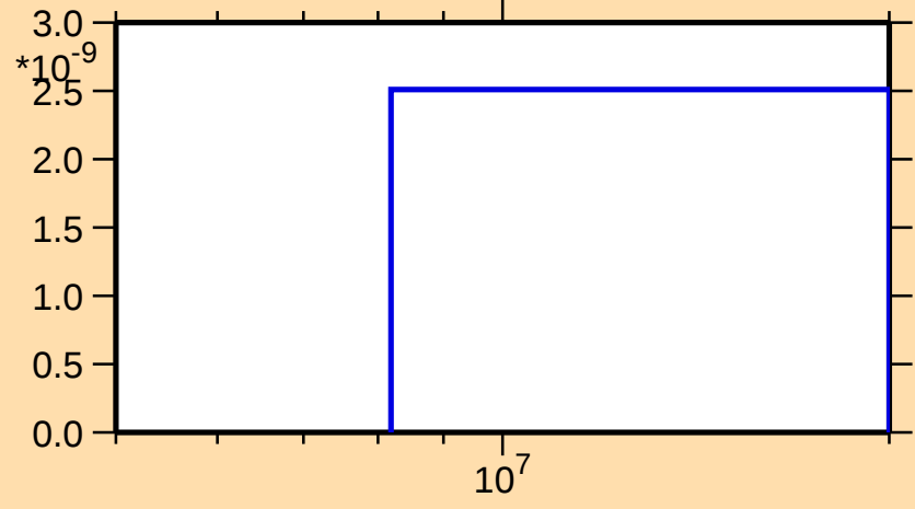
\sigma vs. E for ^{157}\text{Sm}(n,\text{nd})
