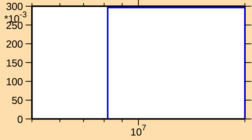
\sigma vs. E for ^{157}\text{Sm}(n,3n)
