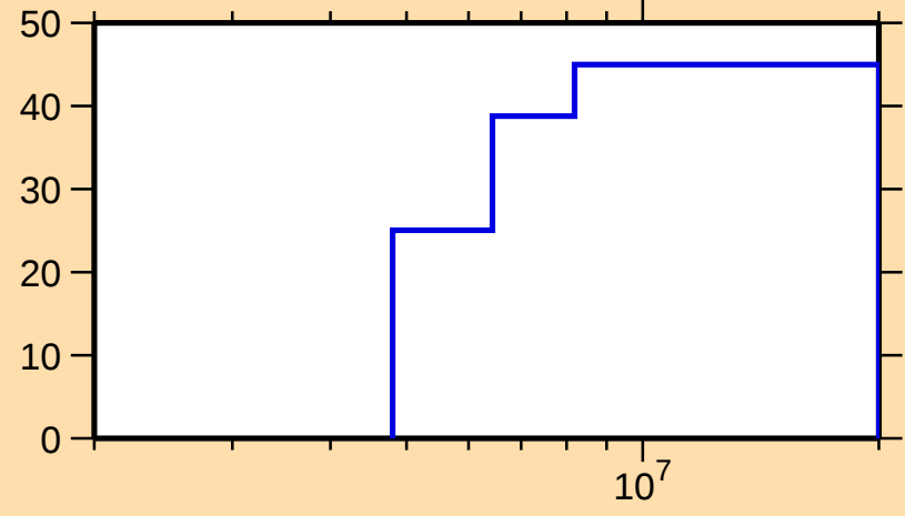
\Delta\sigma/\sigma vs. E for ^{157}\text{Sm}(n,\text{inel.})
