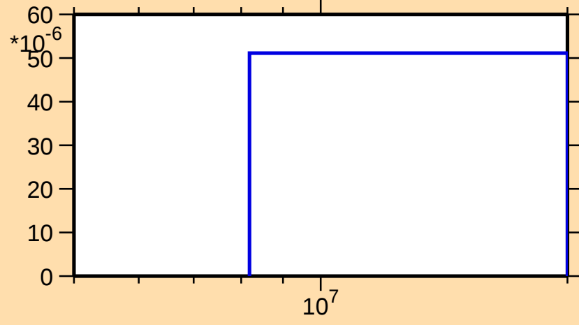
\sigma vs. E for ^{157}\text{Sm}(n,d)
