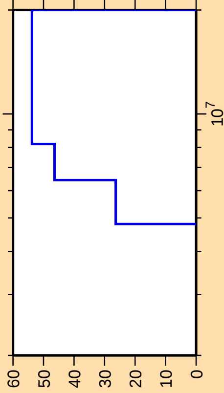
\Delta\sigma/\sigma vs. E for ^{157}\text{Sm}(n,n\text{cont.})
