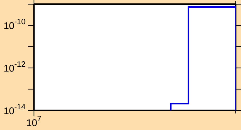
\sigma vs. E for ^{143}\text{Tb}(n,nt)
