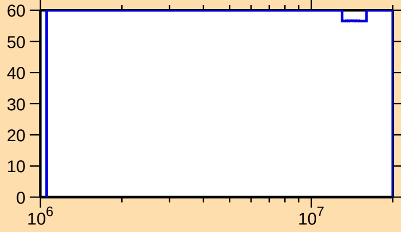
\Delta\sigma/\sigma vs. E for ^{143}\text{Tb}(n,ncont.)
