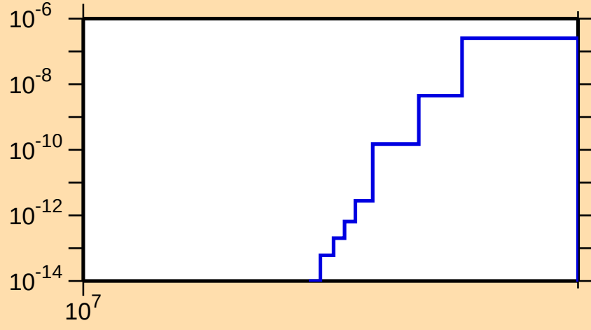
\sigma vs. E for ^{143}\text{Tb}(n,\text{pt})
