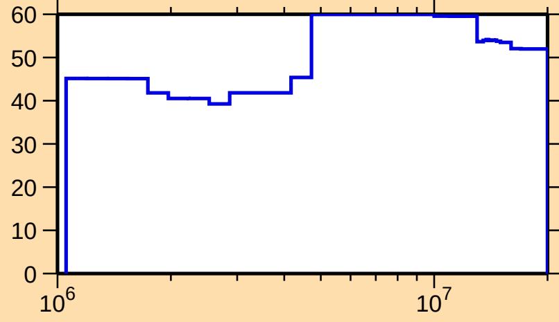
\Delta\sigma/\sigma vs. E for ^{143}\text{Tb}(n,\text{tot.})
