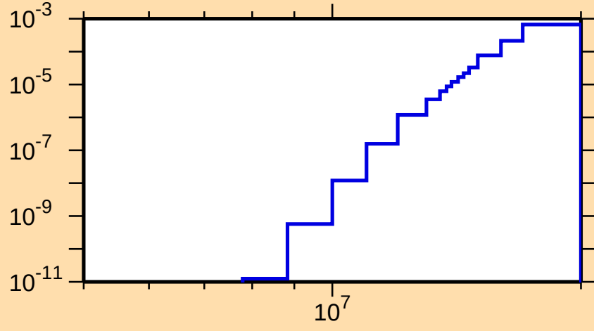
\sigma vs. E for ^{143}\text{Tb}(\text{mt } 45)
