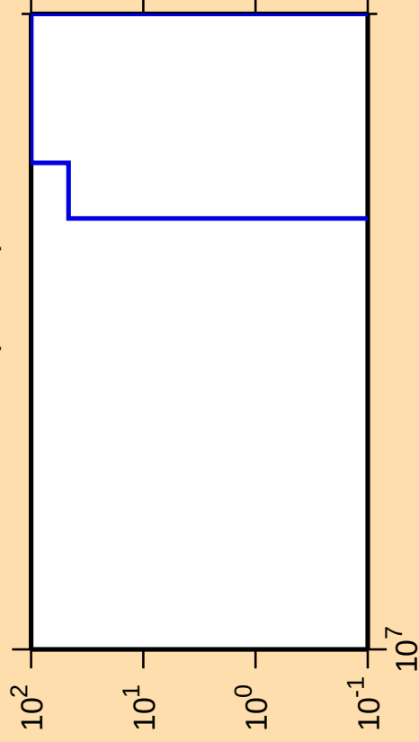
\Delta\sigma/\sigma vs. E for ^{143}\text{Tb}(\text{mt } 34)
