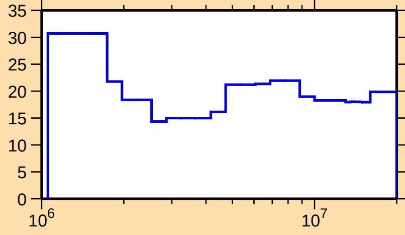
\Delta\sigma/\sigma vs. E for ^{143}\text{Tb}(n,n\text{onel.})
