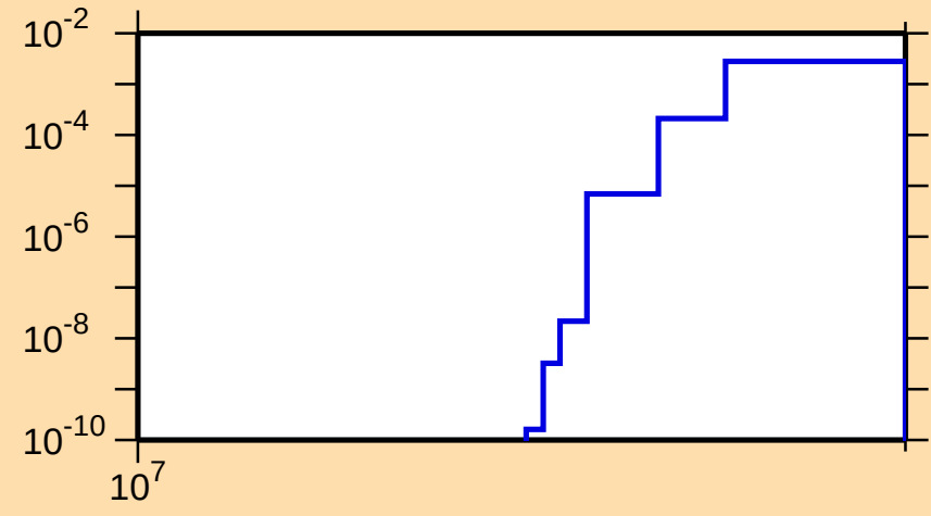
\sigma vs. E for ^{143}\text{Tb}(n,2np)
