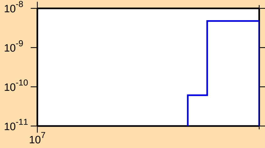
\sigma vs. E for ^{143}\text{Tb}(n,2n\alpha)
