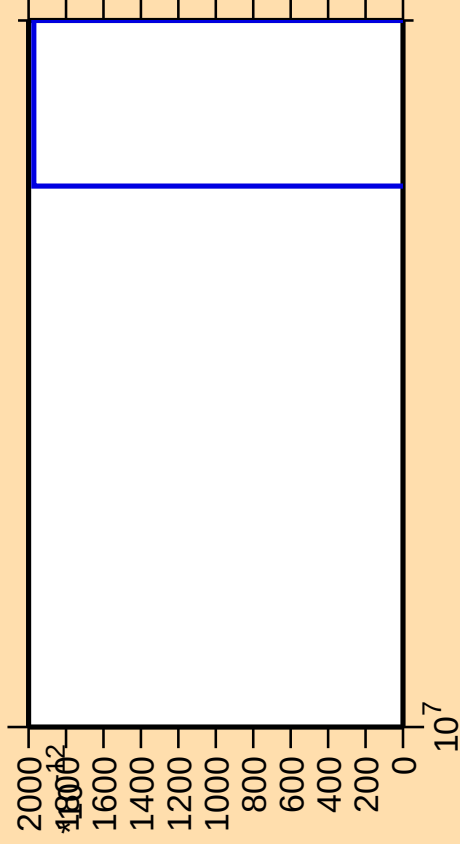
\Delta\sigma/\sigma vs. E for ^{143}\text{Tb}(\text{mt } 11)
