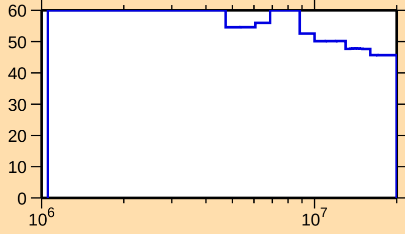
\Delta\sigma/\sigma vs. E for ^{143}\text{Tb}(n,n_1)
