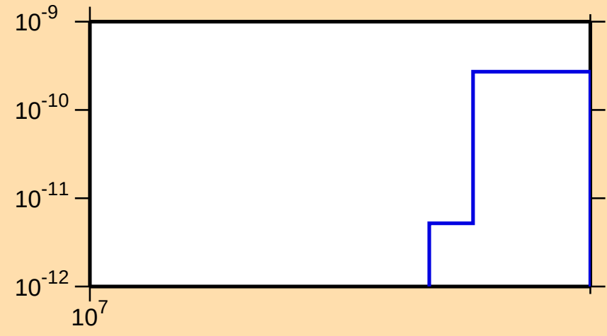
\sigma vs. E for ^{143}\text{Tb}(\text{mt } 34)
