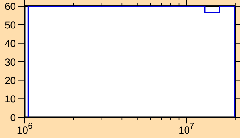
\Delta\sigma/\sigma vs. E for ^{143}\text{Tb}(n,n\text{cont.})
