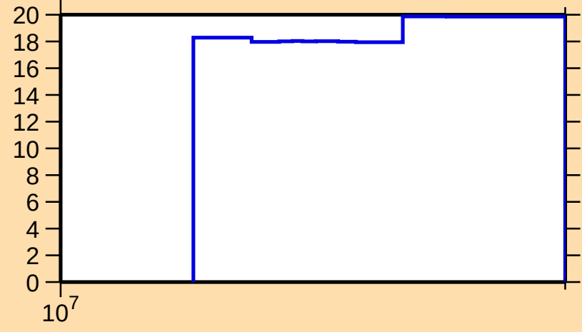
\Delta\sigma/\sigma vs. E for ^{143}\text{Tb}(n,\text{nonel.})
