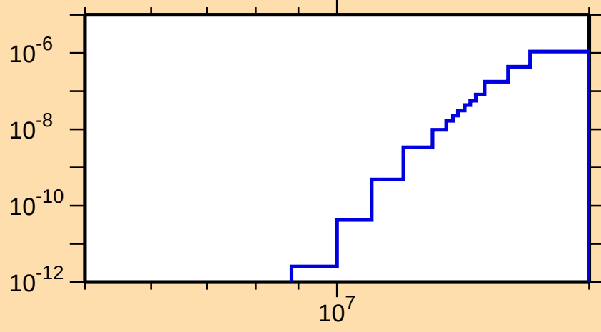
\sigma vs. E for ^{143}\text{Tb}(\text{mt117})
