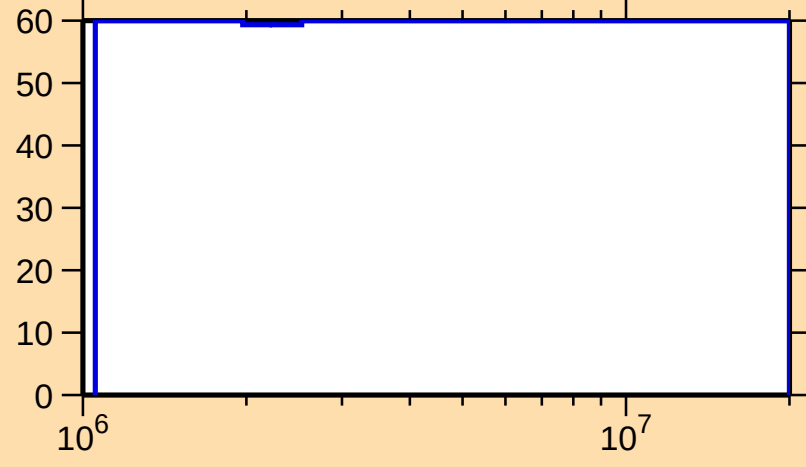
\Delta\sigma/\sigma vs. E for ^{143}\text{Tb}(n,\text{el.})
