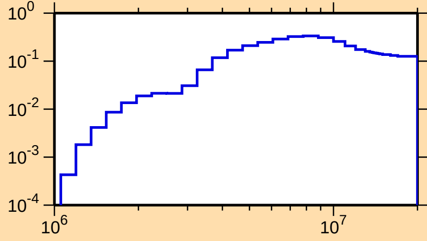
\sigma vs. E for ^{143}\text{Tb}(n,n\text{cont.})
