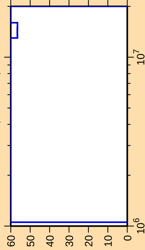
\Delta\sigma/\sigma vs. E for ^{143}\text{Tb}(n,\text{ncont.})
