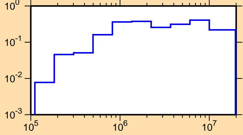
\sigma vs. E for ^{143}\text{Tb}(n,\text{inel.})
