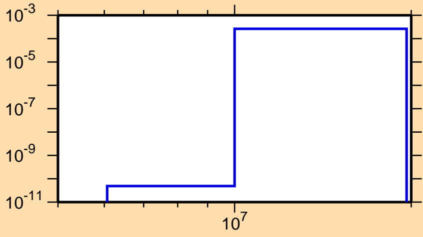
\sigma vs. E for ^{143}\text{Tb}(n,t)
