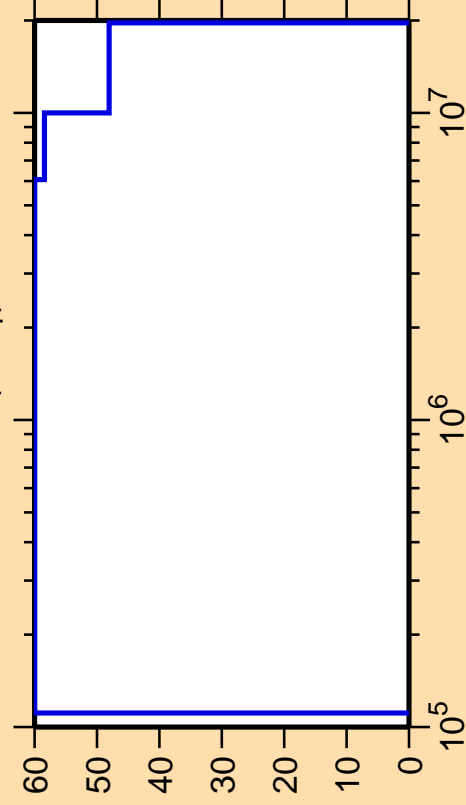
\Delta\sigma/\sigma vs. E for ^{143}\text{Tb}(n,n_1)
