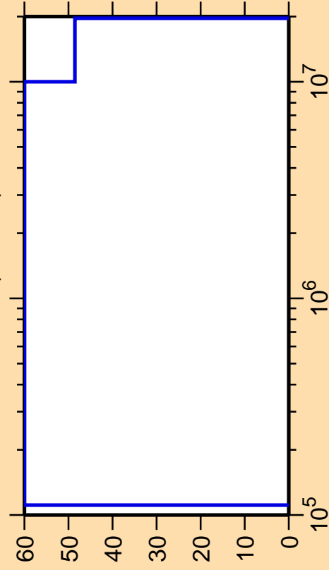
\Delta\sigma/\sigma vs. E for ^{143}\text{Tb}(n,\text{inel.})
