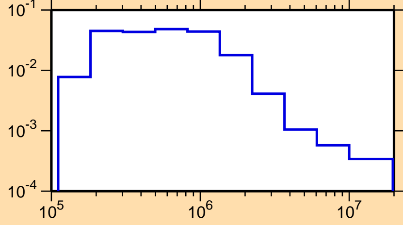
\sigma vs. E for ^{143}\text{Tb}(n,n_1)
