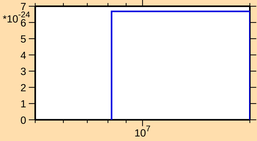
\sigma vs. E for ^{143}\text{Tb}(\text{mt } 11)
