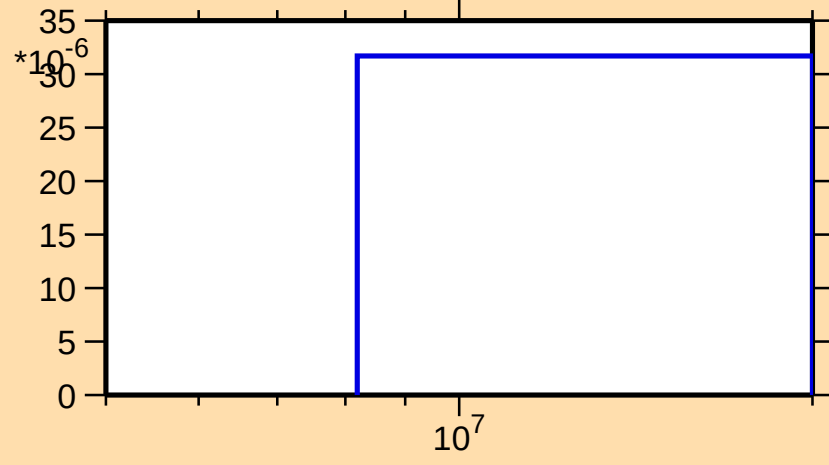
\sigma vs. E for ^{143}\text{Tb}(n,2np)
