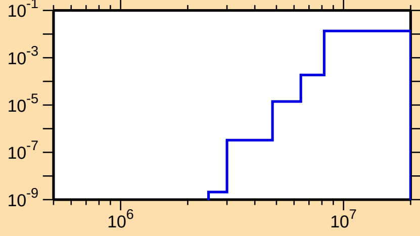
\sigma vs. E for ^{143}\text{Tb}(n,d)
