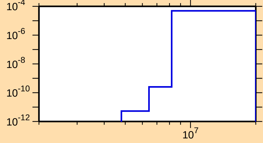
\sigma vs. E for ^{143}\text{Tb}(n,\text{He3})
