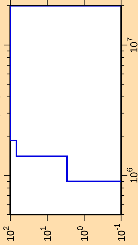
\Delta\sigma/\sigma vs. E for ^{143}\text{Tb}(n,d)
