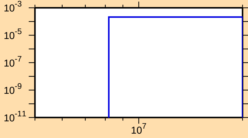
\sigma vs. E for ^{143}\text{Tb}(n,t)
