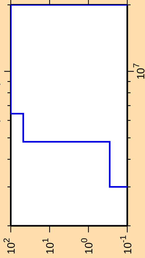
\Delta\sigma/\sigma vs. E for ^{143}\text{Tb}(n,\text{He3})
