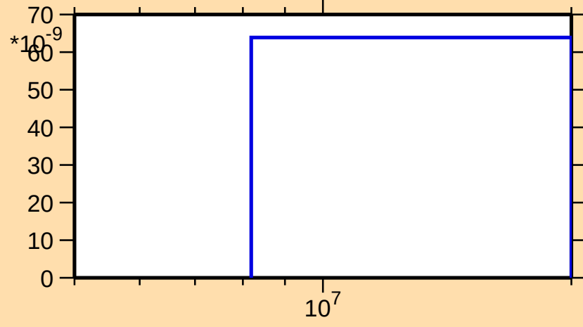
\sigma vs. E for ^{143}\text{Tb}(\text{mt117})
