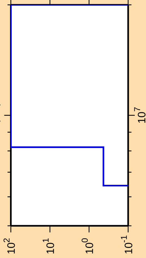
\Delta\sigma/\sigma vs. E for ^{143}\text{Tb}(n,t)
