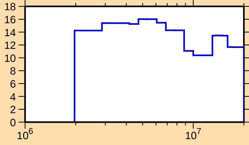
\Delta\sigma/\sigma vs. E for ^{147}\text{Tb}(n,n\text{onel.})
