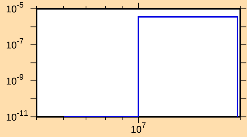
\sigma vs. E for ^{147}\text{Tb}(n,\text{He3})
