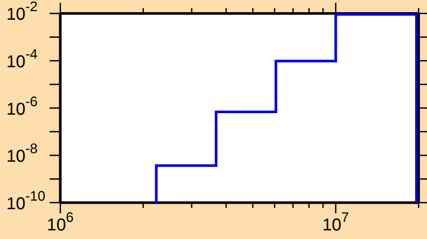
\sigma vs. E for ^{147}\text{Tb}(n,d)
