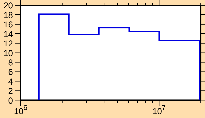
\Delta\sigma/\sigma vs. E for ^{147}\text{Tb}(n,n\text{nonel.})
