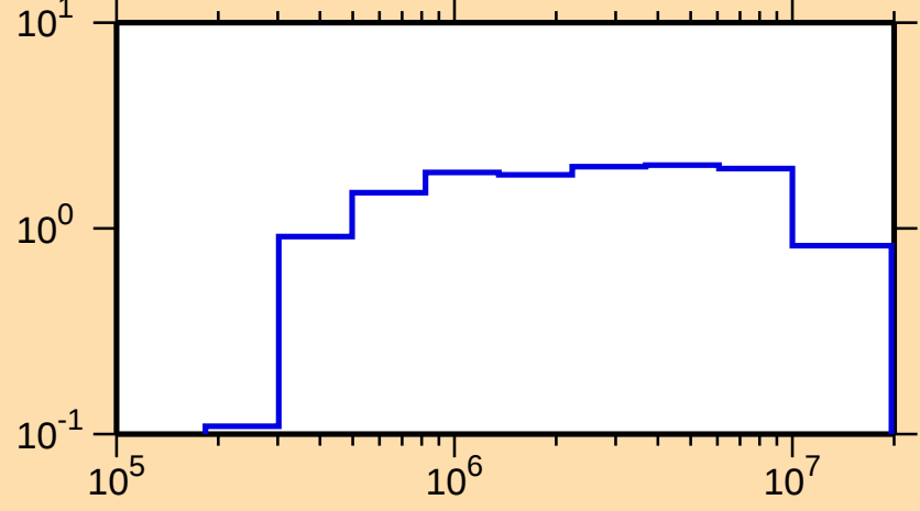
\sigma vs. E for ^{147}\text{Tb}(n,\text{inel.})
