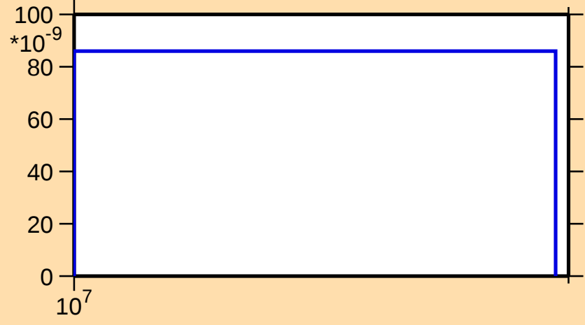
\sigma vs. E for ^{147}\text{Tb}(n,\text{nd})
