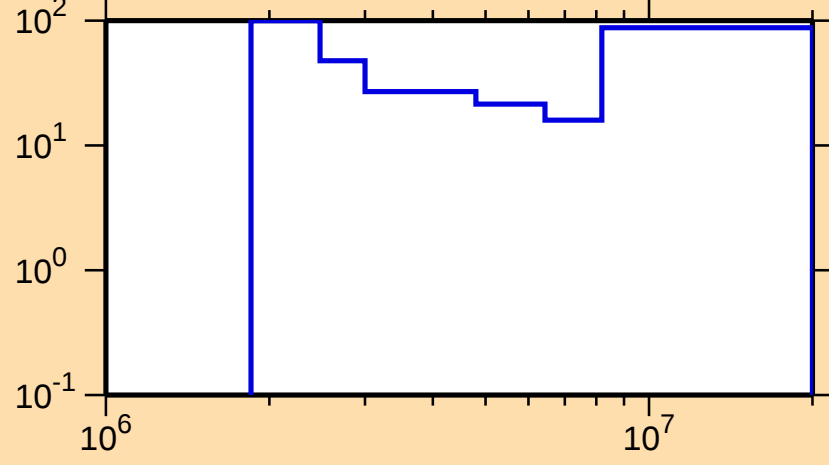
\Delta\sigma/\sigma vs. E for ^{147}\text{Tb}(n,n\text{cont.})
