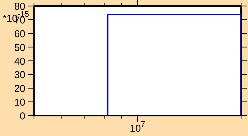
\sigma vs. E for ^{147}\text{Tb}(\text{mt } 34)
