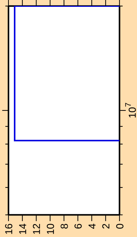
\Delta\sigma/\sigma vs. E for ^{147}\text{Tb}(n,\text{nt})
