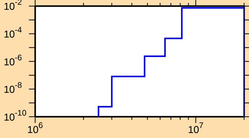
\sigma vs. E for ^{147}\text{Tb}(n,d)
