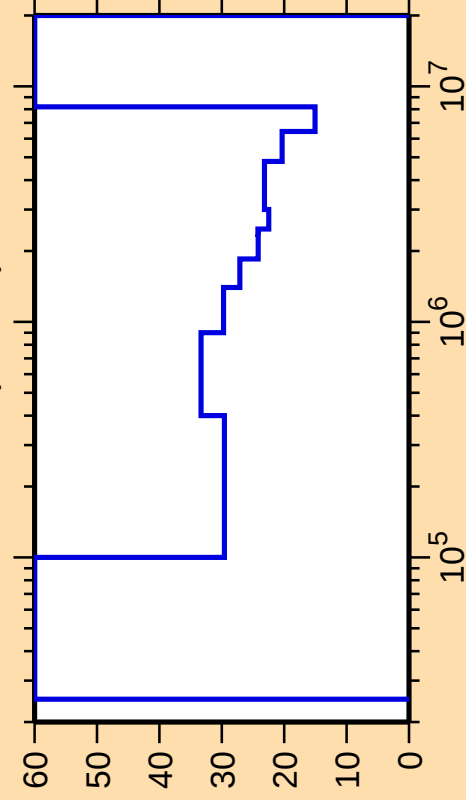
\Delta\sigma/\sigma vs. E for ^{147}\text{Tb}(n,\text{inel.})
