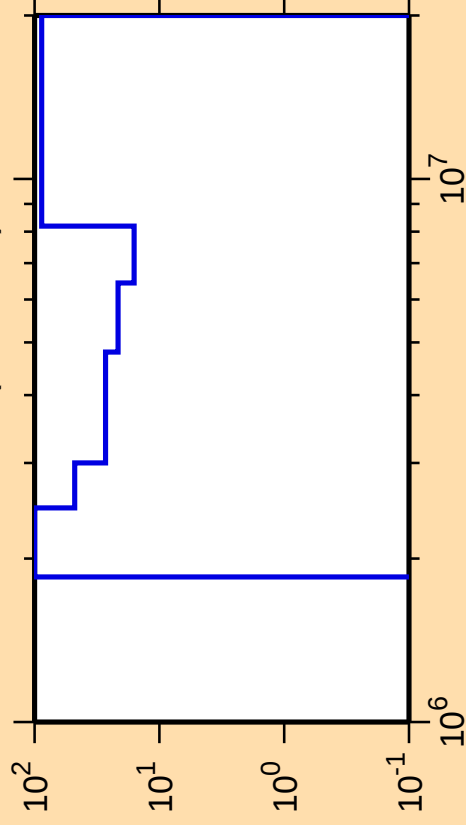
\Delta\sigma/\sigma vs. E for ^{147}\text{Tb}(n,n_{\text{cont}}) .
