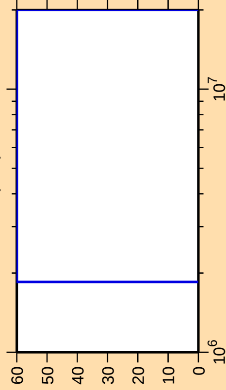
\Delta\sigma/\sigma vs. E for ^{147}\text{Tb}(n,\alpha)
