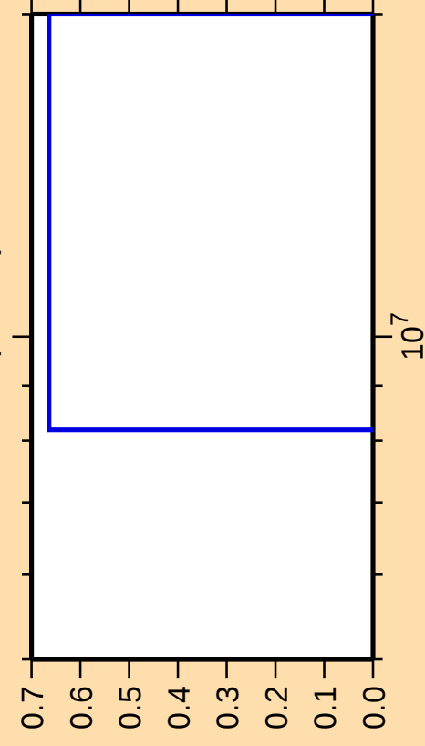
\Delta\sigma/\sigma vs. E for ^{147}\text{Tb}(\text{mt } 34)
