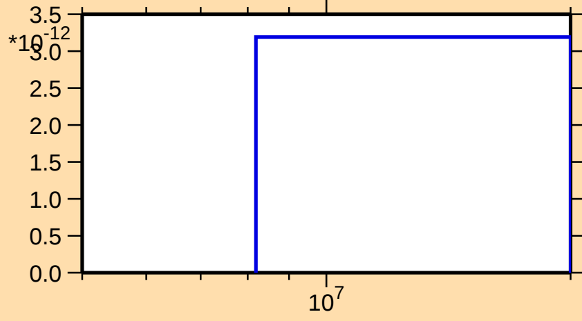
\sigma vs. E for ^{147}\text{Tb}(n,\text{nt})
