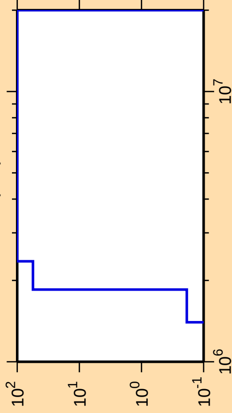
\Delta\sigma/\sigma vs. E for ^{147}\text{Tb}(n,d)
