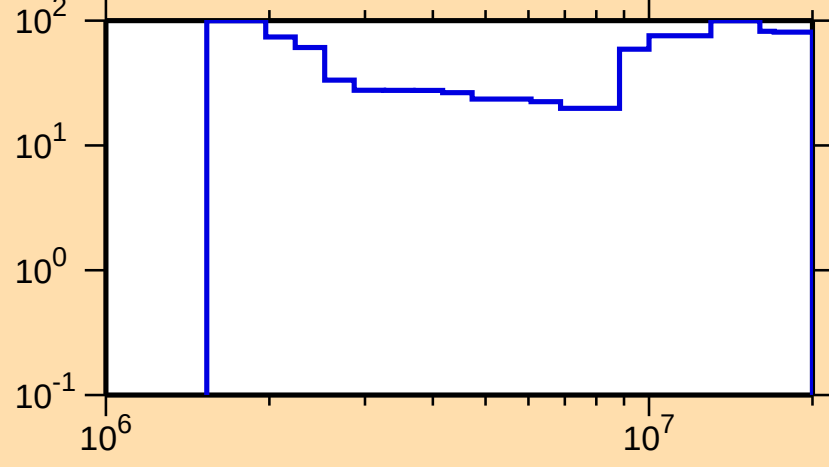
\Delta\sigma/\sigma vs. E for ^{151}\text{Tb}(n,n\text{cont.})
