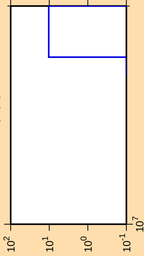
\Delta\sigma/\sigma vs. E for ^{151}\text{Tb}(n,\text{pt})
