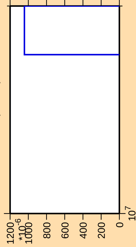
\Delta\sigma/\sigma vs. E for ^{151}\text{Tb} (mt 42)
