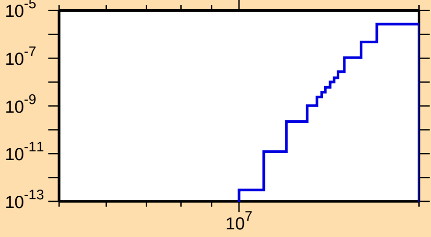
\sigma vs. E for ^{151}\text{Tb}(n,\text{He3})
