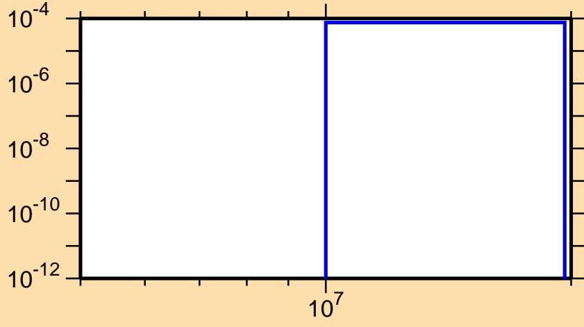
\sigma vs. E for ^{151}\text{Tb}(n,2n\alpha)
