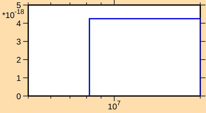
\sigma vs. E for ^{151}\text{Tb}(\text{mt } 42)
