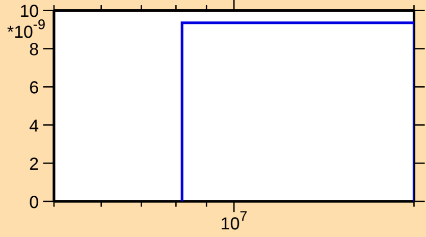
\sigma vs. E for ^{151}\text{Tb}(\text{mt } 45)
