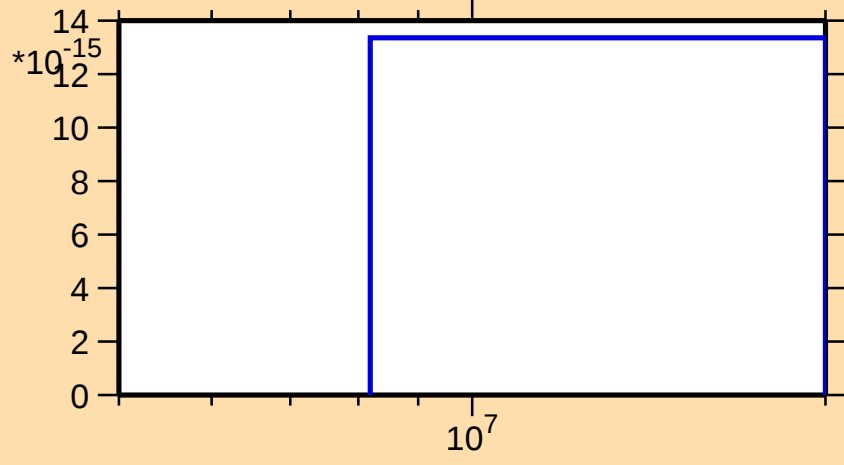
\sigma vs. E for ^{151}\text{Tb}(n,\text{pt})
