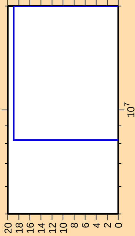
\Delta\sigma/\sigma vs. E for ^{151}\text{Tb}(n,\text{pd})
