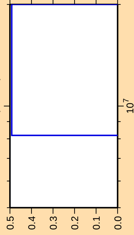
\Delta\sigma/\sigma vs. E for ^{151}\text{Tb}(\text{mt } 34)
