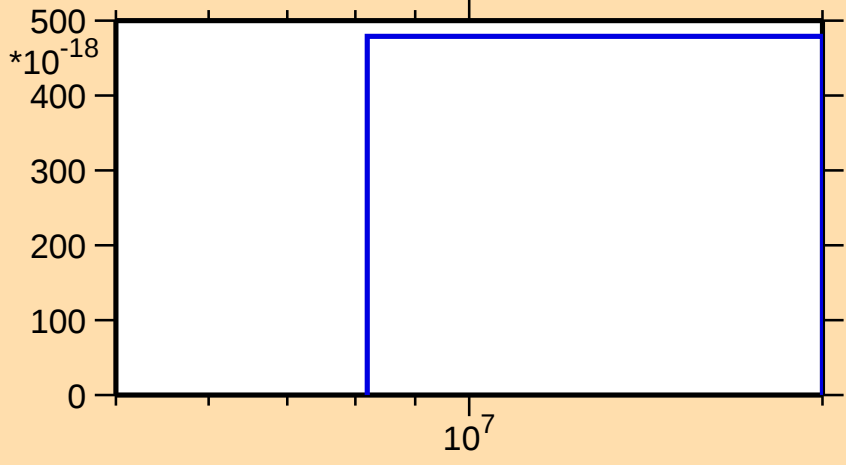
\sigma vs. E for ^{151}\text{Tb}(\text{mt } 11)
