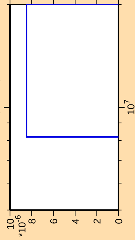
\Delta\sigma/\sigma vs. E for ^{151}\text{Tb}(\text{mt } 42)
