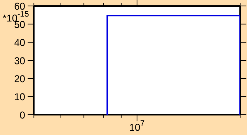
\sigma vs. E for ^{151}\text{Tb}(\text{mt } 34)
