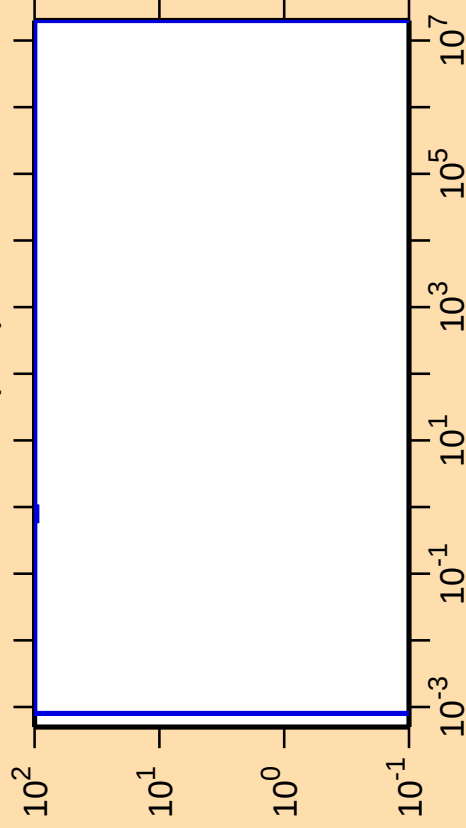
\Delta\sigma/\sigma vs. E for ^{151}\text{Tb}(n,\alpha)
