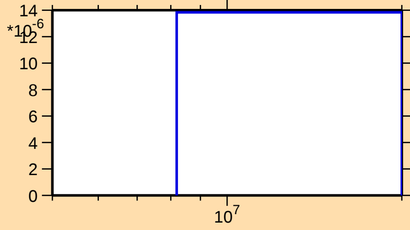
\sigma vs. E for ^{151}\text{Tb}(n,2np)
