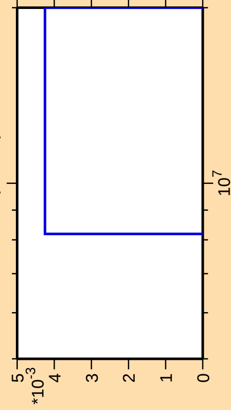
\Delta\sigma/\sigma vs. E for ^{151}\text{Tb}(\text{mt } 11)
