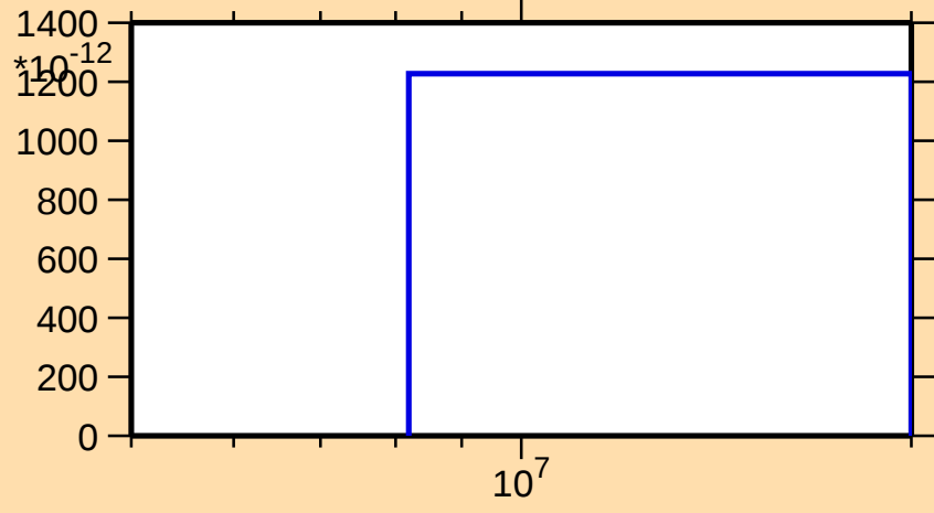
\sigma vs. E for ^{151}\text{Tb}(\text{mt117})
