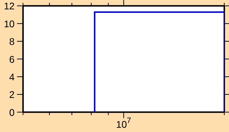
\Delta\sigma/\sigma vs. E for ^{151}\text{Tb}(n,\text{nonel.})
