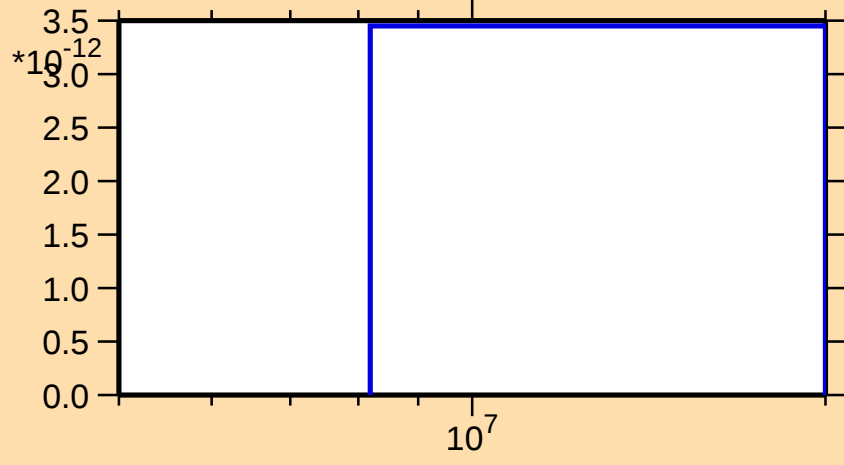
\sigma vs. E for ^{151}\text{Tb}(n,\text{pd})
