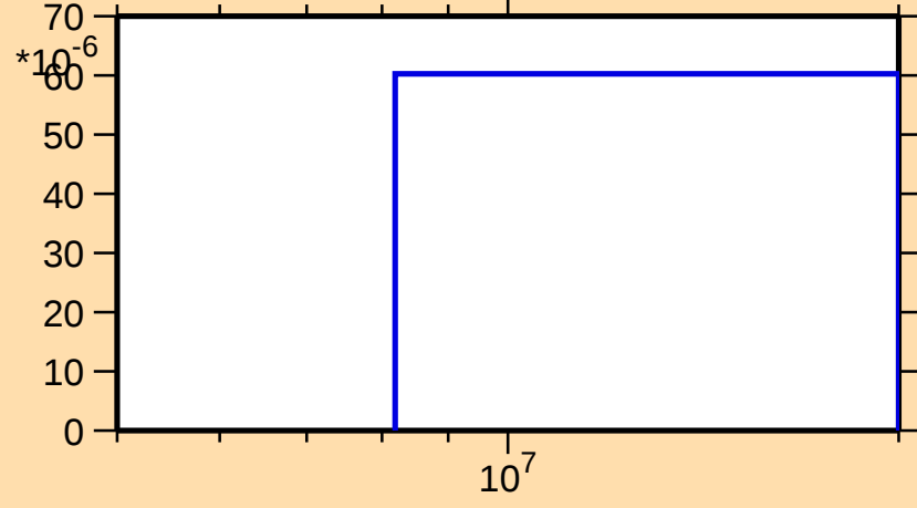
\sigma vs. E for ^{151}\text{Tb}(n,2n\alpha)
