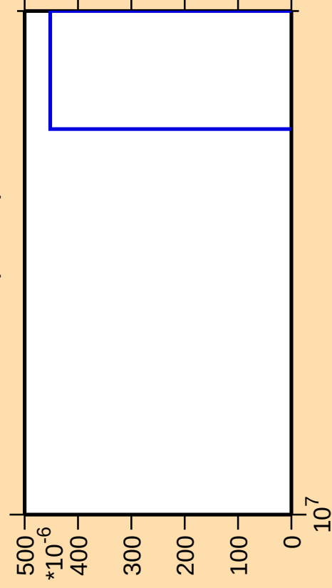
\Delta\sigma/\sigma vs. E for ^{154}\text{Tb} (mt 42)
