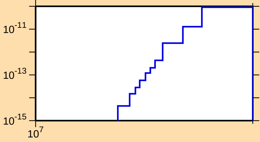
\sigma vs. E for ^{154}\text{Tb}(\text{mt } 45)
