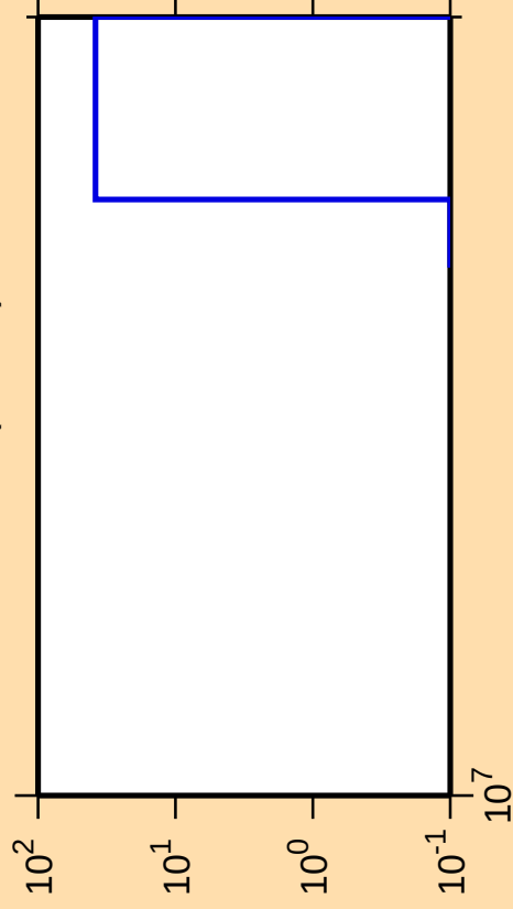
\Delta\sigma/\sigma vs. E for ^{154}\text{Tb} (mt 34)
