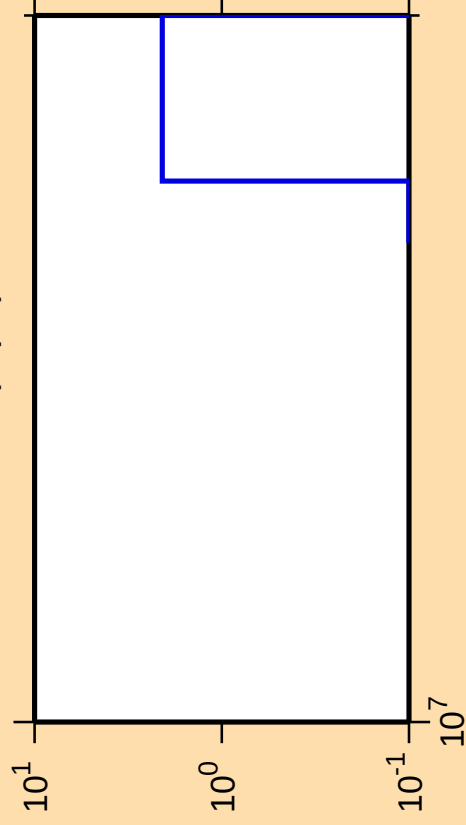
\Delta\sigma/\sigma vs. E for ^{154}\text{Tb}(n,\text{pd})
