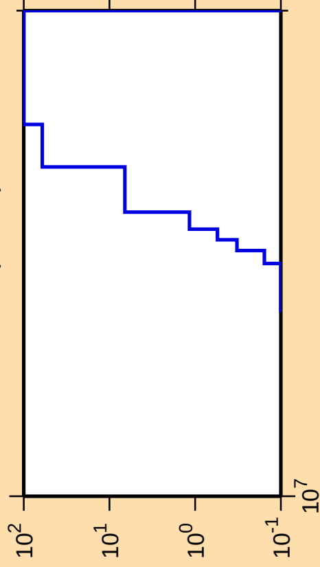
\Delta\sigma/\sigma vs. E for ^{154}\text{Tb}(\text{mt } 45)
