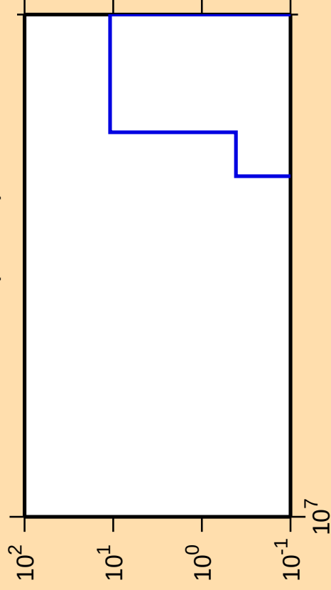
\Delta\sigma/\sigma vs. E for ^{154}\text{Tb}(n,3n\alpha)
