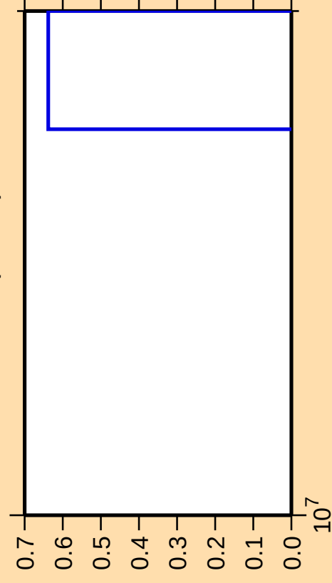
\Delta\sigma/\sigma vs. E for ^{154}\text{Tb}(\text{mt } 11)
