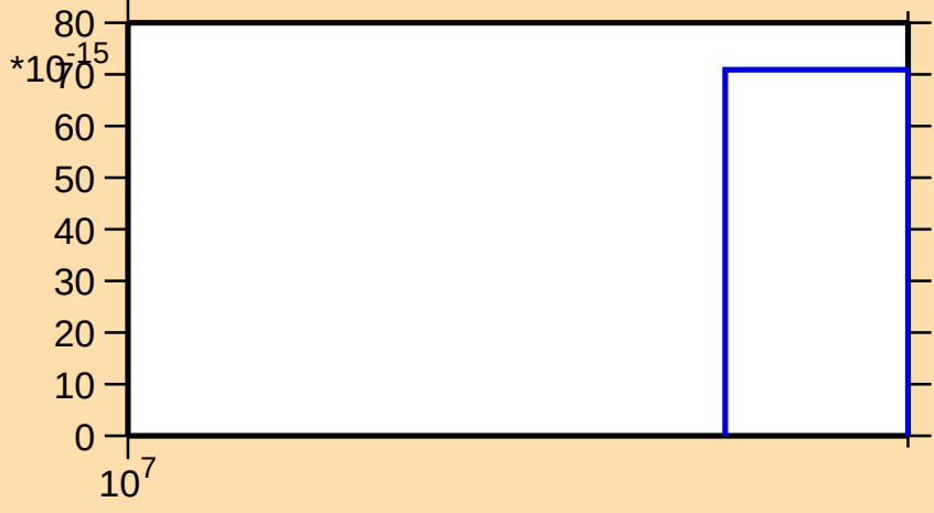
\sigma vs. E for ^{154}\text{Tb}(\text{mt } 11)
