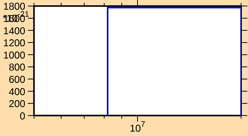
\sigma vs. E for ^{154}\text{Tb}(\text{mt } 42)
