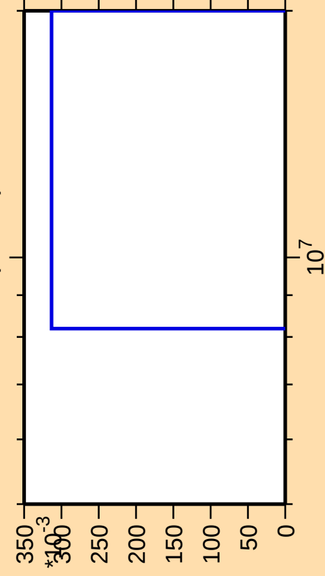
\Delta\sigma/\sigma vs. E for ^{154}\text{Tb}(\text{mt } 34)
