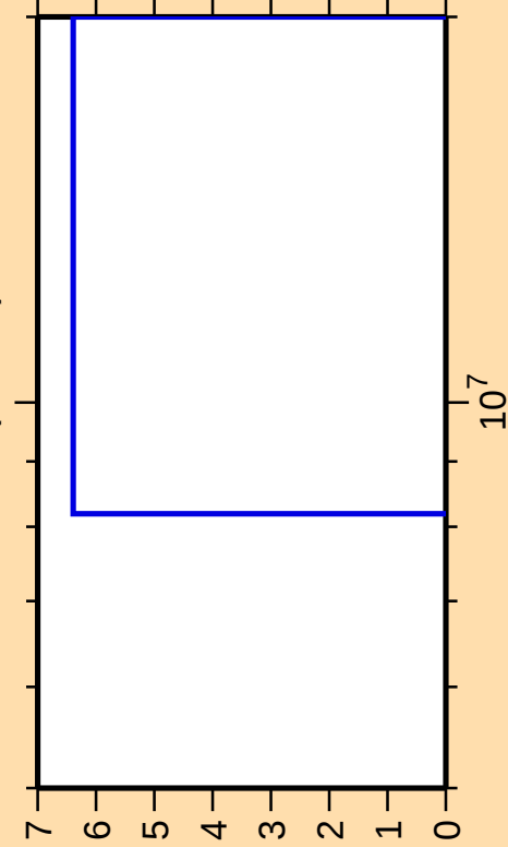
\Delta\sigma/\sigma vs. E for ^{154}\text{Tb}(\text{mt } 45)
