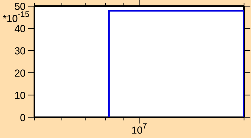
\sigma vs. E for ^{154}\text{Tb}(\text{mt } 34)
