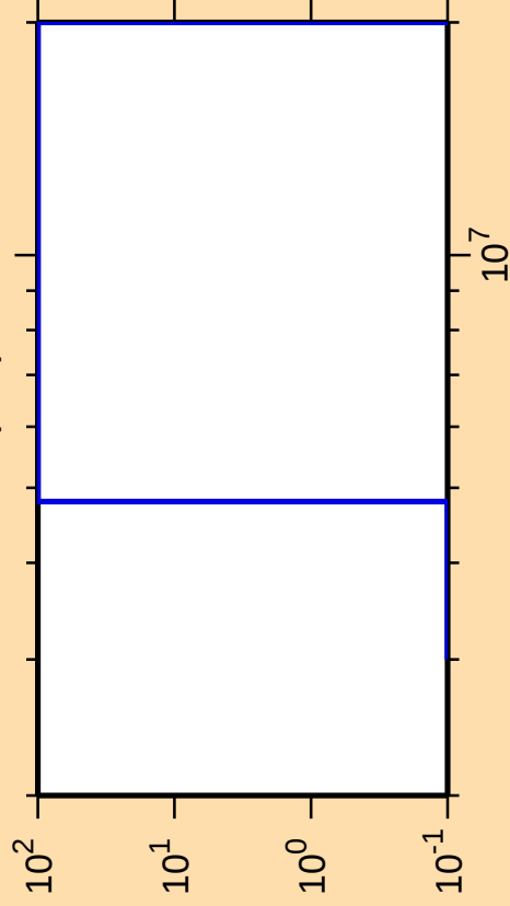
\Delta\sigma/\sigma vs. E for ^{154}\text{Tb}(n,d)
