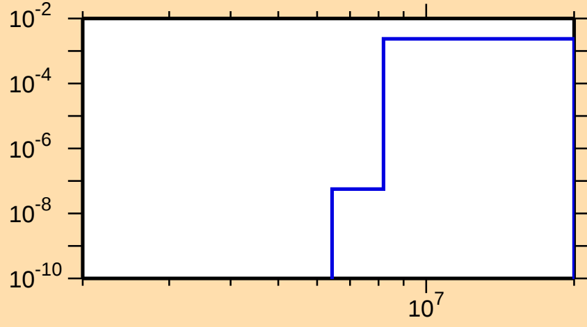
\sigma vs. E for ^{154}\text{Tb}(n,d)
