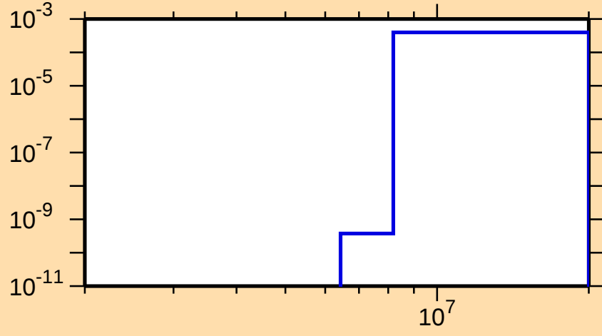
\sigma vs. E for ^{154}\text{Tb}(n,t)
