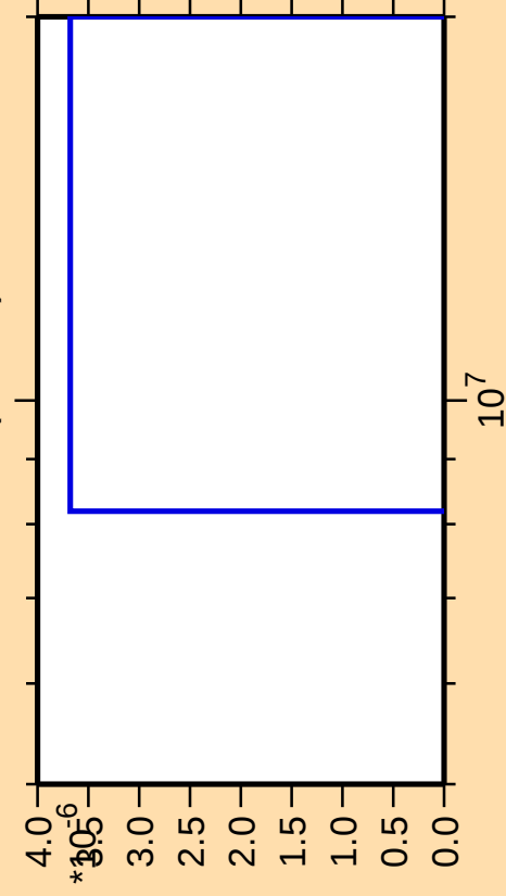
\Delta\sigma/\sigma vs. E for ^{154}\text{Tb}(\text{mt } 42)
