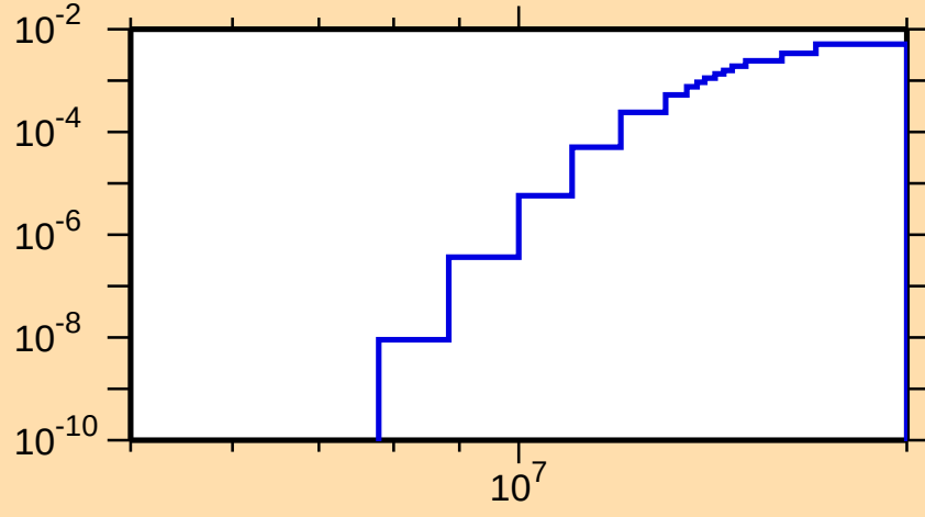
\sigma vs. E for ^{158}\text{Tb}(n,d)
