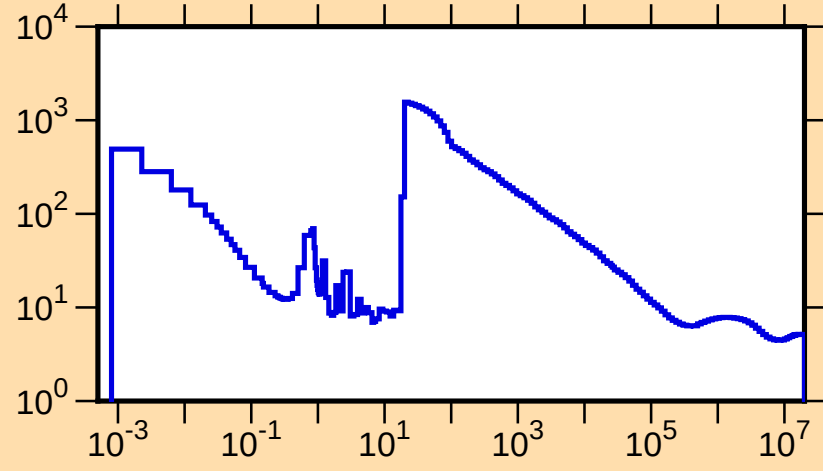
\sigma vs. E for ^{158}\text{Tb}(n,\text{tot.})
