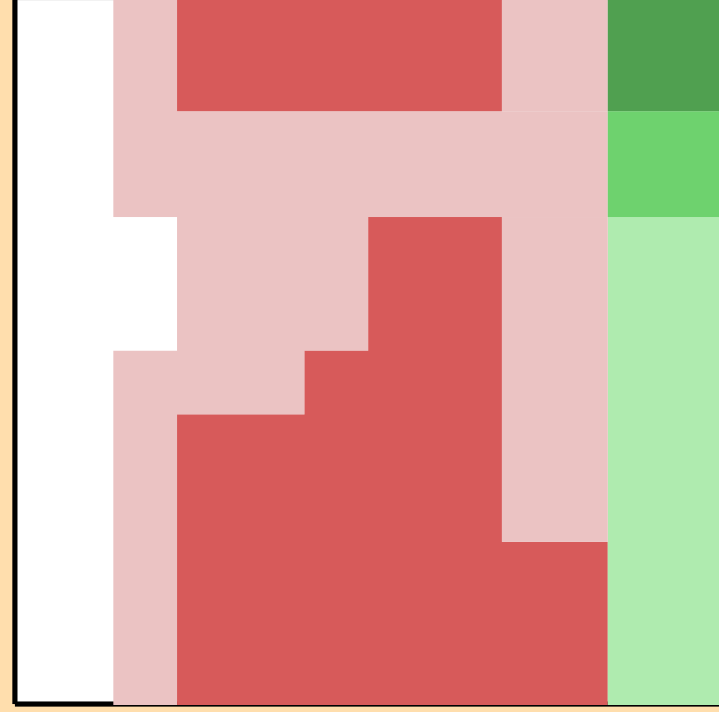
\Delta\sigma/\sigma vs. E for ^{158}\text{Tb}(n,2n)
