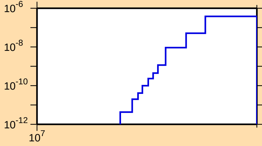
\sigma vs. E for ^{158}\text{Tb}(n,2n\alpha)
