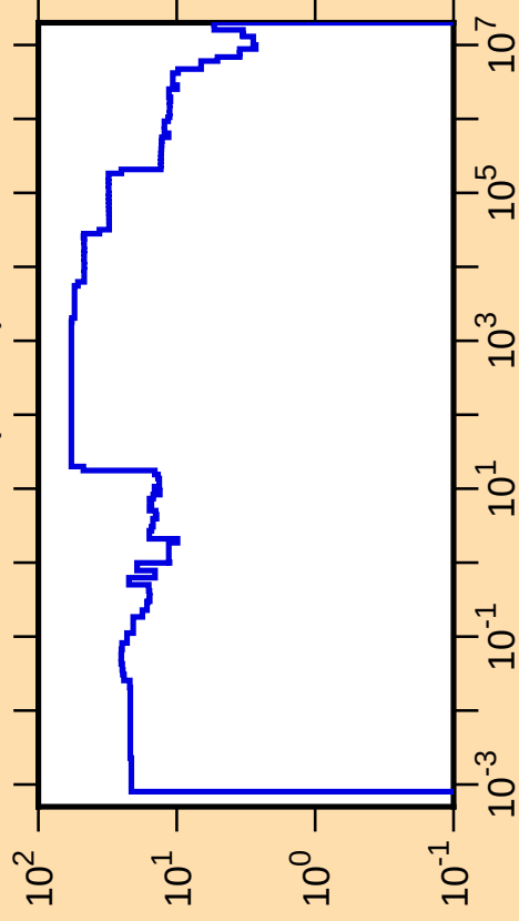
\Delta\sigma/\sigma vs. E for ^{158}\text{Tb}(n,\text{tot.})
