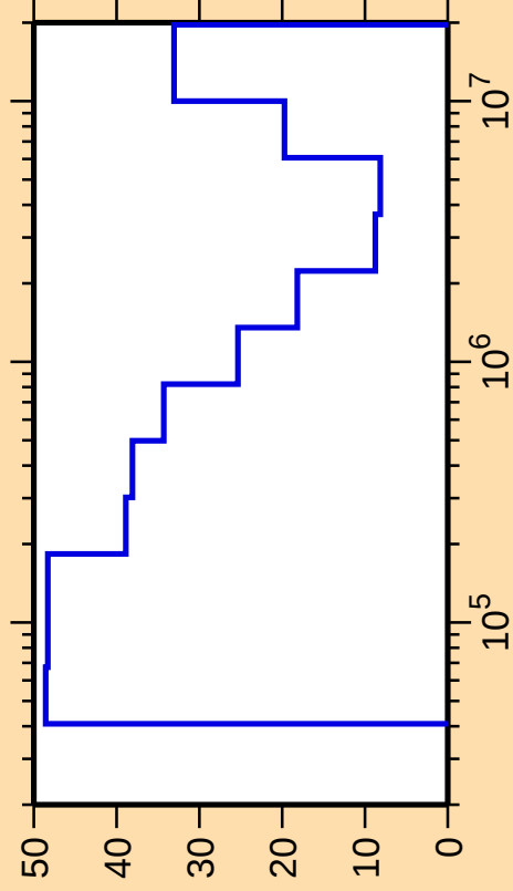
\Delta\sigma/\sigma vs. E for ^{158}\text{Tb}(n,\text{inel.})
