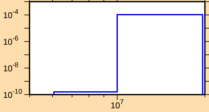
\sigma vs. E for ^{158}\text{Tb}(n,t)
