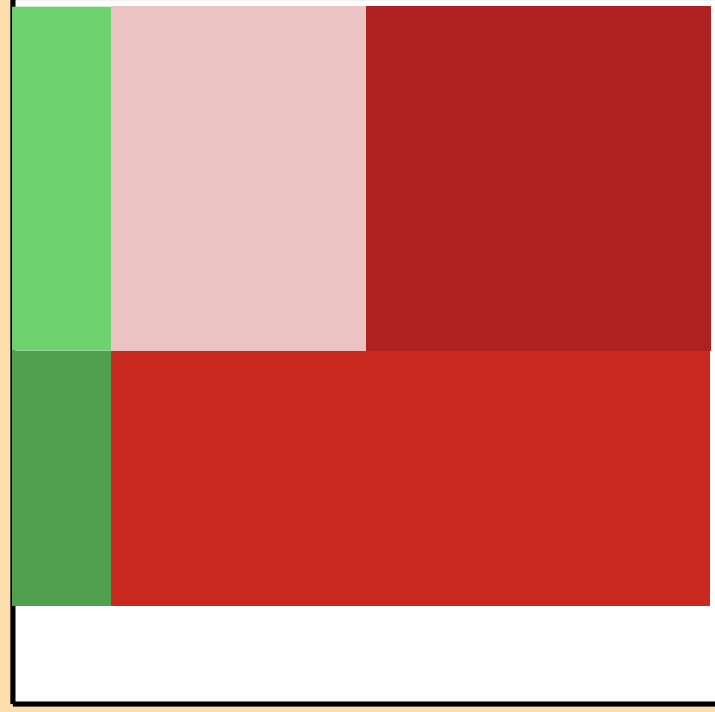
\Delta\sigma/\sigma vs. E for ^{158}\text{Tb}(n,\text{tot.})
