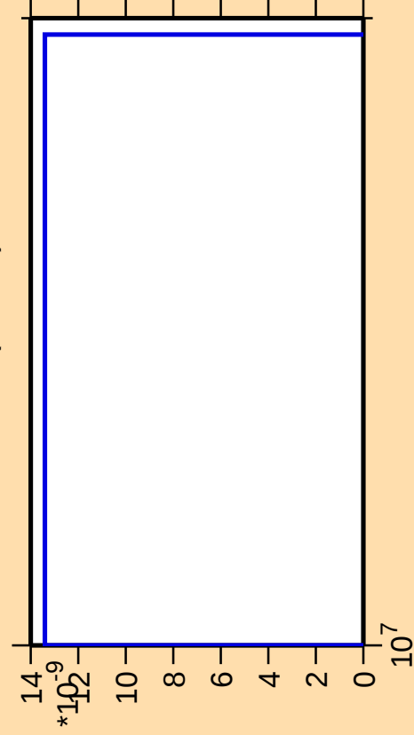
\Delta\sigma/\sigma vs. E for ^{158}\text{Tb}(\text{mt } 11)
