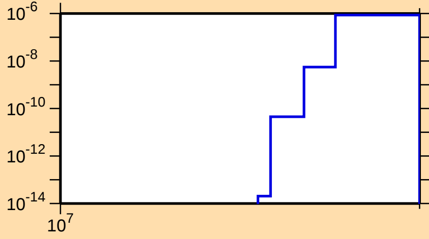
\sigma vs. E for ^{160}\text{Tb}(n,nt)
