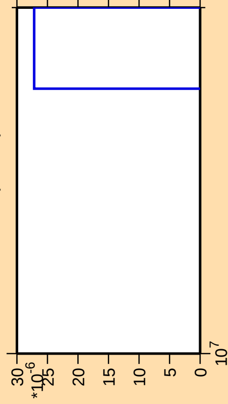
\Delta\sigma/\sigma vs. E for ^{160}\text{Tb}(\text{mt } 11)
