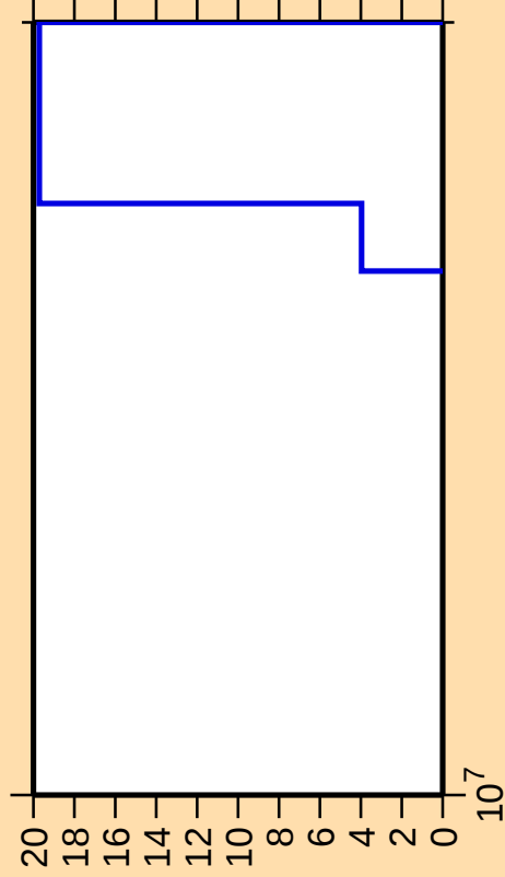
\Delta\sigma/\sigma vs. E for ^{160}\text{Tb}(n,p\alpha)
