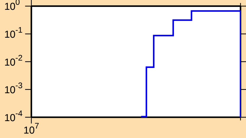
\sigma vs. E for ^{160}\text{Tb}(n,3n)
