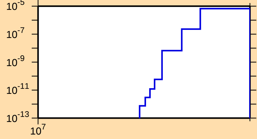
\sigma vs. E for ^{160}\text{Tb}(n,2np)
