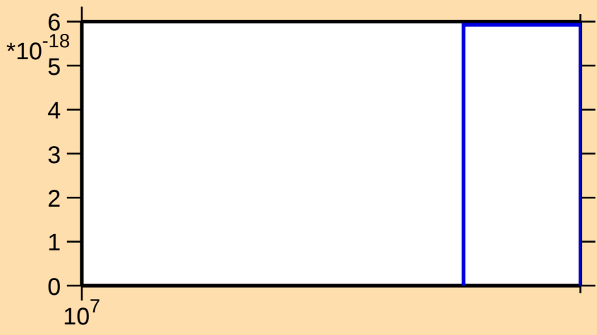
\sigma vs. E for ^{160}\text{Tb}(\text{mt } 11)
