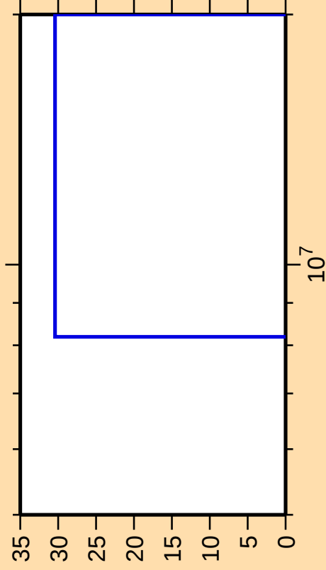
\Delta\sigma/\sigma vs. E for ^{160}\text{Tb}(n,3n)
