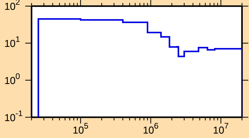
\Delta\sigma/\sigma vs. E for ^{160}\text{Tb}(n,\text{nonel.})
