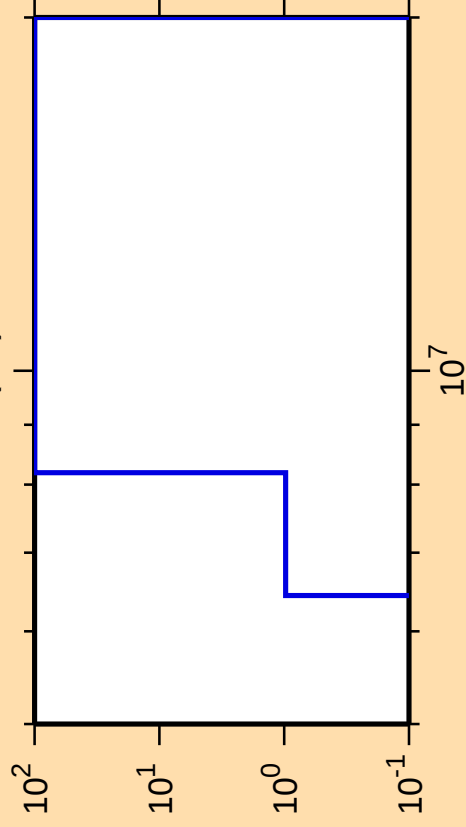
\Delta\sigma/\sigma vs. E for ^{160}\text{Tb}(n,t)
