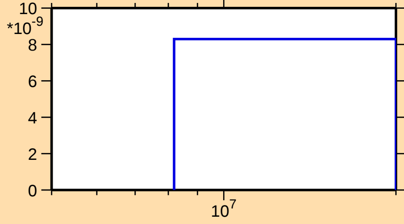
\sigma vs. E for ^{160}\text{Tb}(n,2n\alpha)
