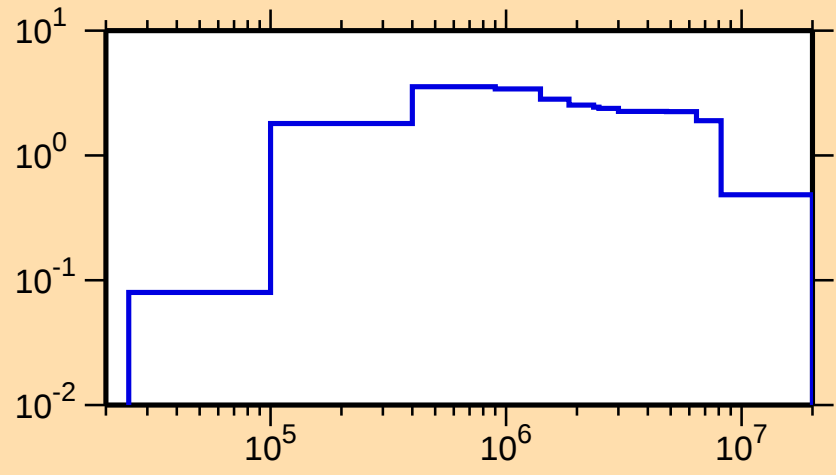
\sigma vs. E for ^{160}\text{Tb}(n,\text{inel.})
