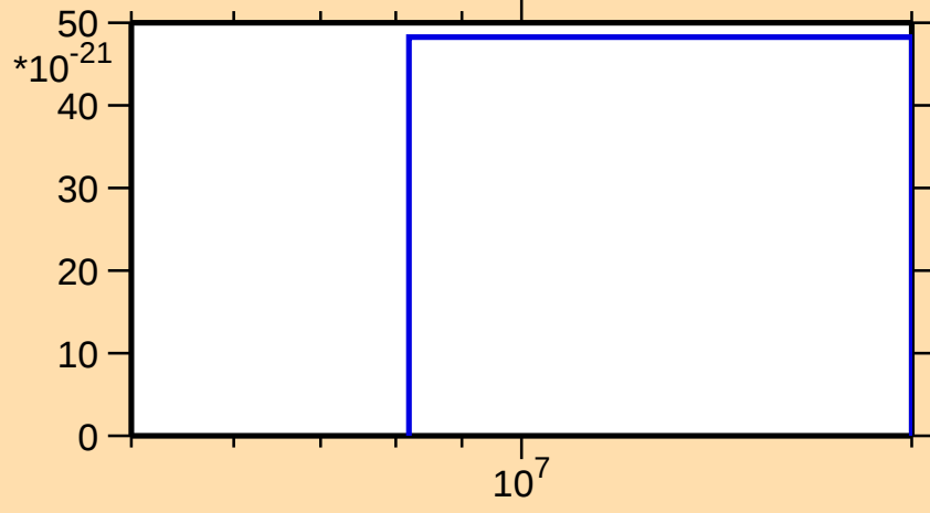
\sigma vs. E for ^{160}\text{Tb}(\text{mt } 11)
