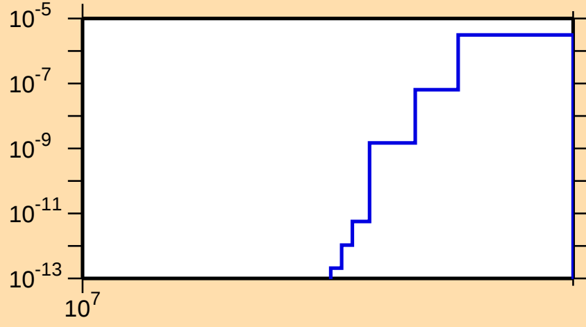
\sigma vs. E for ^{165}\text{Tb}(n,\text{nt})
