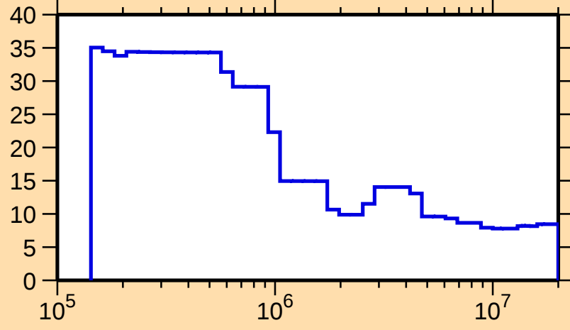
\Delta\sigma/\sigma vs. E for ^{165}\text{Tb}(n,n\text{oncl.})
