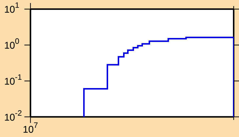
\sigma vs. E for ^{165}\text{Tb}(n,3n)
