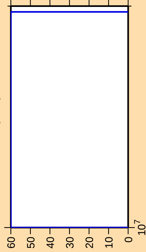
\Delta\sigma/\sigma vs. E for ^{165}\text{Tb}(n,\text{nt})
