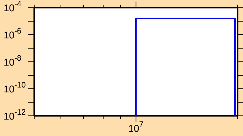
\sigma vs. E for ^{165}\text{Tb}(n,t)
