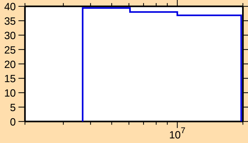
\Delta\sigma/\sigma vs. E for ^{165}\text{Tb}(n,n_1)
