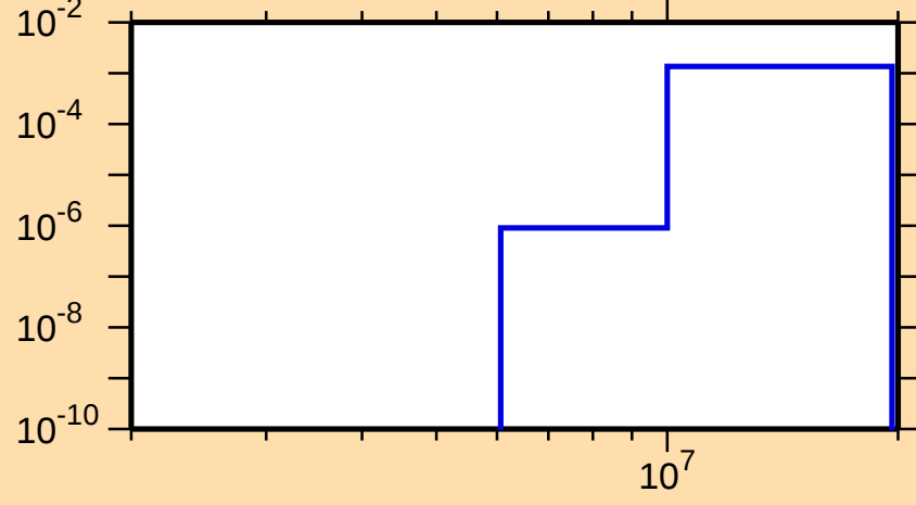
\sigma vs. E for ^{165}\text{Tb}(n,p)
