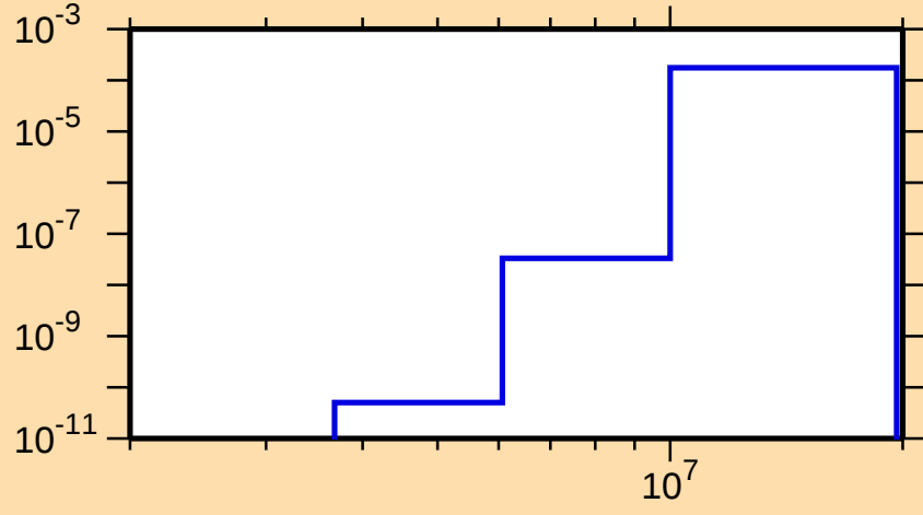
\sigma vs. E for ^{165}\text{Tb}(n,\alpha)
