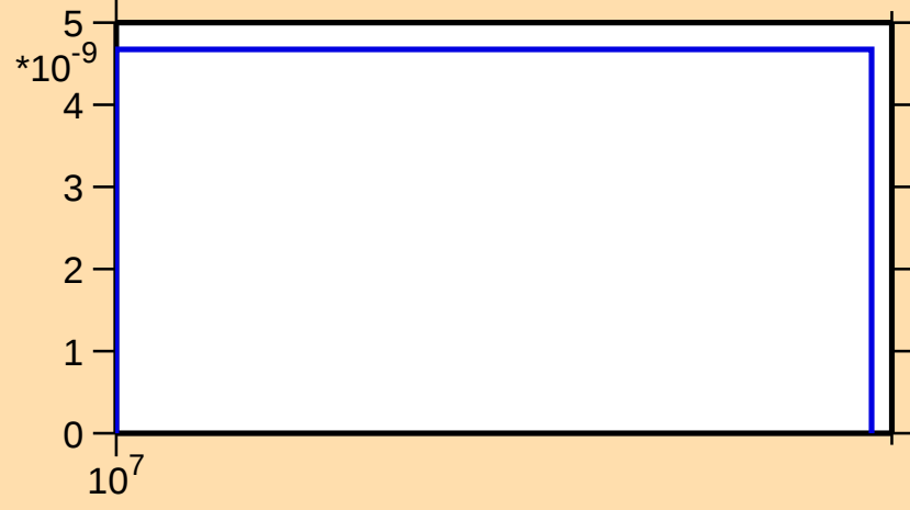
\sigma vs. E for ^{165}\text{Tb}(n,\text{nd})
