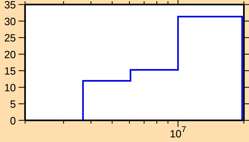
\Delta\sigma/\sigma vs. E for ^{165}\text{Tb}(n,n\text{cont.})
