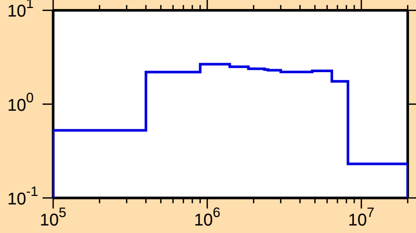
\sigma vs. E for ^{165}\text{Tb}(n,\text{inel.})
