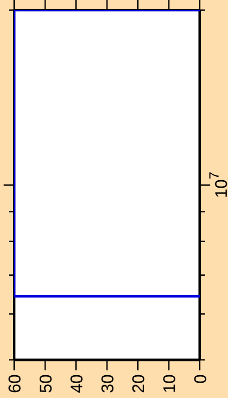
\Delta\sigma/\sigma vs. E for ^{165}\text{Tb}(n,\alpha)
