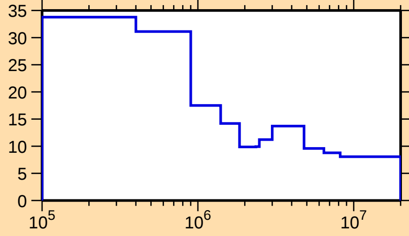
\Delta\sigma/\sigma vs. E for ^{165}\text{Tb}(n,n\text{onel.})
