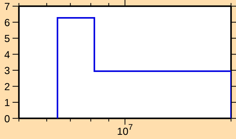
\Delta\sigma/\sigma vs. E for ^{165}\text{Tb}(n,\text{tot.})
