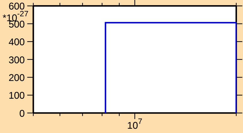
\sigma vs. E for ^{165}\text{Tb}(\text{mt } 42)
