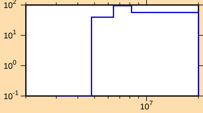
\Delta\sigma/\sigma vs. E for ^{165}\text{Tb}(n,p)
