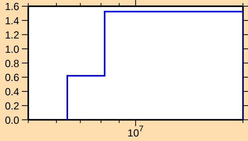
\sigma vs. E for ^{165}\text{Tb}(n,2n)
