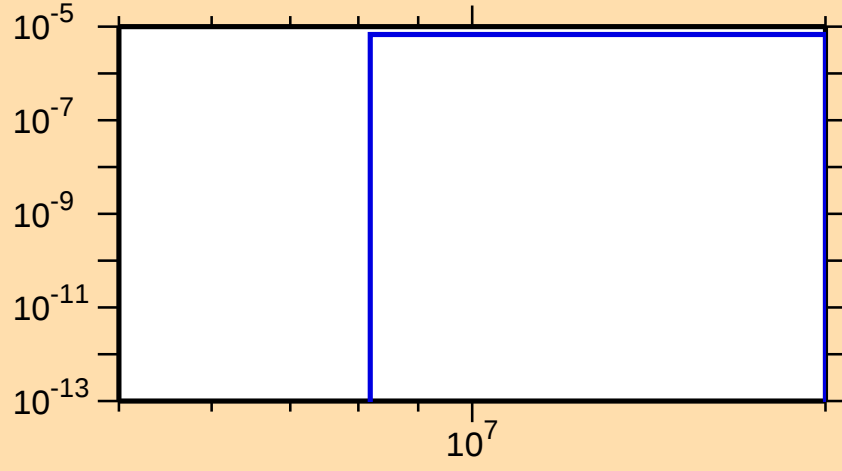
\sigma vs. E for ^{165}\text{Tb}(n,n\alpha)
