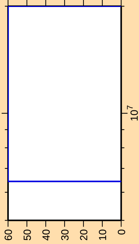
\Delta\sigma/\sigma vs. E for ^{165}\text{Tb}(n,\gamma)
