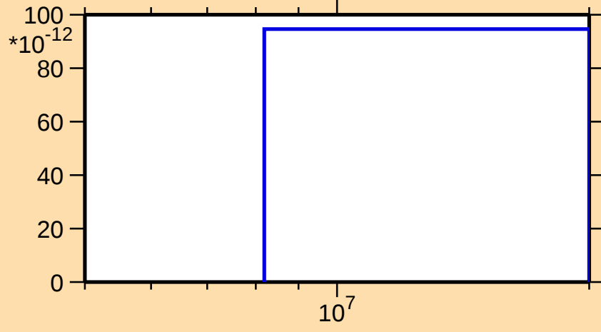
\sigma vs. E for ^{165}\text{Tb}(n,2n\alpha)
