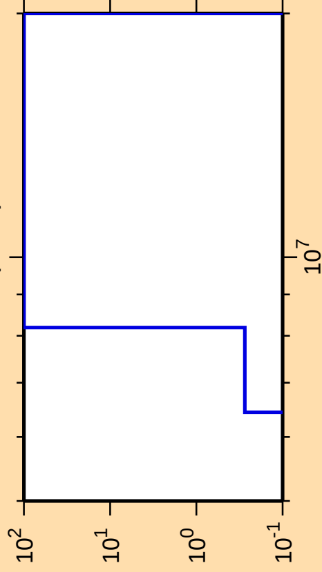
\Delta\sigma/\sigma vs. E for ^{165}\text{Tb}(n,n\alpha)
