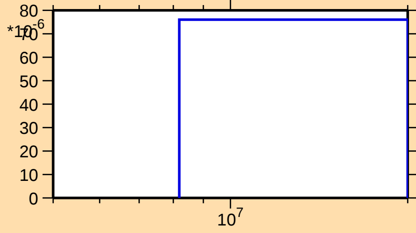
\sigma vs. E for ^{165}\text{Tb}(n,d)
