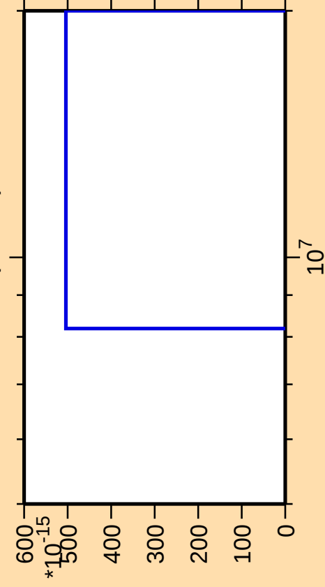
\Delta\sigma/\sigma vs. E for ^{165}\text{Tb}(\text{mt } 42)
