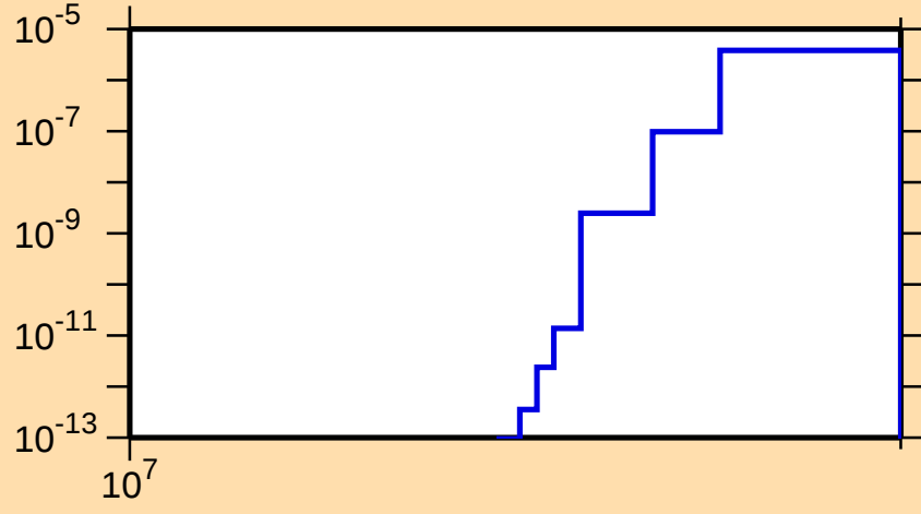
\sigma vs. E for ^{167}\text{Tb}(n,nt)
