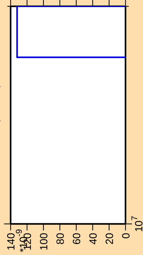
\Delta\sigma/\sigma vs. E for ^{167}\text{Tb} (mt 42)
