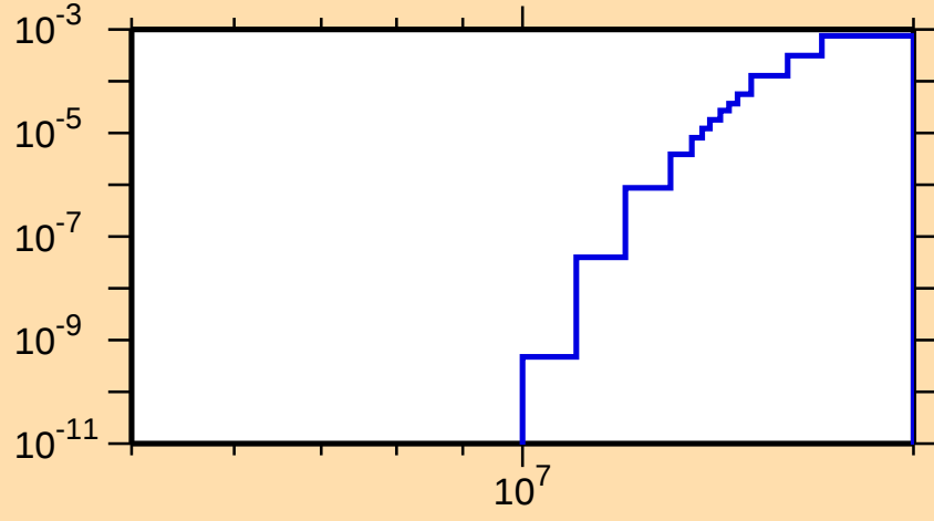
\sigma vs. E for ^{167}\text{Tb}(n,d)
