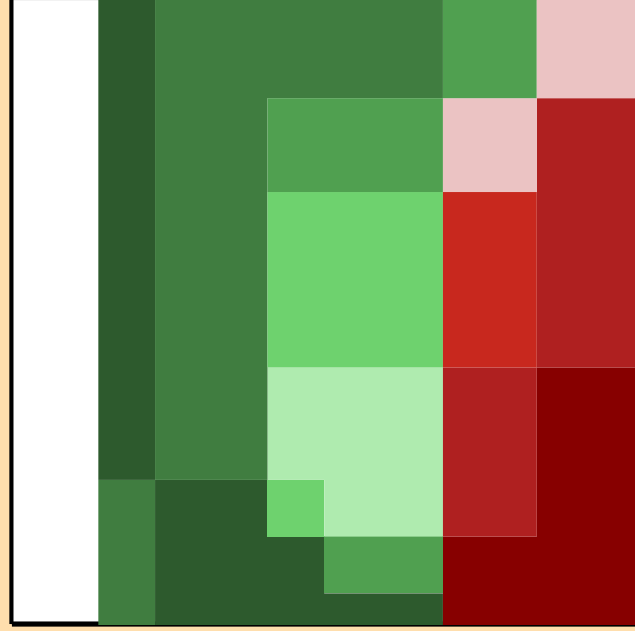
\Delta\sigma/\sigma vs. E for ^{167}\text{Tb}(n,p)
