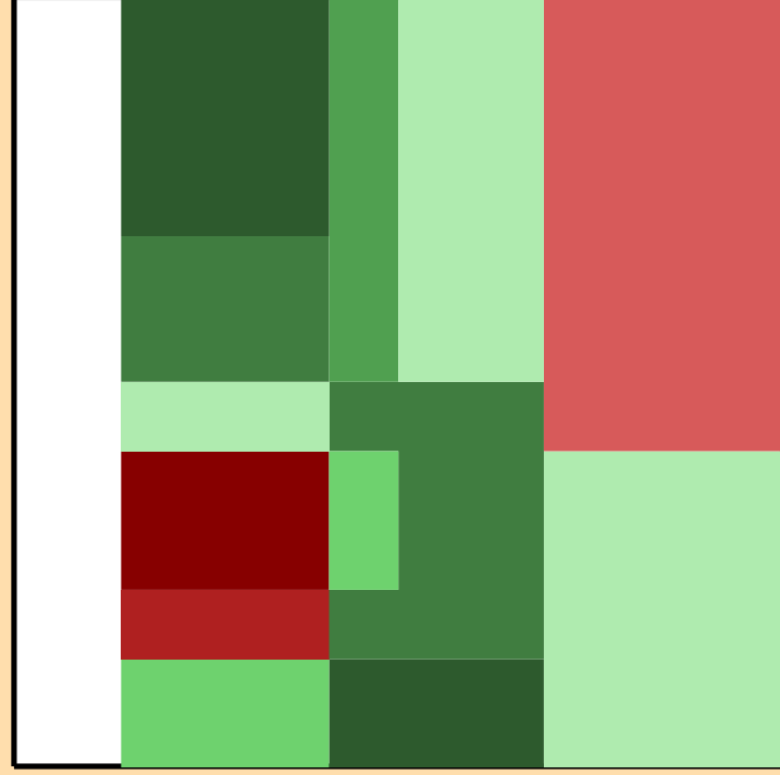
\Delta\sigma/\sigma vs. E for ^{167}\text{Tb}(n,2n)
