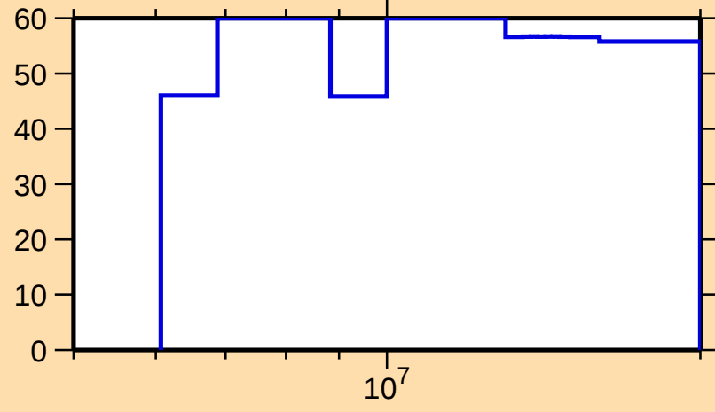
\Delta\sigma/\sigma vs. E for ^{167}\text{Tb}(n,ncont.)
