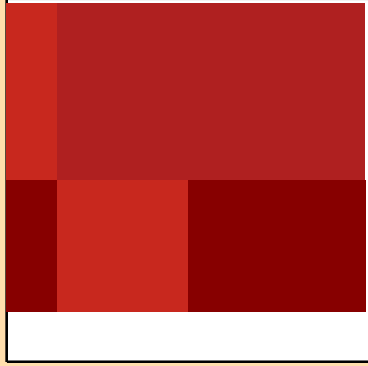
\Delta\sigma/\sigma vs. E for ^{167}\text{Tb}(n,\text{tot.})
