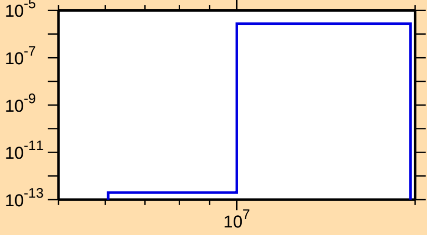
\sigma vs. E for ^{167}\text{Tb}(n,n\alpha)
