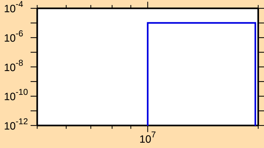
\sigma vs. E for ^{167}\text{Tb}(n,t)
