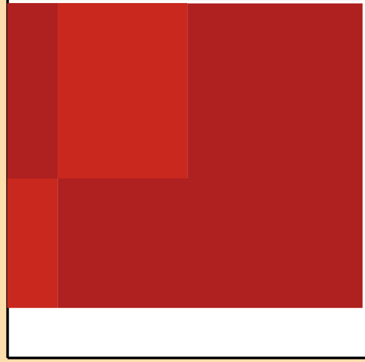
\Delta\sigma/\sigma vs. E for ^{167}\text{Tb}(n,n_1)
