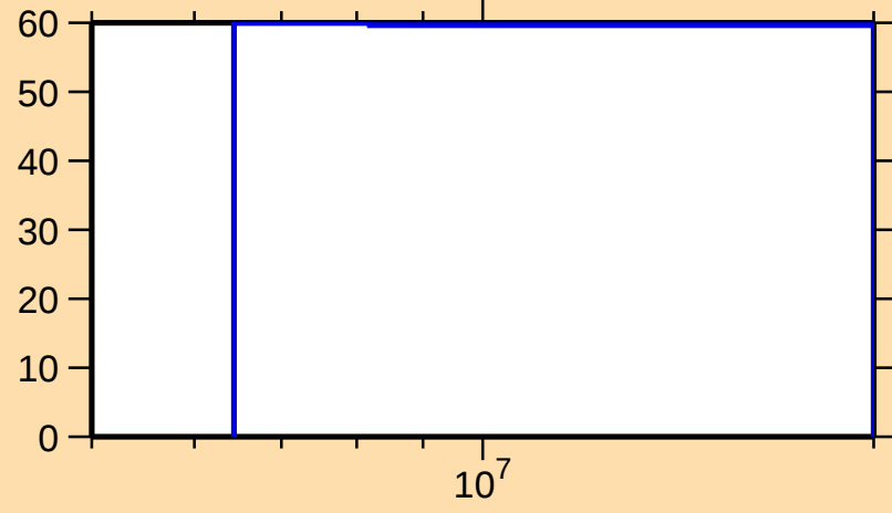
\Delta\sigma/\sigma vs. E for ^{167}\text{Tb}(n,n_1)
