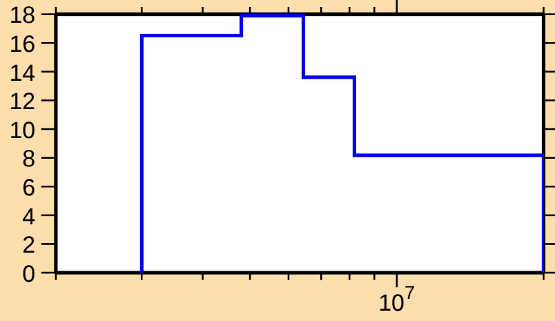
\Delta\sigma/\sigma vs. E for ^{167}\text{Tb}(n,\text{nonel.})
