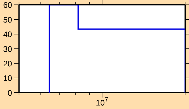
\Delta\sigma/\sigma vs. E for ^{167}\text{Tb}(n,n\text{cont.})
