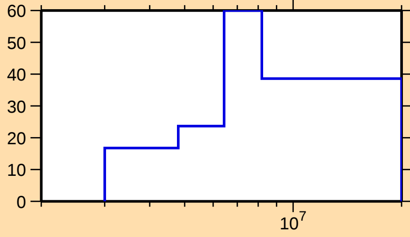
\Delta\sigma/\sigma vs. E for ^{167}\text{Tb}(n,\text{inel.})
