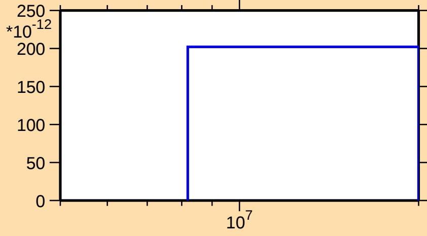
\sigma vs. E for ^{167}\text{Tb}(n,2np)
