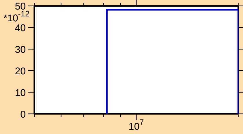
\sigma vs. E for ^{167}\text{Tb}(n,2n\alpha)
