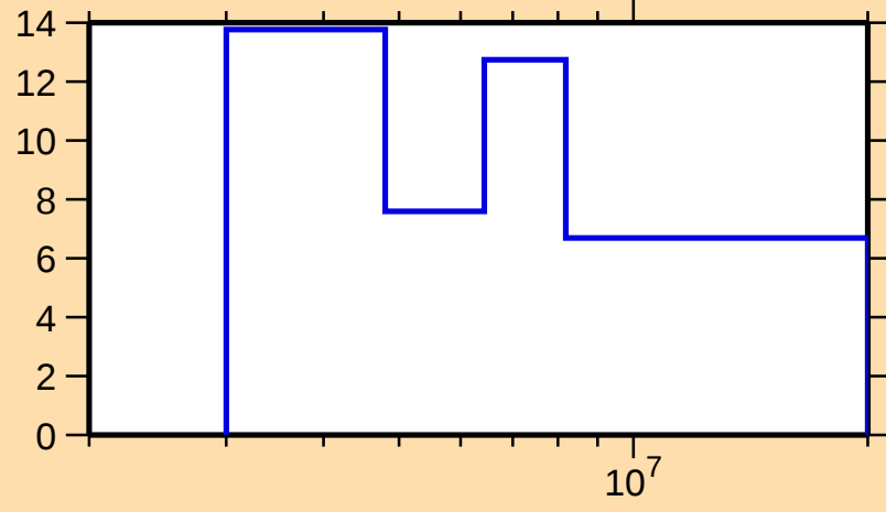
\Delta\sigma/\sigma vs. E for ^{167}\text{Tb}(n,\text{tot.})
