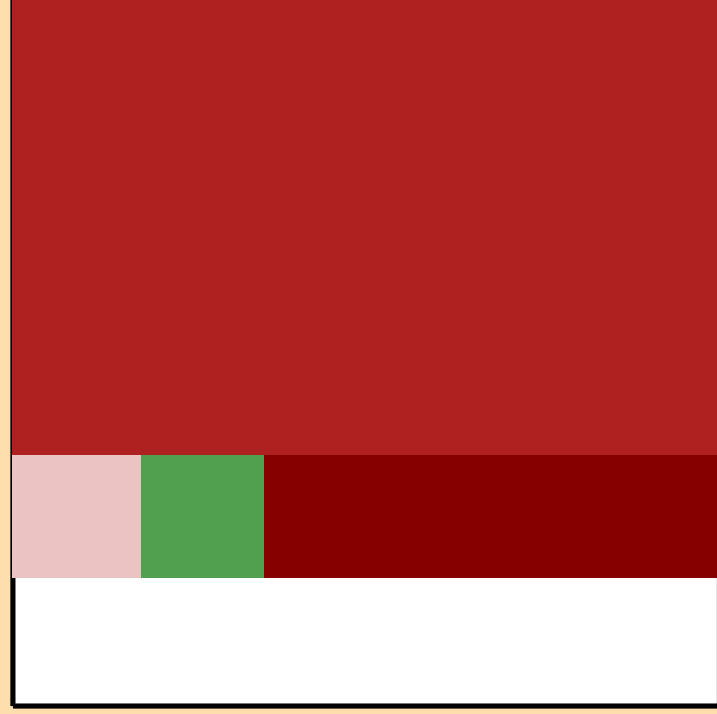
\Delta\sigma/\sigma vs. E for ^{167}\text{Tb}(n,\text{el.})
