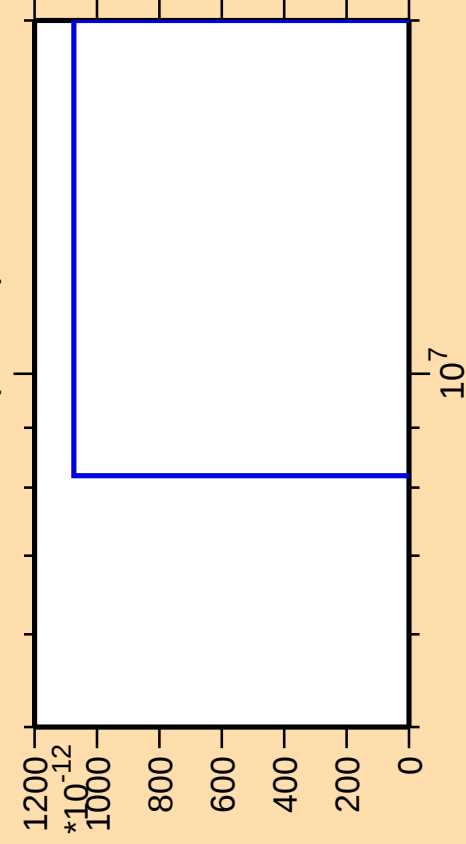
\Delta\sigma/\sigma vs. E for ^{167}\text{Tb}(\text{mt } 42)
