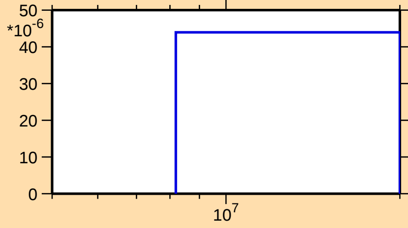
\sigma vs. E for ^{167}\text{Tb}(n,d)
