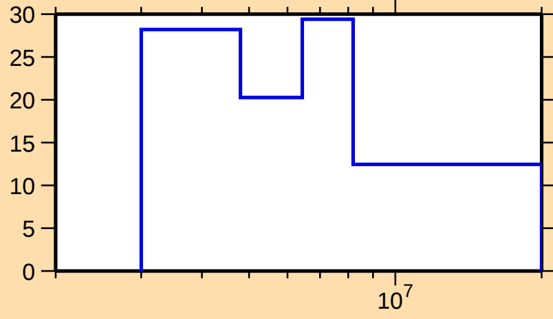
\Delta\sigma/\sigma vs. E for ^{167}\text{Tb}(n,\text{el.})
