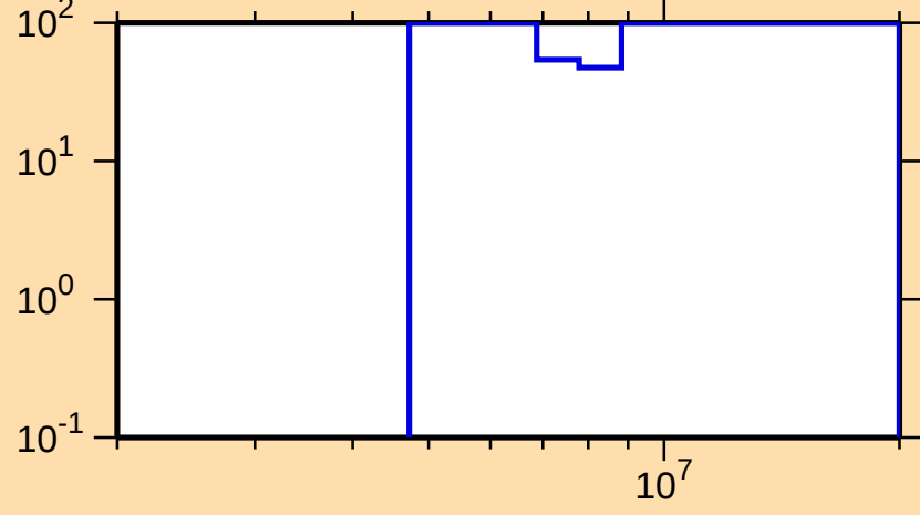
\Delta\sigma/\sigma vs. E for ^{168}\text{Tb}(n,\gamma)
