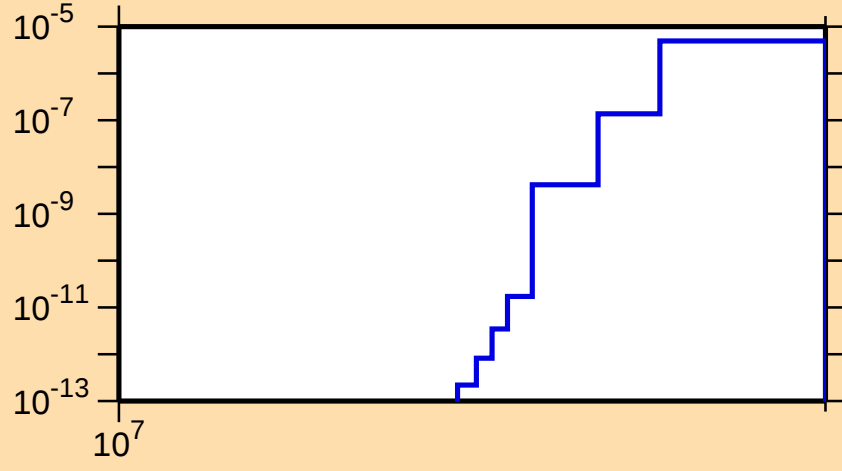
\sigma vs. E for ^{168}\text{Tb}(n,nt)
