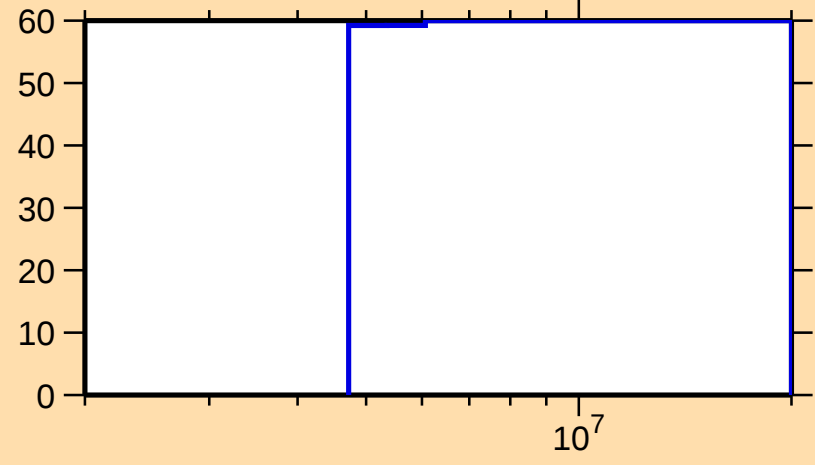
\Delta\sigma/\sigma vs. E for ^{168}\text{Tb}(n,ncont.)
