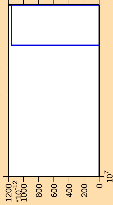
\Delta\sigma/\sigma vs. E for ^{168}\text{Tb}(\text{mt } 42)
