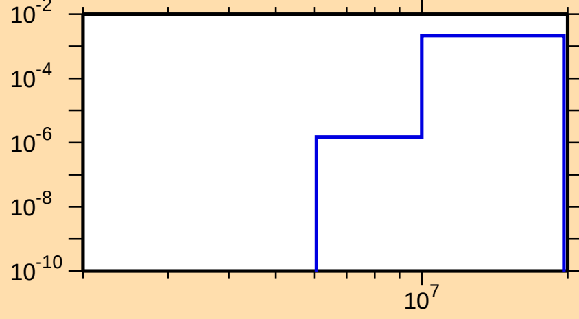
\sigma vs. E for ^{168}\text{Tb}(n,p)
