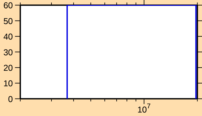
\Delta\sigma/\sigma vs. E for ^{168}\text{Tb}(n,\gamma)
