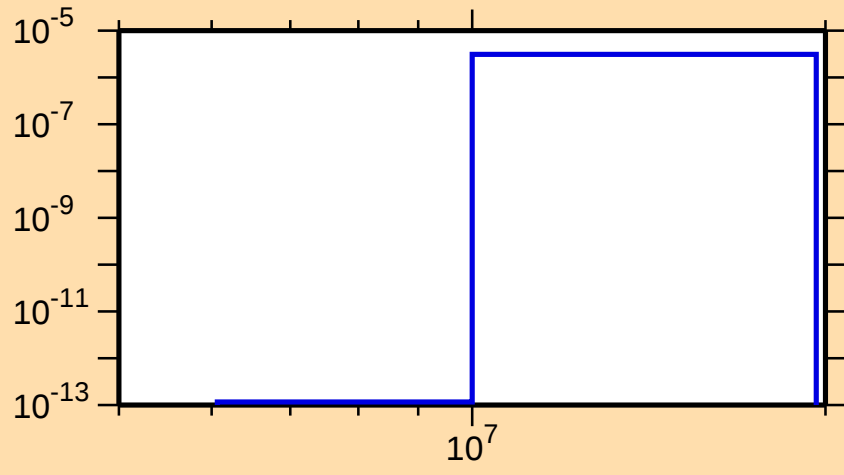
\sigma vs. E for ^{168}\text{Tb}(n,n\alpha)
