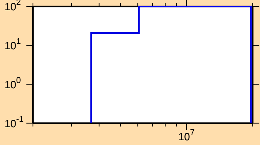
\Delta\sigma/\sigma vs. E for ^{168}\text{Tb}(n,ncont.)
