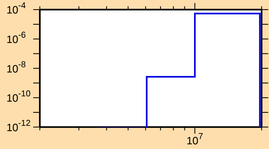
\sigma vs. E for ^{168}\text{Tb}(n,\alpha)
