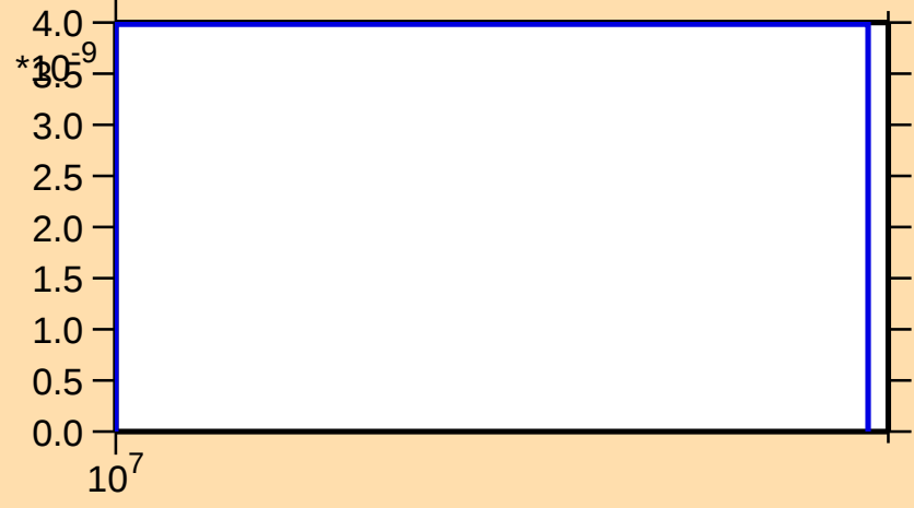
\sigma vs. E for ^{168}\text{Tb}(n,2np)
