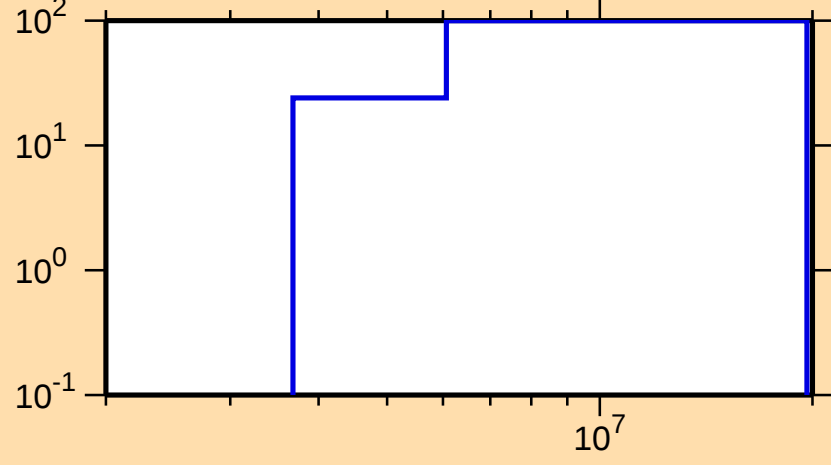
\Delta\sigma/\sigma vs. E for ^{168}\text{Tb}(n,\text{inel.})
