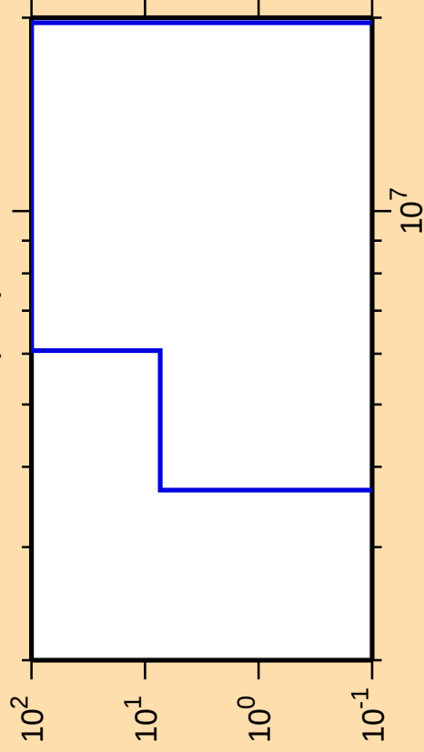
\Delta\sigma/\sigma vs. E for ^{168}\text{Tb}(n,\alpha)
