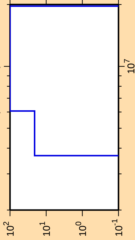
\Delta\sigma/\sigma vs. E for ^{168}\text{Tb}(n,n\text{cont.})
