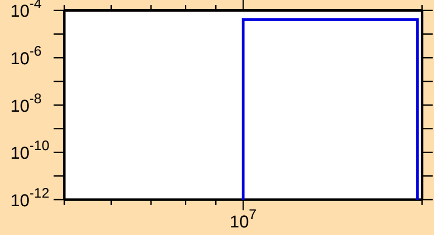
\sigma vs. E for ^{168}\text{Tb}(n,d)
