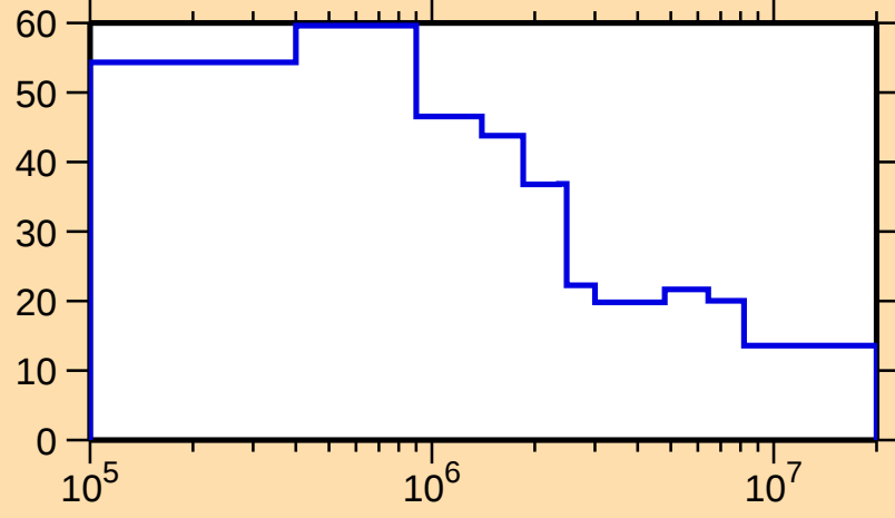
\Delta\sigma/\sigma vs. E for ^{168}\text{Tb}(n,n\text{onel.})
