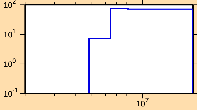
\Delta\sigma/\sigma vs. E for ^{168}\text{Tb}(n,p)
