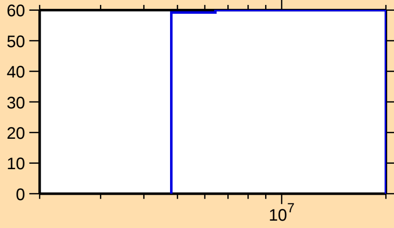
\Delta\sigma/\sigma vs. E for ^{168}\text{Tb}(n,n\text{cont.})
