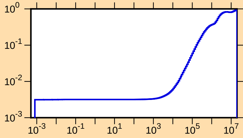
\mu vs. E for ^{215}\text{Th}(\text{mt251})
