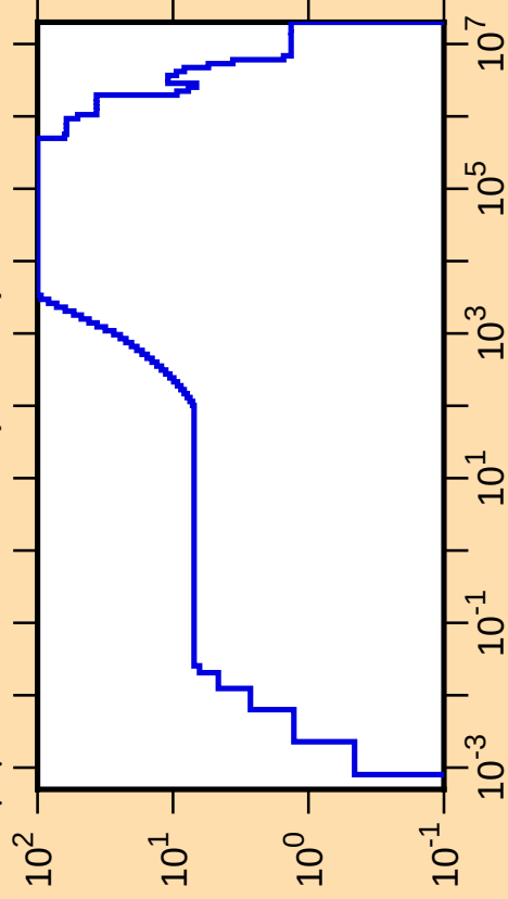
\Delta\mu/\mu vs. E for ^{215}\text{Th}(\text{mt251})
