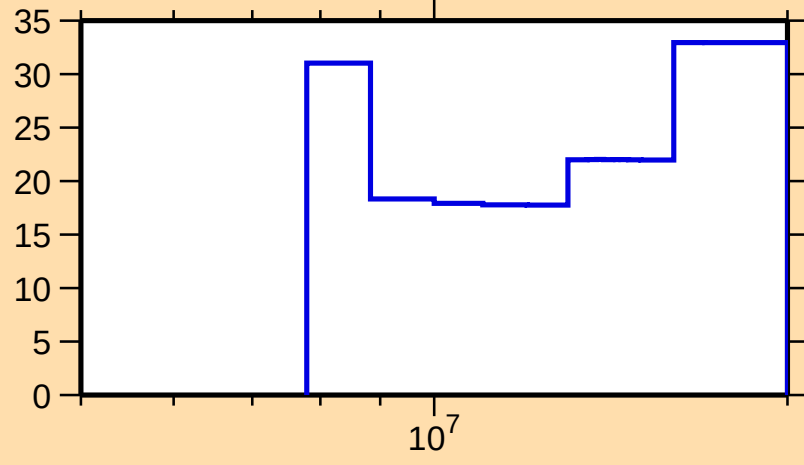
\Delta\sigma/\sigma vs. E for ^{215}\text{Th}(n,2n)
