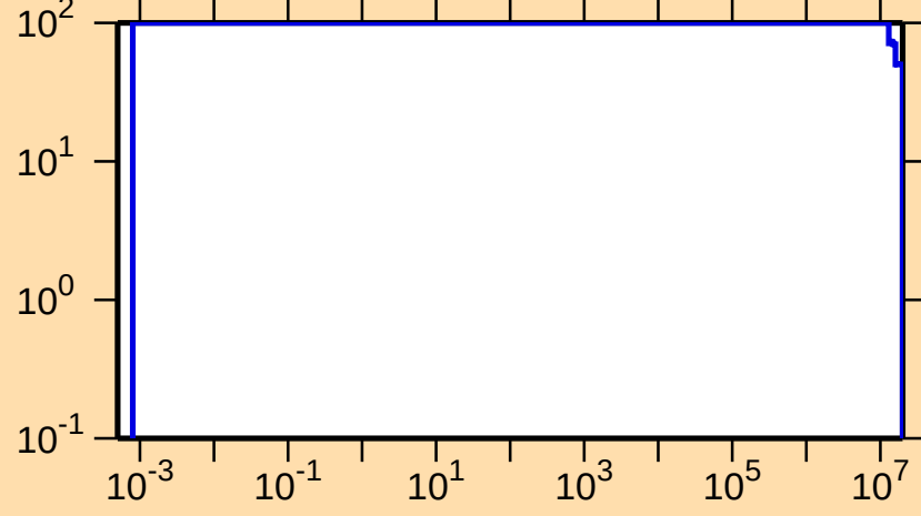
\Delta\sigma/\sigma vs. E for ^{215}\text{Th}(n,p)
