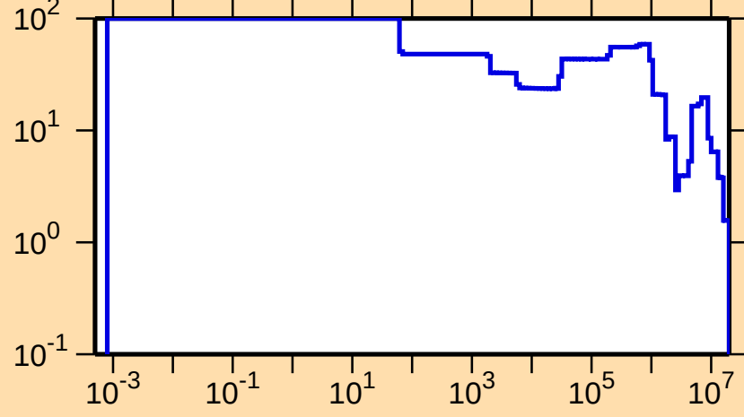
\Delta\sigma/\sigma vs. E for ^{215}\text{Th}(n,\text{el.})
