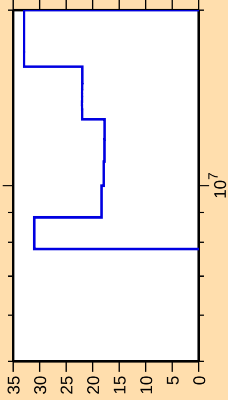
\Delta\sigma/\sigma vs. E for ^{215}\text{Th}(n,2n)
