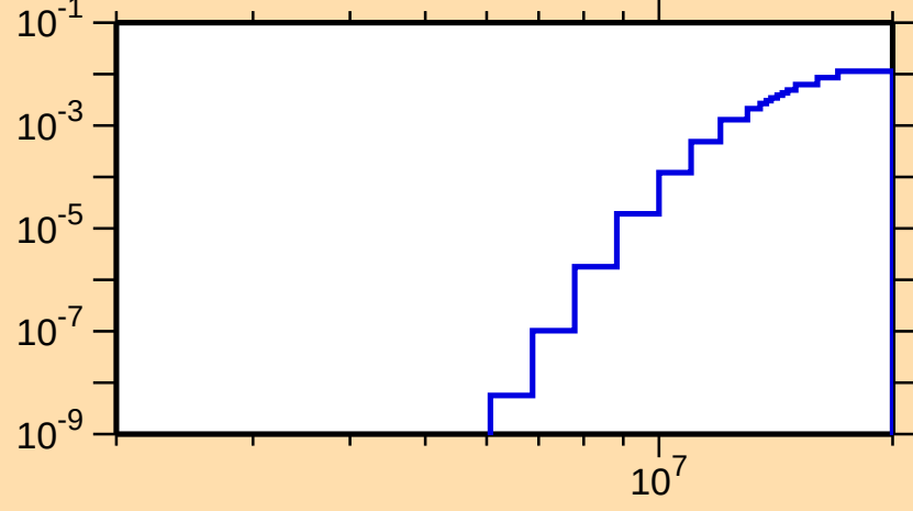
\sigma vs. E for ^{215}\text{Th}(n,d)
