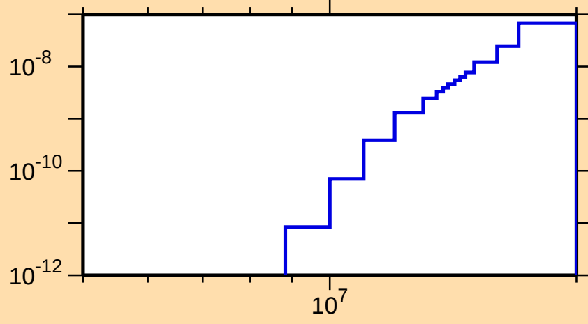
\sigma vs. E for ^{215}\text{Th}(\text{mt117})
