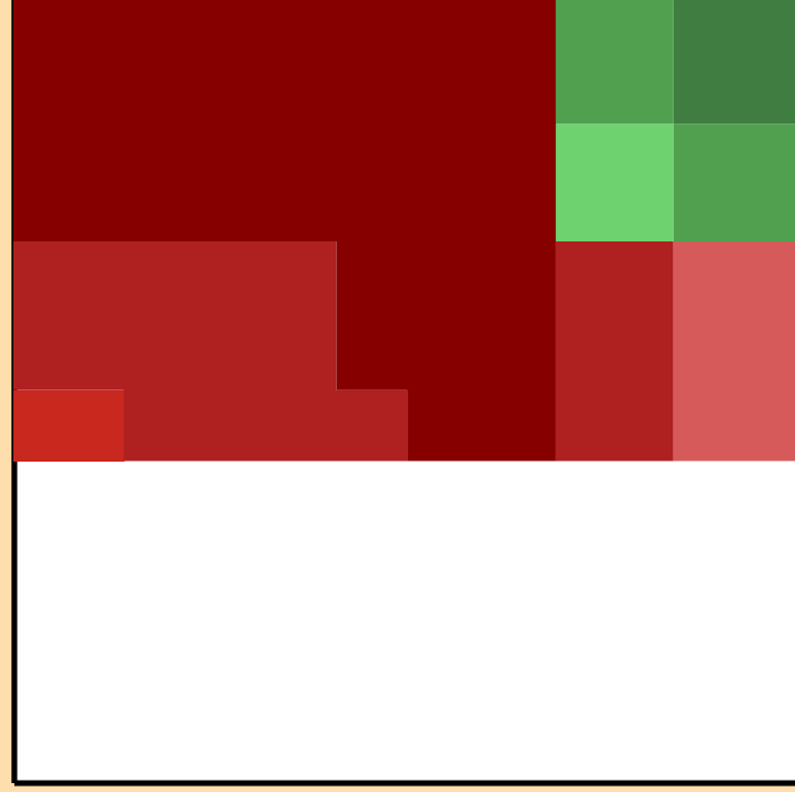
\Delta\sigma/\sigma vs. E for ^{215}\text{Th}(n,\text{el.})
