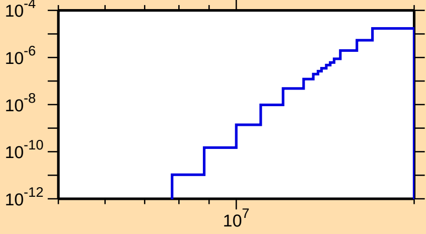
\sigma vs. E for ^{215}\text{Th}(n,\text{He3})
