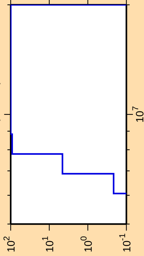
\Delta\sigma/\sigma vs. E for ^{215}\text{Th}(n,\text{He3})
