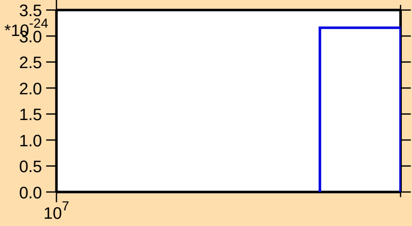
\sigma vs. E for ^{215}\text{Th}(\text{mt } 42)
