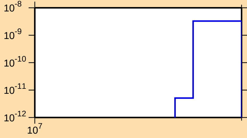
\sigma vs. E for ^{215}\text{Th}(n,\text{nt})
