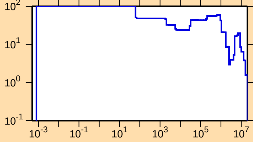
\Delta\sigma/\sigma vs. E for ^{215}\text{Th}(n,\text{el.})
