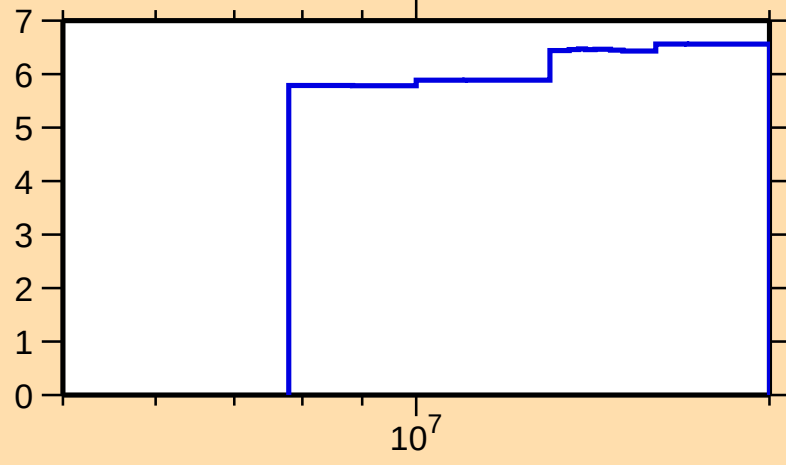
\Delta\sigma/\sigma vs. E for ^{215}\text{Th}(n,\text{nonel.})
