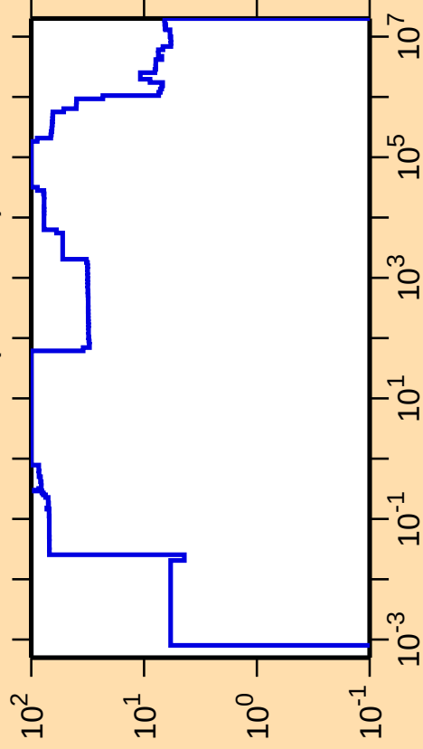
\Delta\sigma/\sigma vs. E for ^{215}\text{Th}(n,\text{nonel.})
