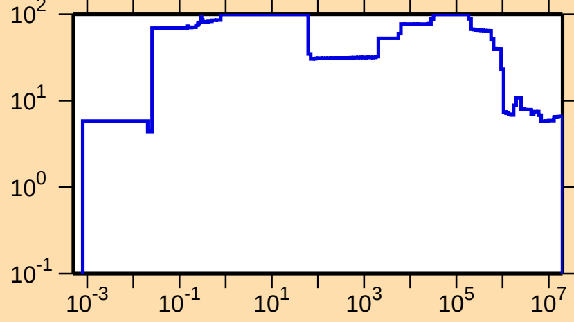
\Delta\sigma/\sigma vs. E for ^{215}\text{Th}(n,\text{nonel.})
