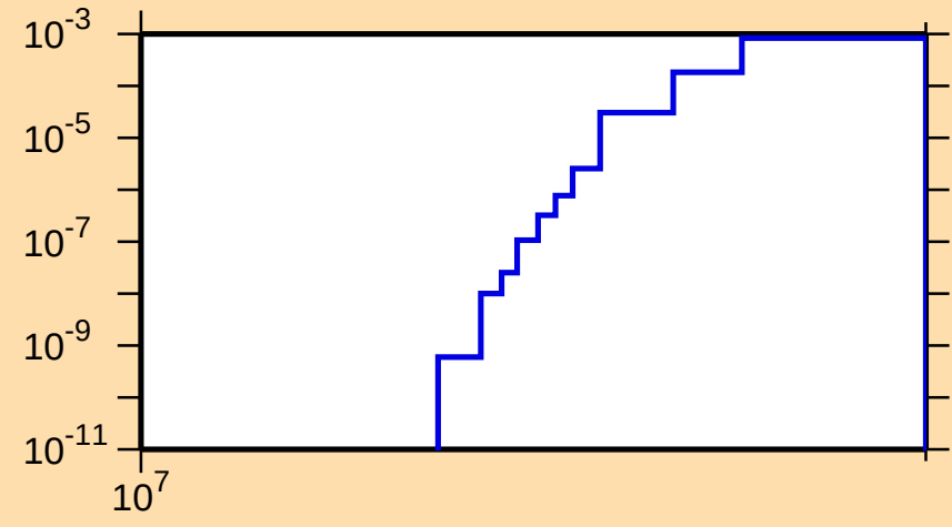
\sigma vs. E for ^{215}\text{Th}(n,2np)
