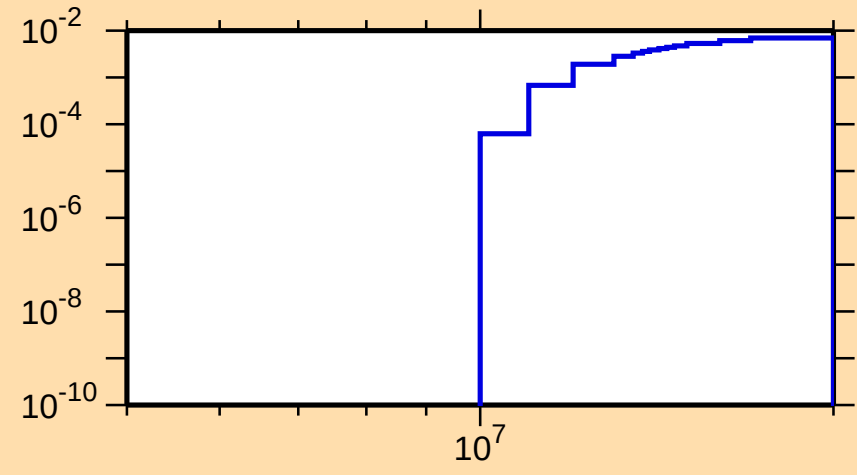
\sigma vs. E for ^{215}\text{Th}(n,2n\alpha)
