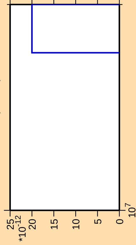
\Delta\sigma/\sigma vs. E for ^{215}\text{Th}(\text{mt } 42)
