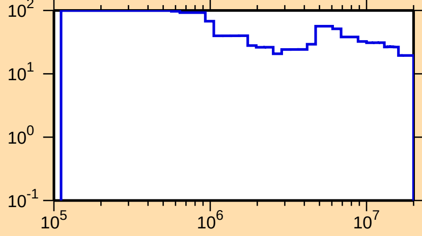
\Delta\sigma/\sigma vs. E for ^{215}\text{Th}(n,n_1)
