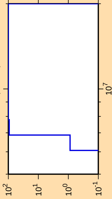
\Delta\sigma/\sigma vs. E for ^{215}\text{Th}(\text{mt } 45)
