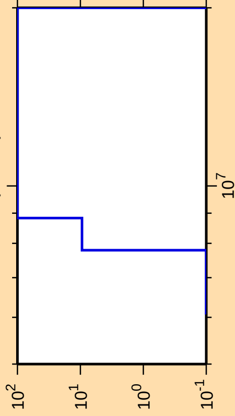
\Delta\sigma/\sigma vs. E for ^{215}\text{Th}(n,2n\alpha)
