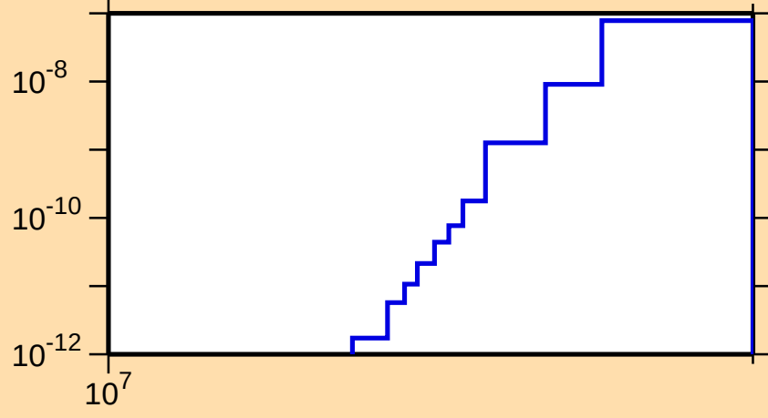
\sigma vs. E for ^{215}\text{Th}(n,\text{pt})
