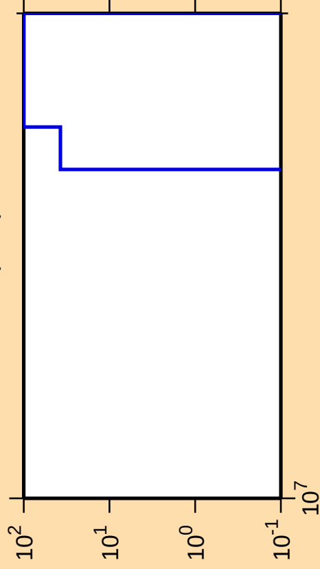
\Delta\sigma/\sigma vs. E for ^{215}\text{Th}(n,\text{nt})
