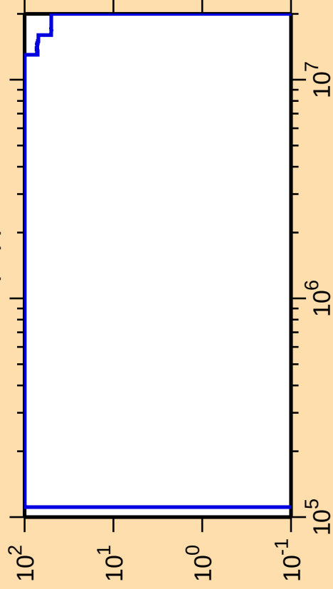
\Delta\sigma/\sigma vs. E for ^{215}\text{Th}(n,p)
