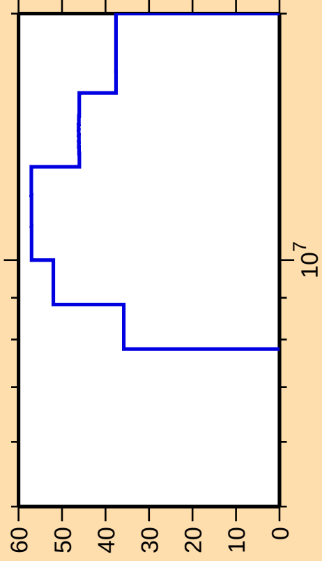
\Delta\sigma/\sigma vs. E for ^{215}\text{Th}(n,n\text{cont.})
