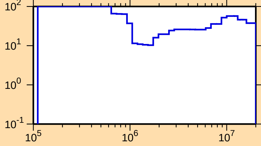
\Delta\sigma/\sigma vs. E for ^{215}\text{Th}(n,n\text{cont.})
