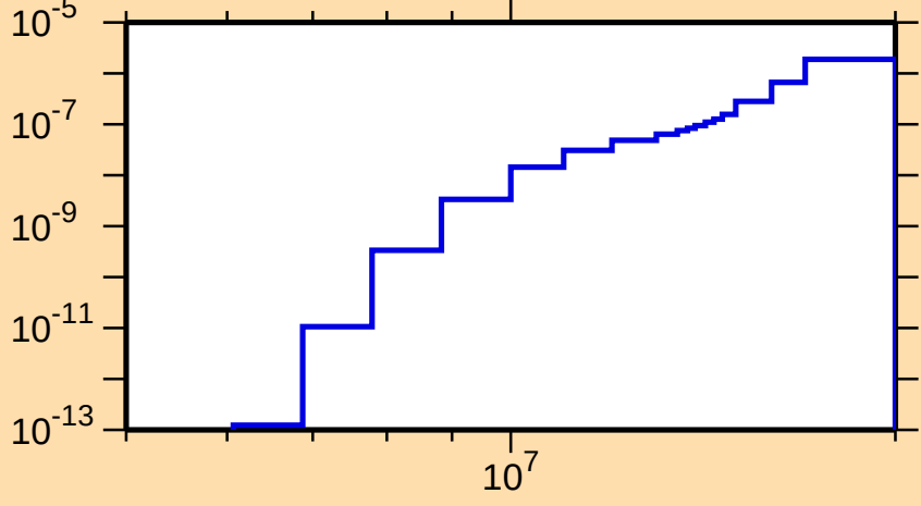
\sigma vs. E for ^{215}\text{Th}(\text{mt } 45)
