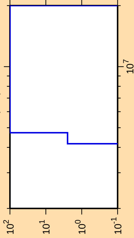
\Delta\sigma/\sigma vs. E for ^{215}\text{Th}(n,d)
