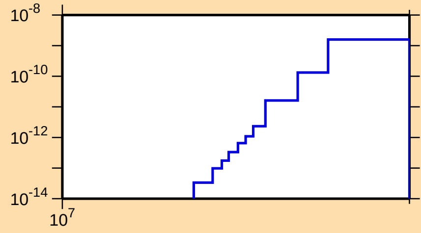
\sigma vs. E for ^{215}\text{Th}(\text{mt } 34)
