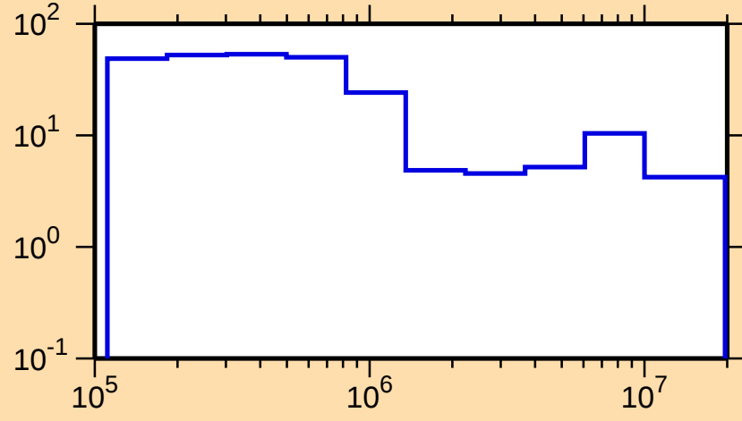
\Delta\sigma/\sigma vs. E for ^{215}\text{Th}(n,\text{tot.})
