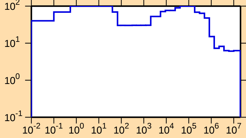
\Delta\sigma/\sigma vs. E for ^{215}\text{Th}(n,\text{nonel.})
