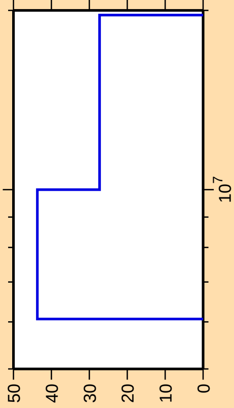
\Delta\sigma/\sigma vs. E for ^{215}\text{Th}(n,n_1)
