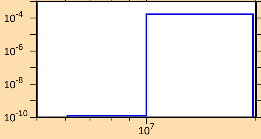
\sigma vs. E for ^{215}\text{Th}(n,t)
