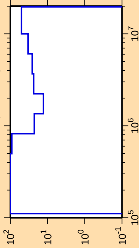
\Delta\sigma/\sigma vs. E for ^{215}\text{Th}(n,\text{ncont.})
