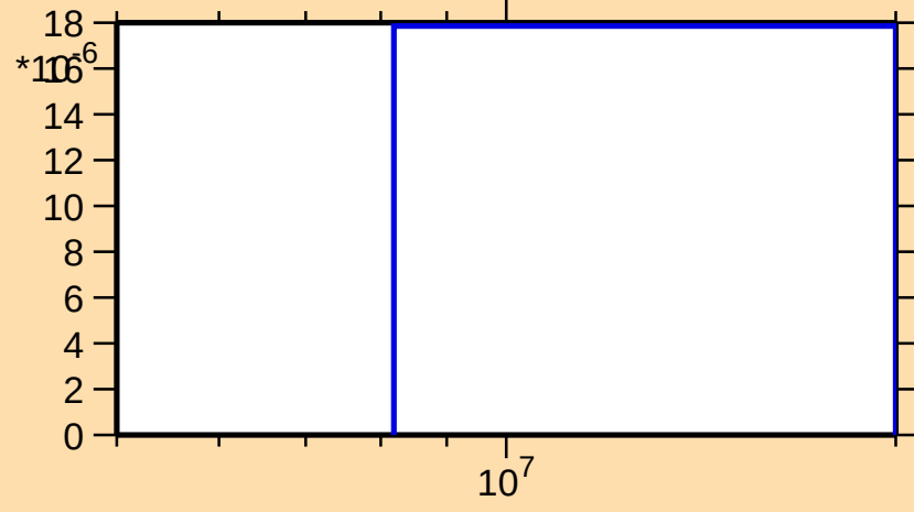
\sigma vs. E for ^{215}\text{Th}(n,2np)
