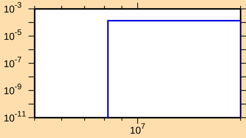
\sigma vs. E for ^{215}\text{Th}(n,t)
