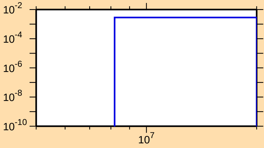
\sigma vs. E for ^{215}\text{Th}(n,2n\alpha)
