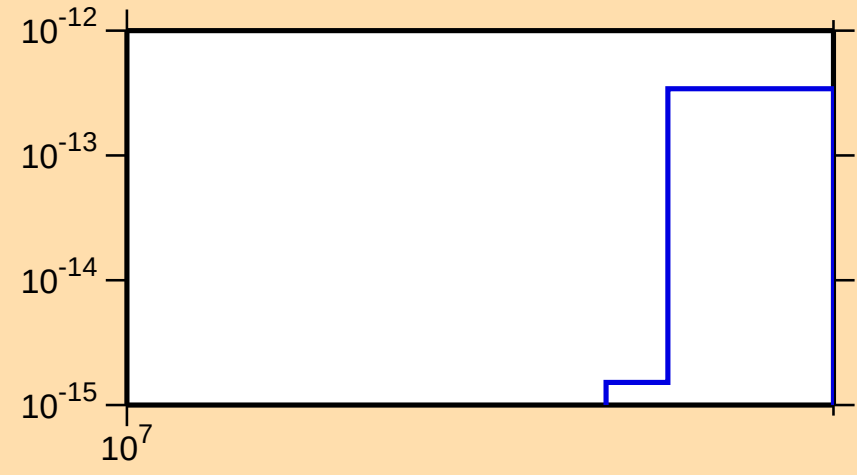
\sigma vs. E for ^{227}\text{Th} (mt 34)
