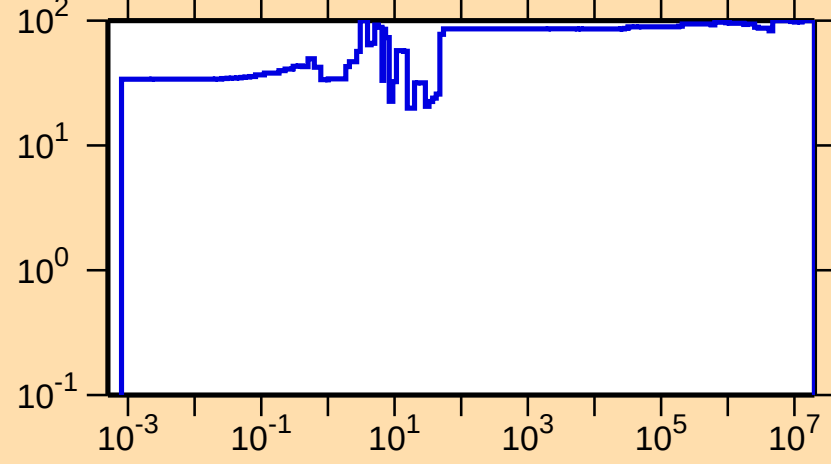
\Delta\sigma/\sigma vs. E for ^{227}\text{Th}(n,\gamma)
