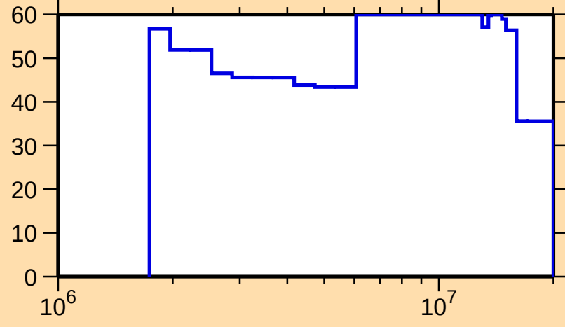
\Delta\sigma/\sigma vs. E for ^{227}\text{Th}(n,n\text{cont.})
