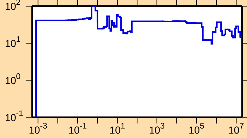
\Delta\sigma/\sigma vs. E for ^{227}\text{Th}(n,\text{el.})
