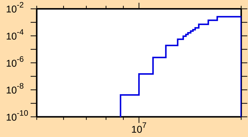
\sigma vs. E for ^{227}\text{Th}(n,d)
