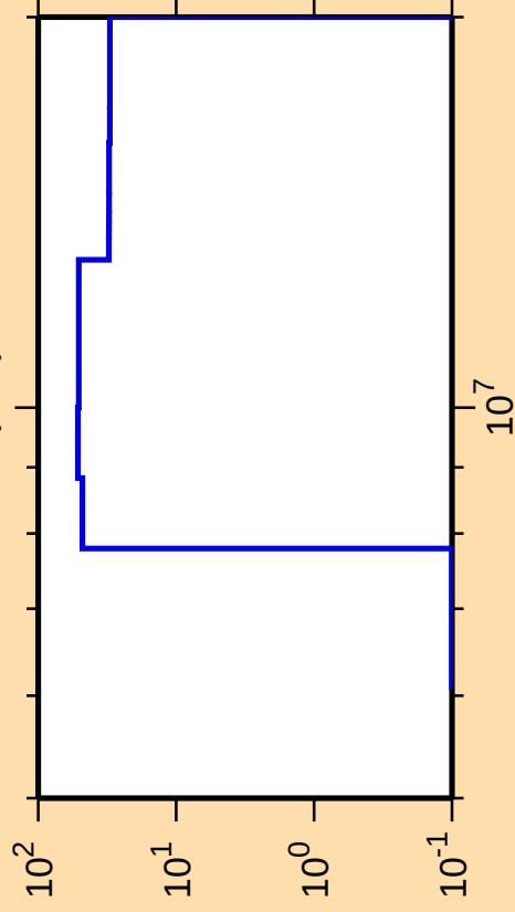
\Delta\sigma/\sigma vs. E for ^{227}\text{Th}(n,d)
