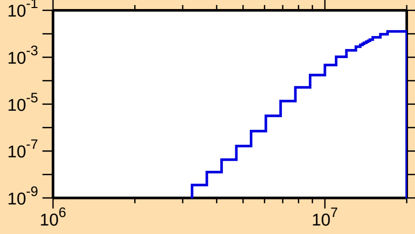
\sigma vs. E for ^{227}\text{Th}(n,p)
