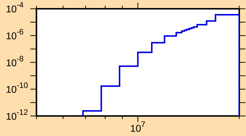
\sigma vs. E for ^{227}\text{Th}(n,2n\alpha)
