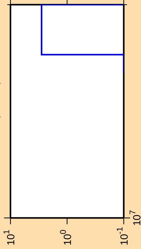
\Delta\sigma/\sigma vs. E for ^{227}\text{Th} (mt 34)
